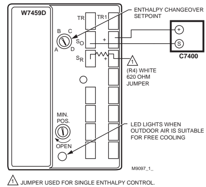
Figure 4. Control module with one enthalpy sensor
