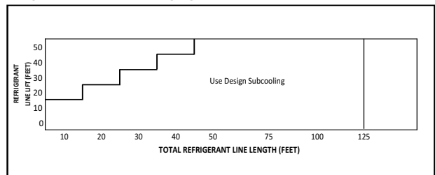
Figure 2. Subcool Charging Corrections – 042A
