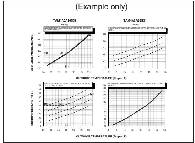
Fixed Orifice Superheat Charging Table
