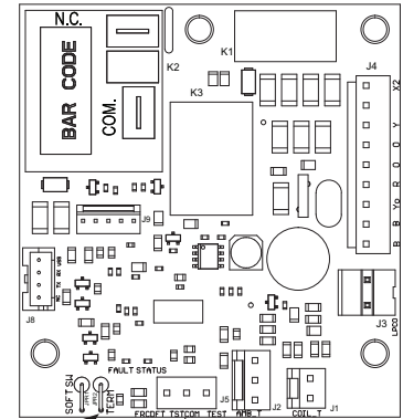
Jumper J2 J5 Test Pins
