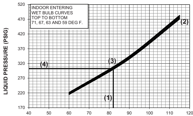
TAM9A0B30V31 Cooling @ 900 SCFM
