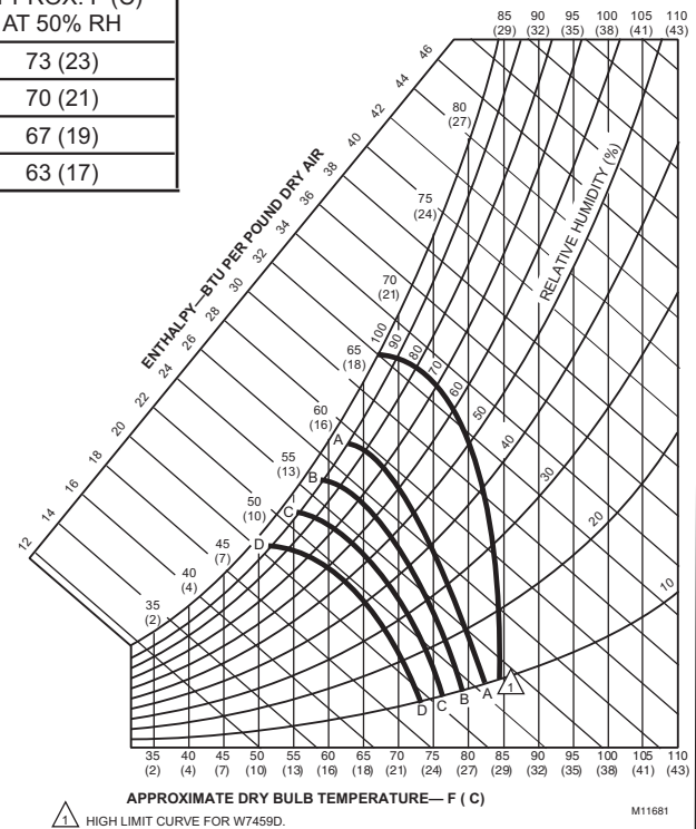
Figure 16. Single Enthalpy Changeover Set Point
