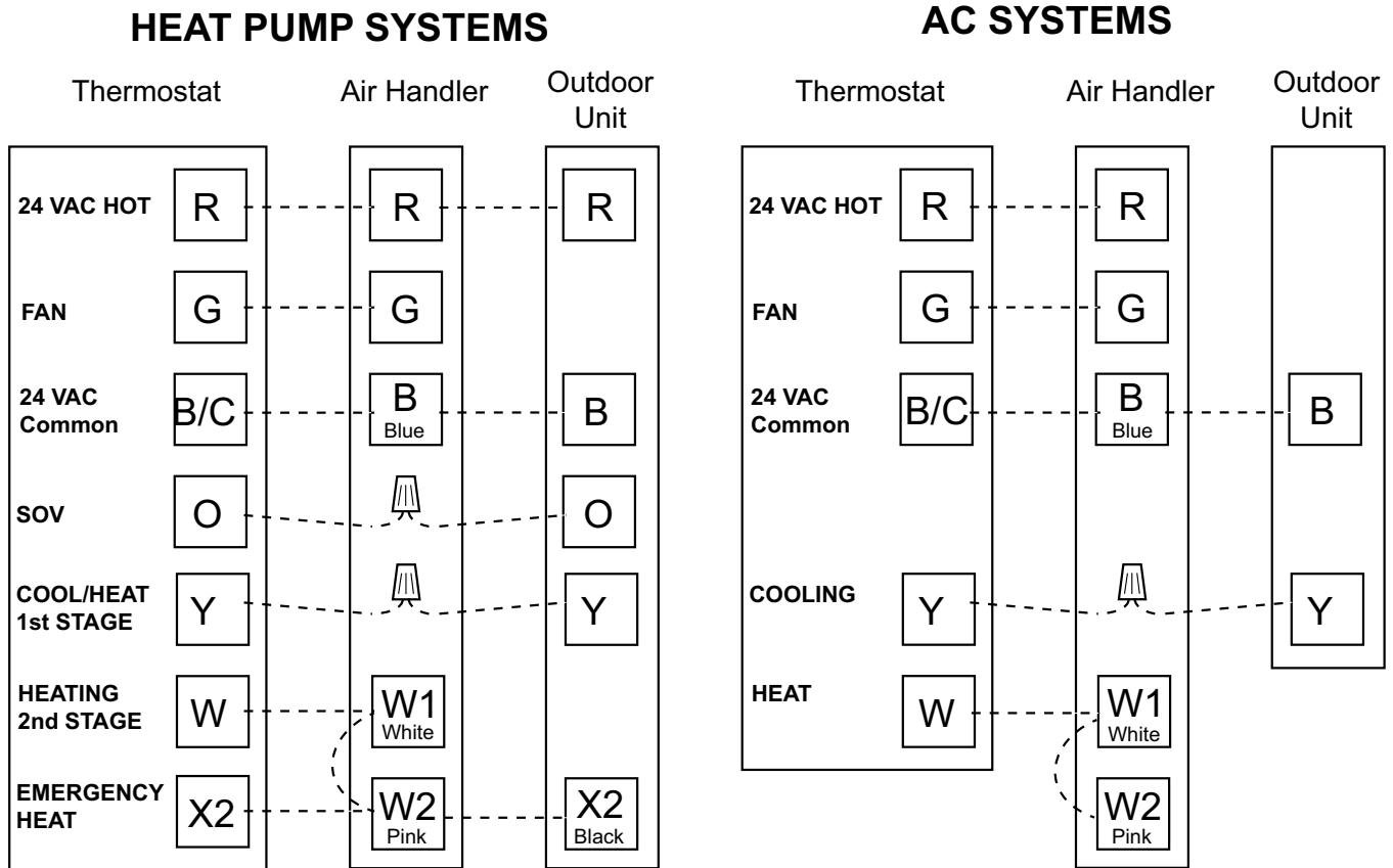
Figure 4. Field Wiring Diagram — A4AH5E*
