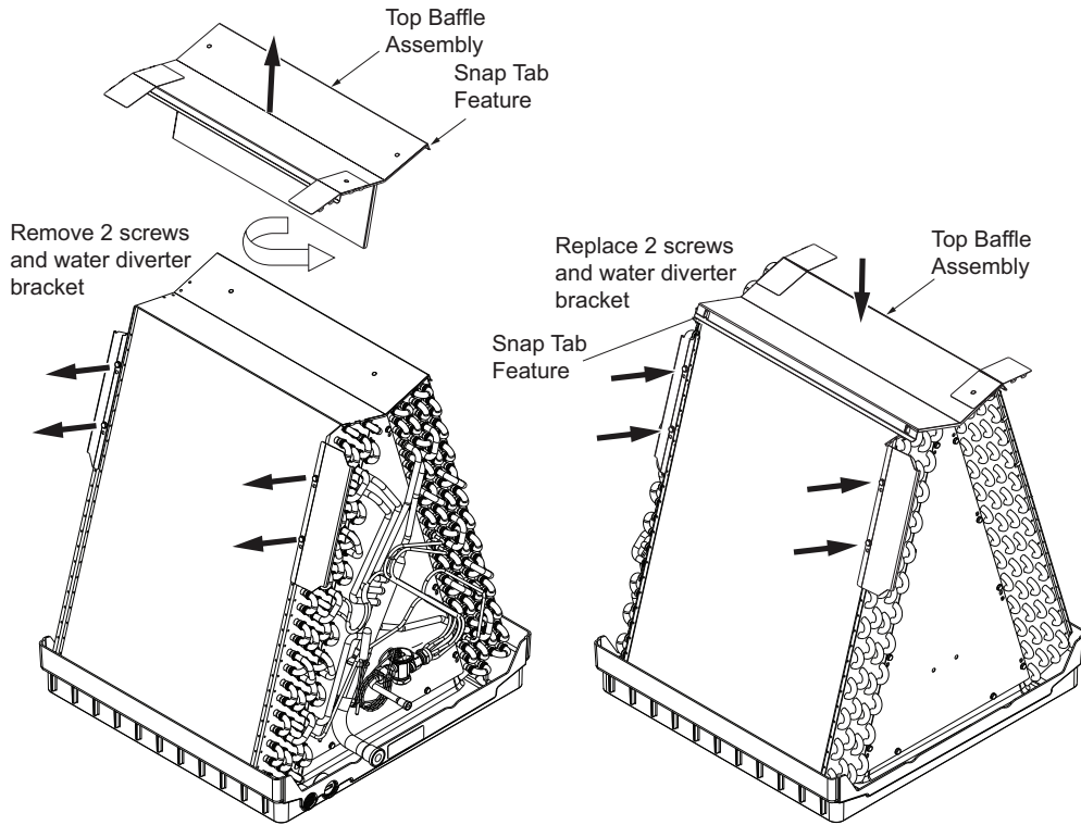
Figure 20. A4AH5E43A1C30AA, A4AH5V36A1C30AA, A4AH5V42A1C30AA
