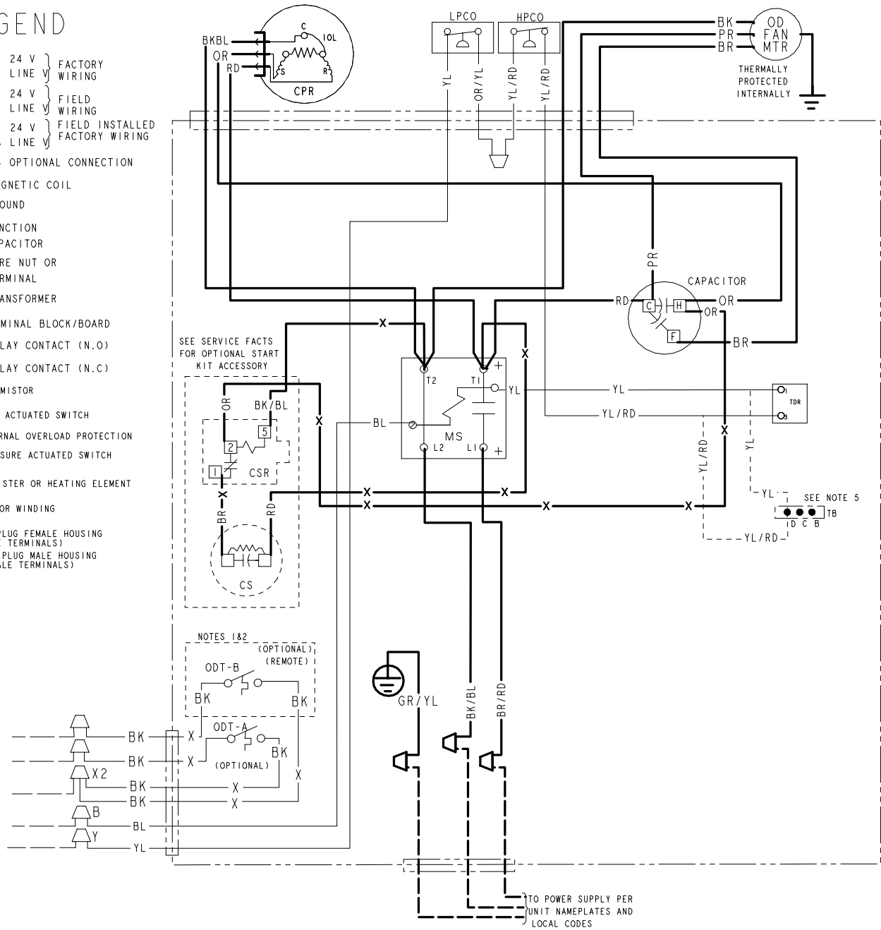
Figure 9. 1.5, 2.0, 2.5, 3.0, 3.5 and 4.0 Ton Models
