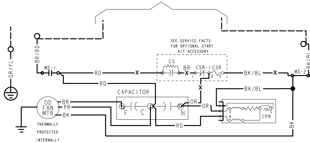
Figure 8. 1.5, 2.0, 2.5, 3.0, 3.5 and 4.0 Ton Models
