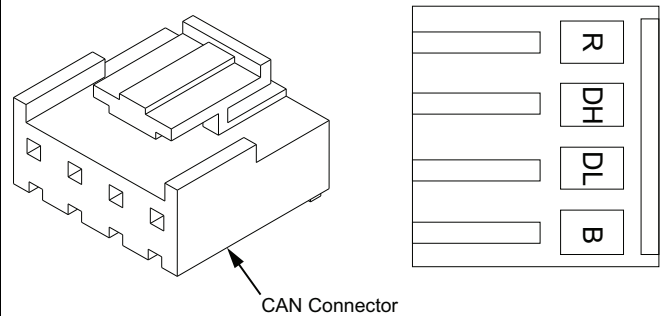
CAN Connector
