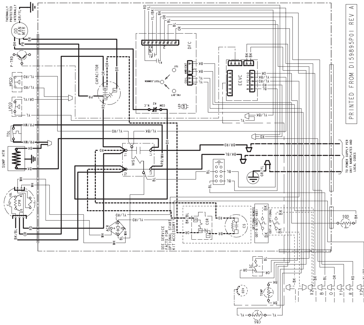
Wiring Diagram – 024E Models
