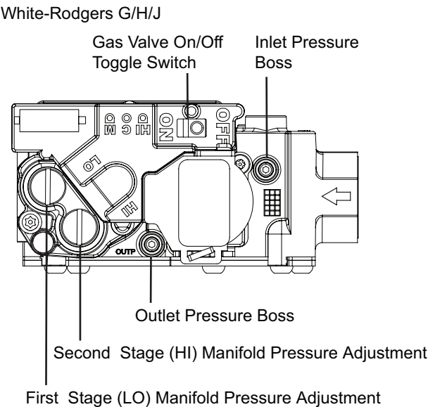
Figure 15. White-Rodgers two-stage gas valve only
