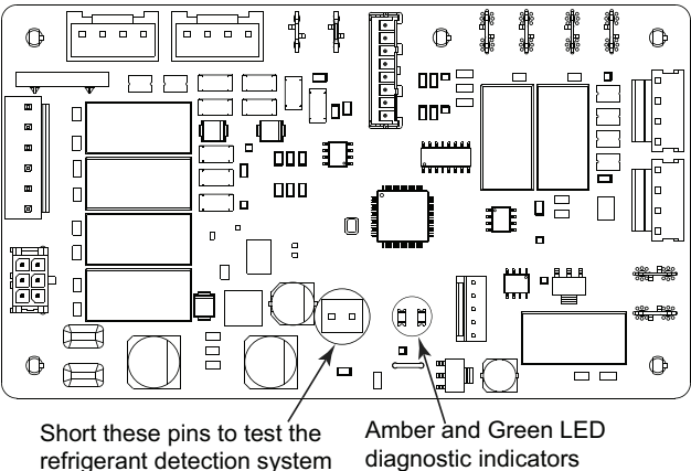
Figure 26. Mitigation control board
