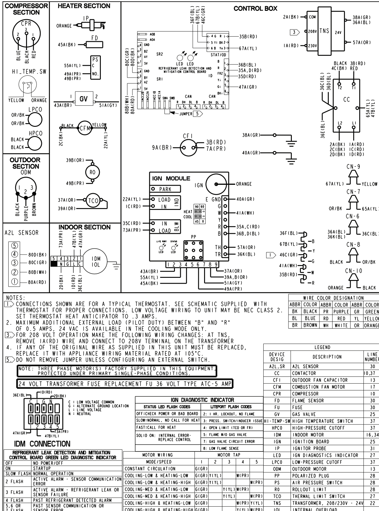
Figure 41. Models — 5YCC4036A3, 5YCC4048A3, and 5YCC4060A3
