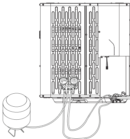
Figure 33. Charging the unit
