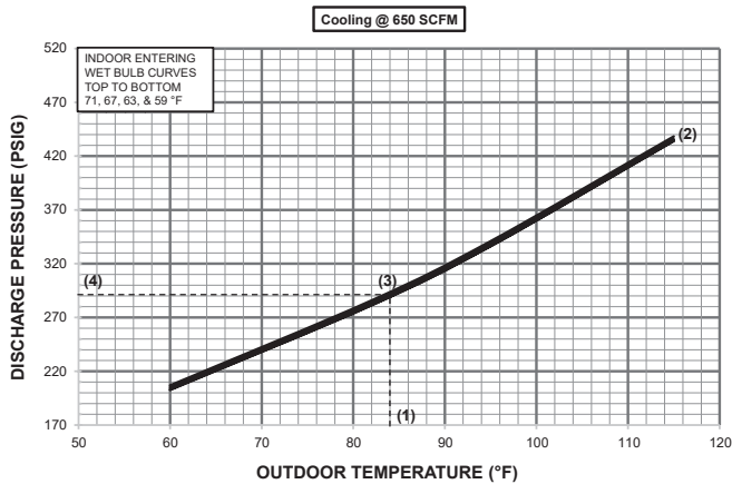
Figure 42. Pressure curves – model A5HP4018A1
