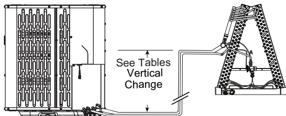
Figure 4. Refrigerant piping vertical change limit
