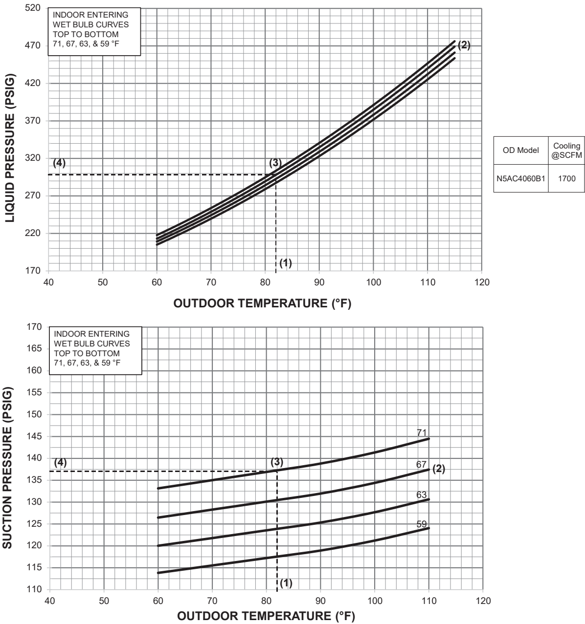
Figure 38. Model N5AC4060B1
