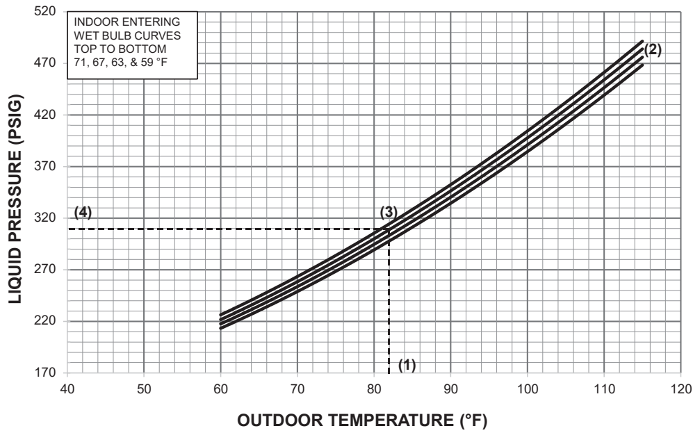
Figure 37. Models N5AC4036B1 and N5AC4048B1
