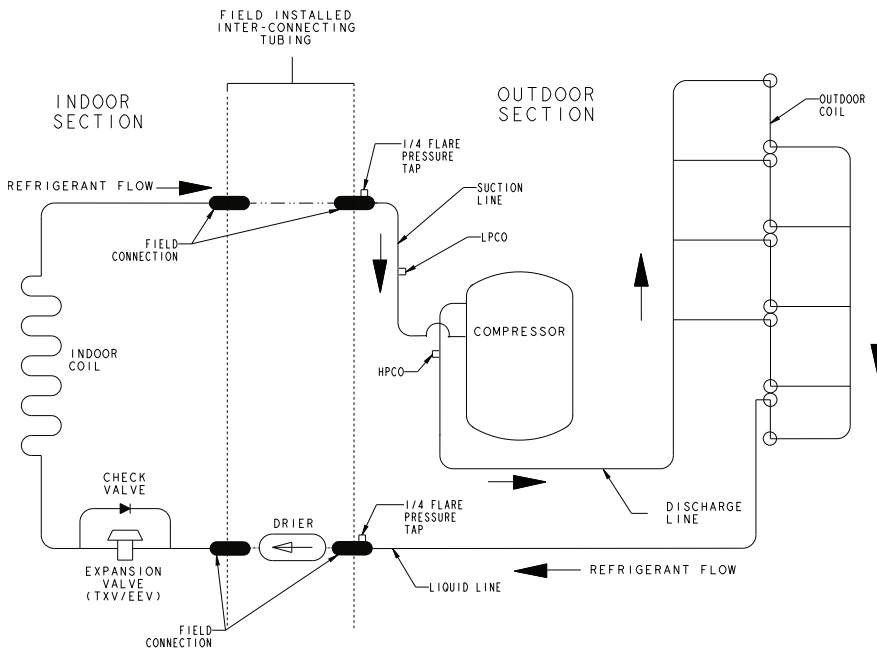
Figure 40. Model - 060
