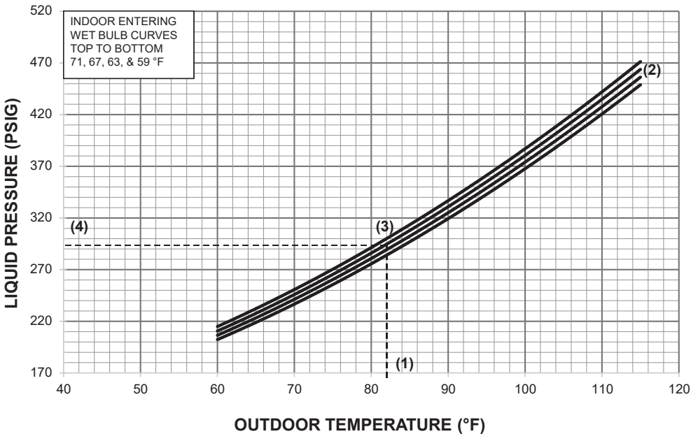
Figure 35. Model N5AC4018B1
