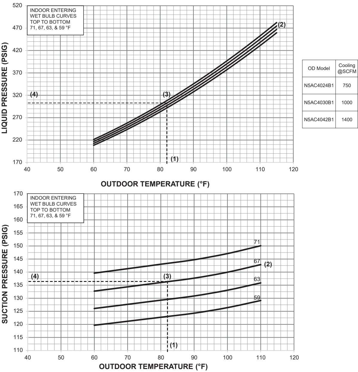
Figure 36. Models N5AC4024B1, N5AC4030B1, and N5AC4042B1
