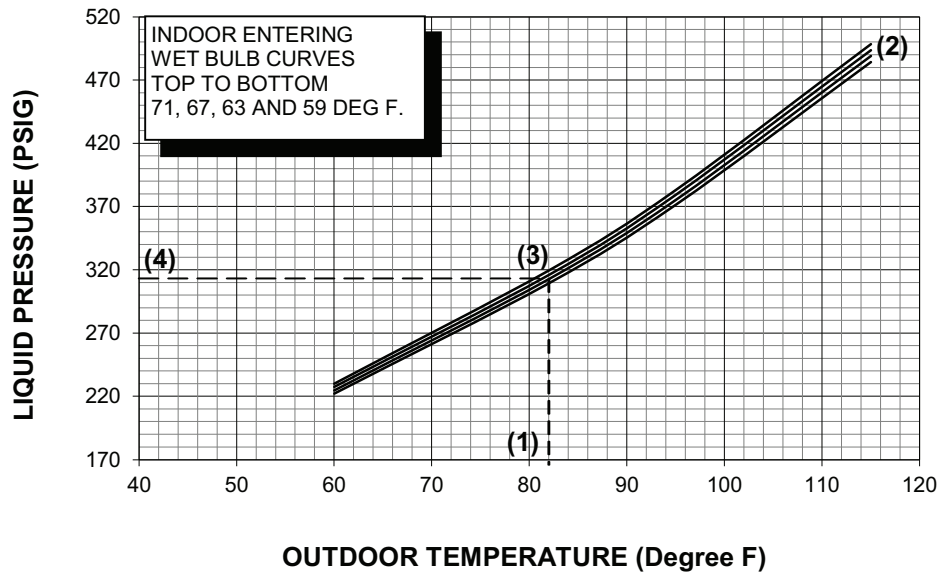
Figure 40. Pressure curves - model 5TTR6060A1
