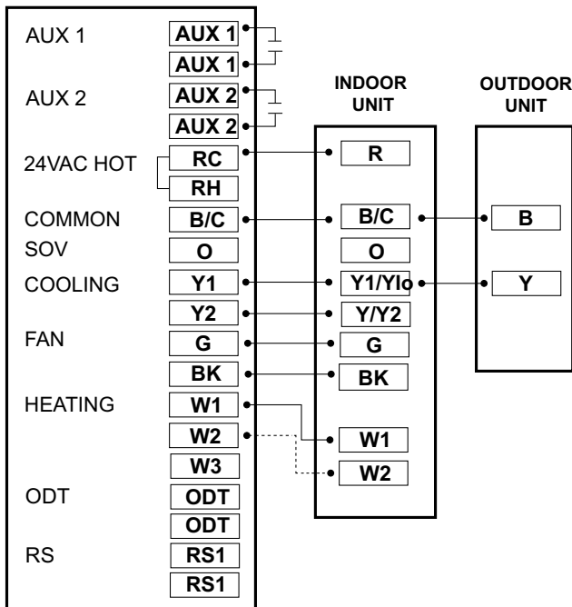
Figure 25. 2-stage AC thermostat
