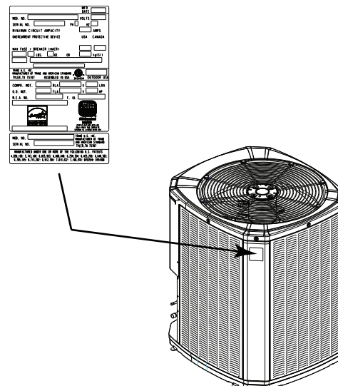
Figure 26. Nameplate location
