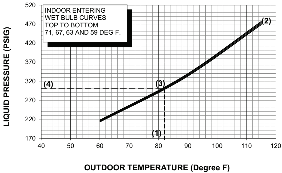
Figure 39. Pressure curves - models 5TTR6024A1, 5TTR6030A1, 5TTR6036A1, 5TTR6042A1, and 5TTR6048A1
