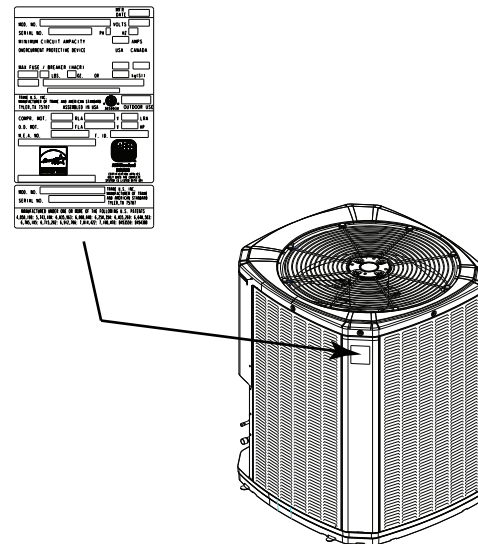
Figure 26. Nameplate location
