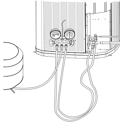
Figure 33. Charging the unit
