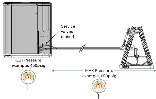
Figure 17. Refrigerant line leak check
