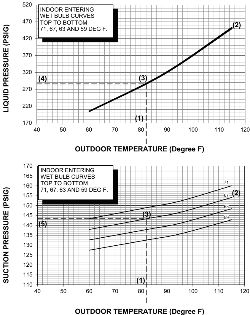
Figure 37. Pressure curves - model 5TTR4018A1
