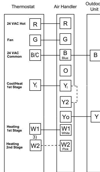
Figure 22. Single stage, AC, 5TEM4
