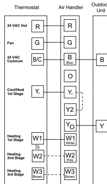
Figure 23. Single stage, AC, 5TEM5
