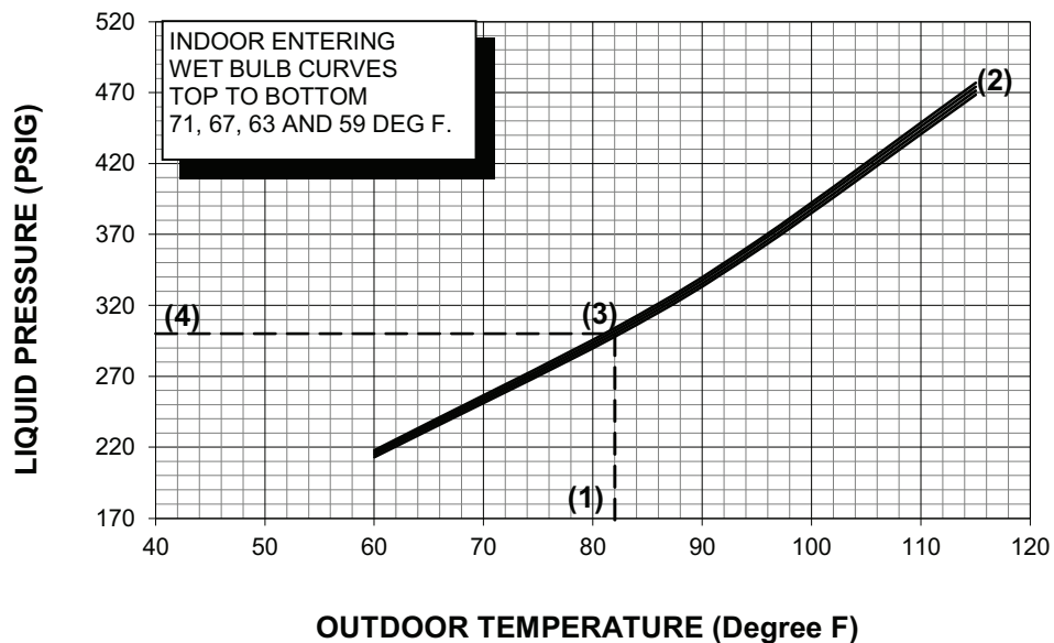
Figure 38. Pressure curves - models 5TTR4024A1, 5TTR4030A1, 5TTR4036A1, 5TTR4042A1, and 5TTR4048A1
