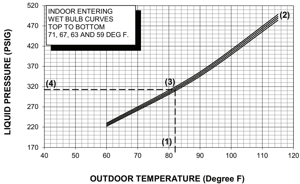
Figure 39. Pressure curves - model 5TTR4060A1
