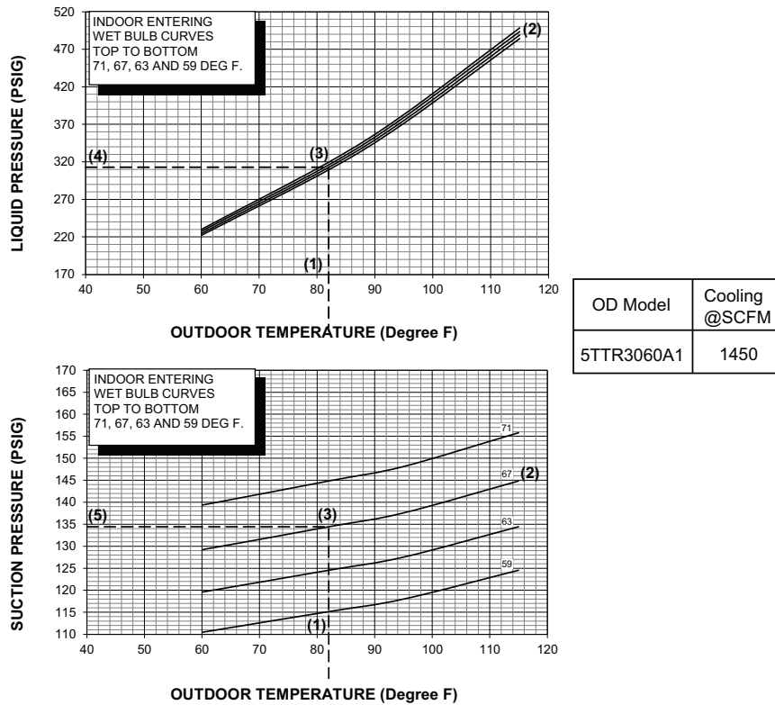
Figure 42. Pressure curves - Model 5TTR3060A1
