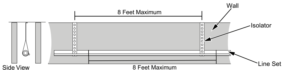
Figure 10. Isolation in wall spaces
