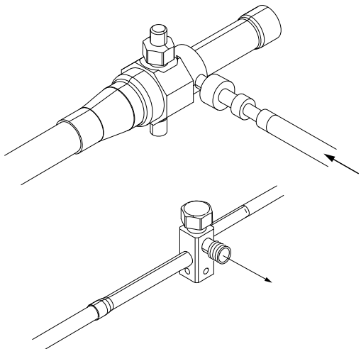
Figure 15. Purging of refrigerant lines
