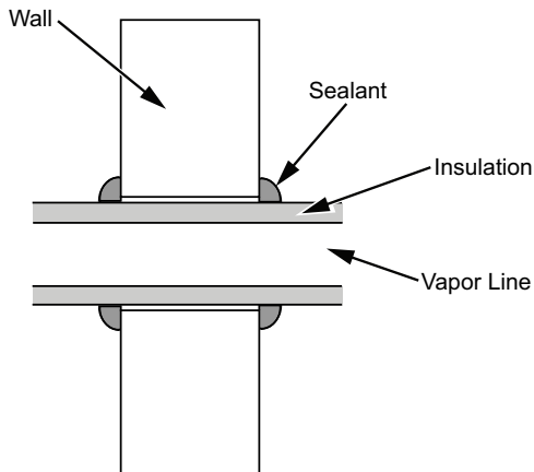
Figure 12. Incorrect lineset installation
