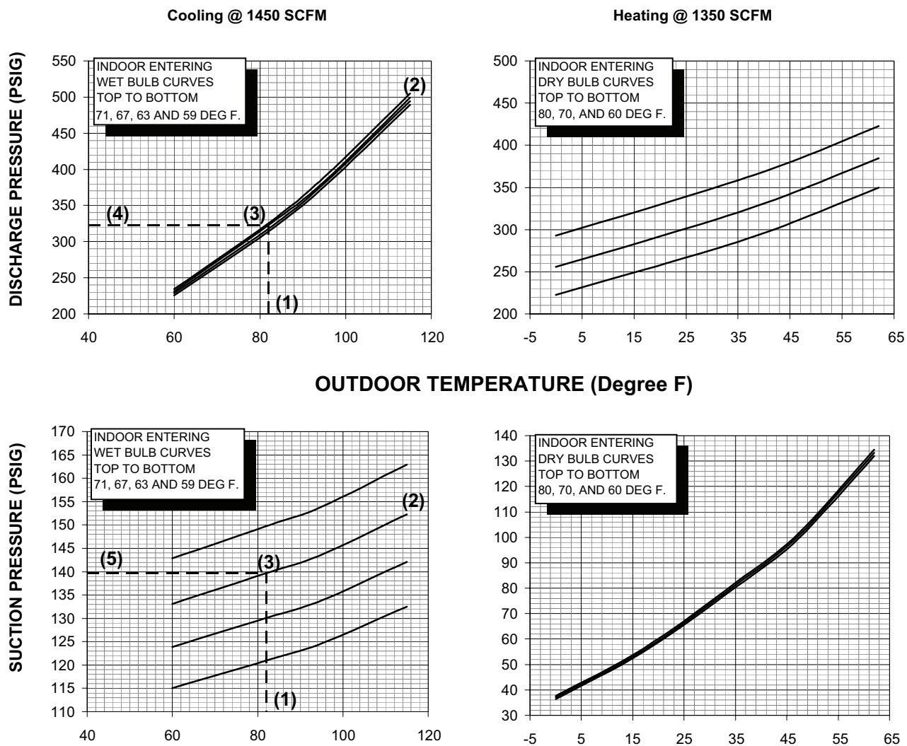
Figure 36. Pressure curve sample
