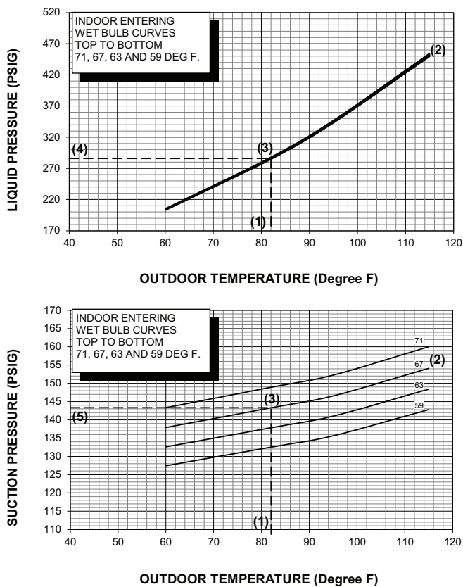
Figure 40. Pressure curves - model 5TTR3018A1
