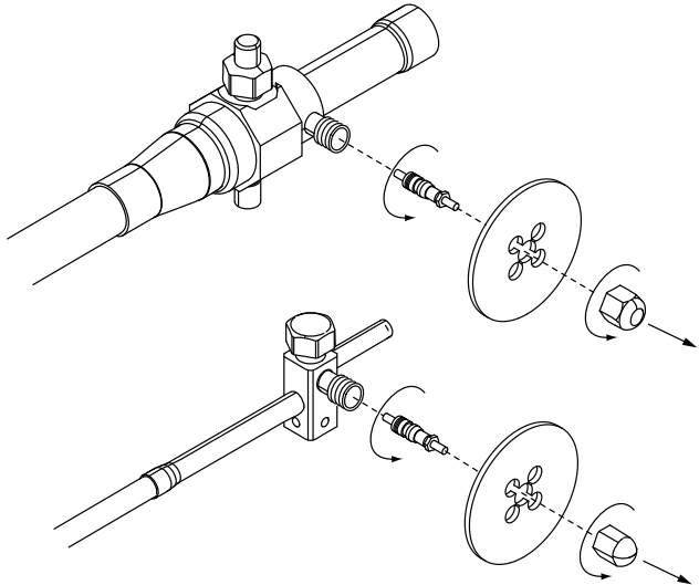
Figure 15. Purging of refrigerant lines
