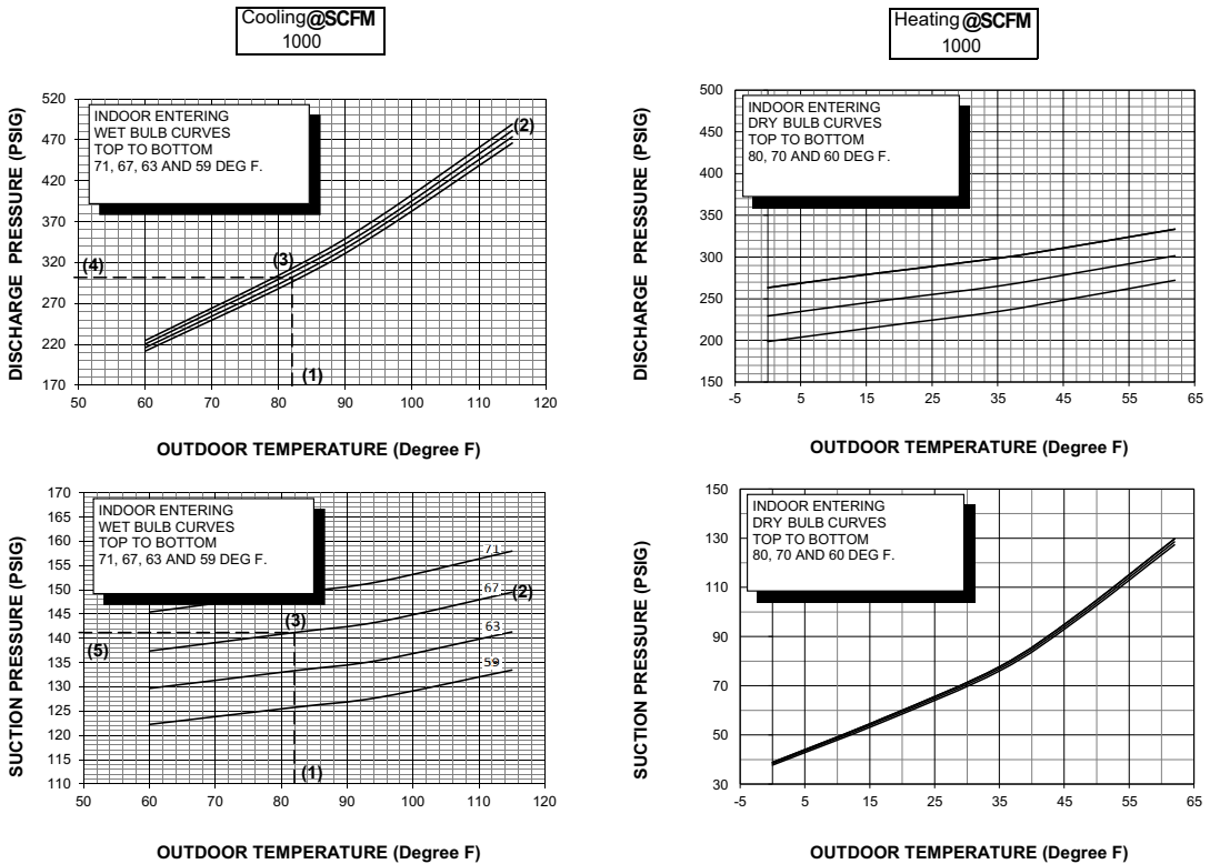
Figure 50. Pressure curves - model 5TWR5030A1
