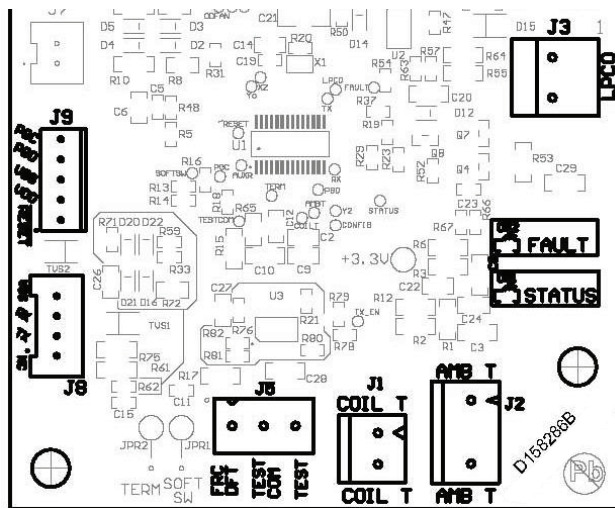
Figure 44. Defrost board detail
