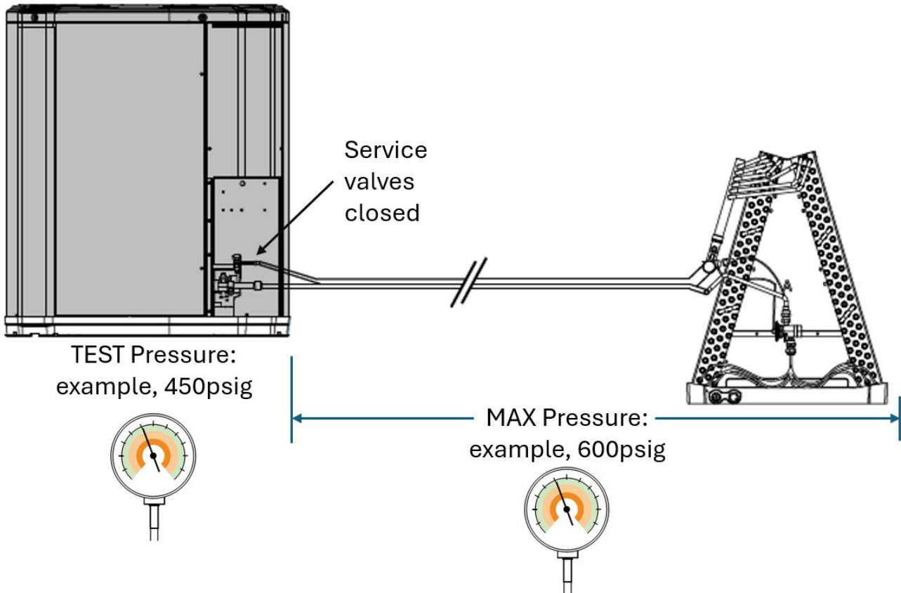
Figure 16. Pressure check
