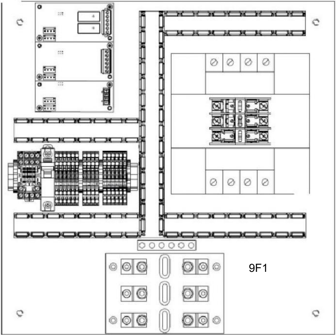
CONTROL PANEL DETAIL
