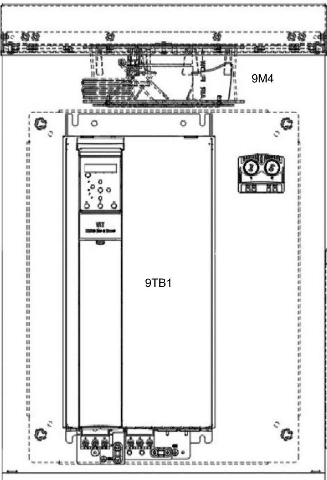
VFD PANEL DETAIL
