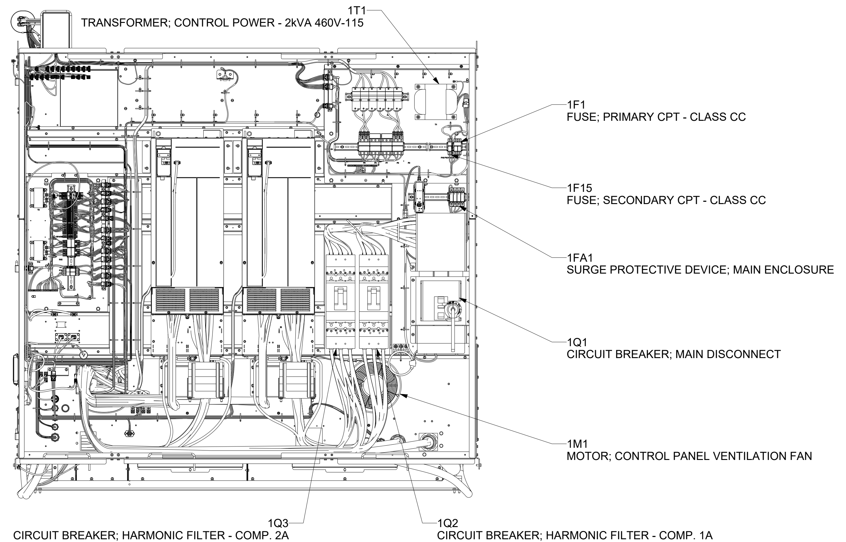
CONTROL PANEL, FRONT VIEW HARMONIC FILTERS SHOWN WITH LOW VOLTAGE AND PANEL DOORS AND MULLION HIDDEN
