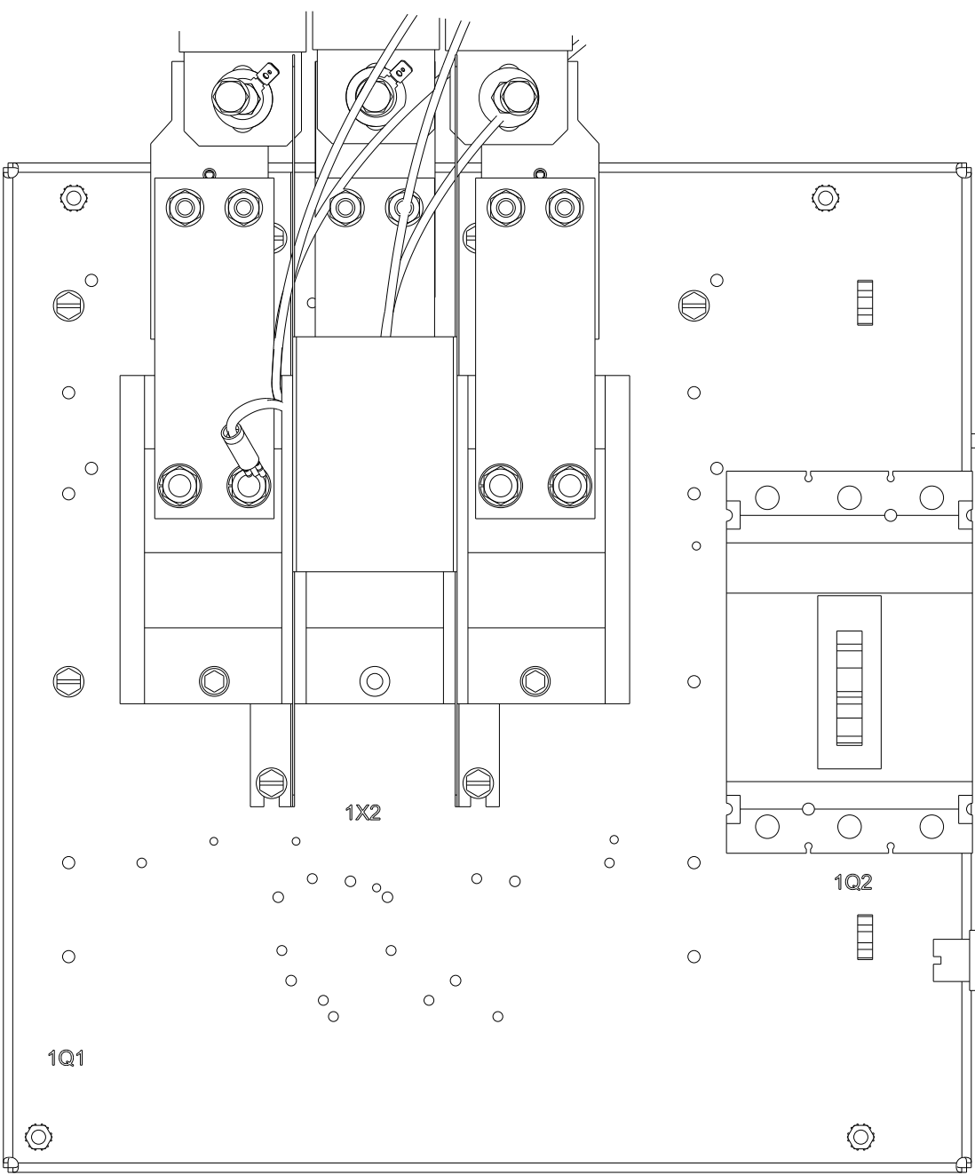
DETAIL C TERMINAL BLOCK OPTION
