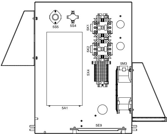
VSD PUMP ENCLOSURE - SMALL FACTORY PUMP ONLY OPTION FOR S & V UNITS
