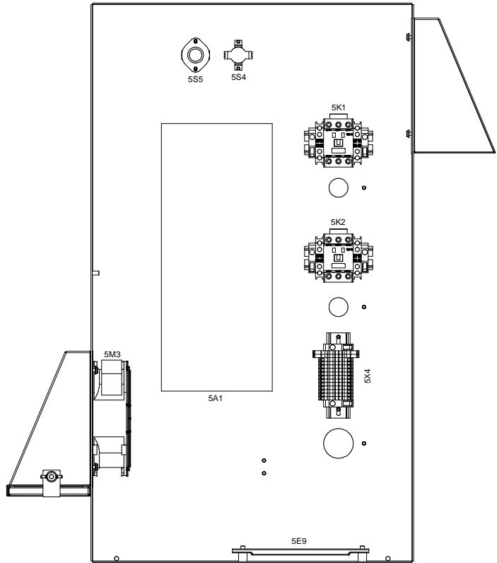
VSD PUMP ENCLOSURE - LARGE FACTORY PUMP ONLY OPTION FOR W UNITS
