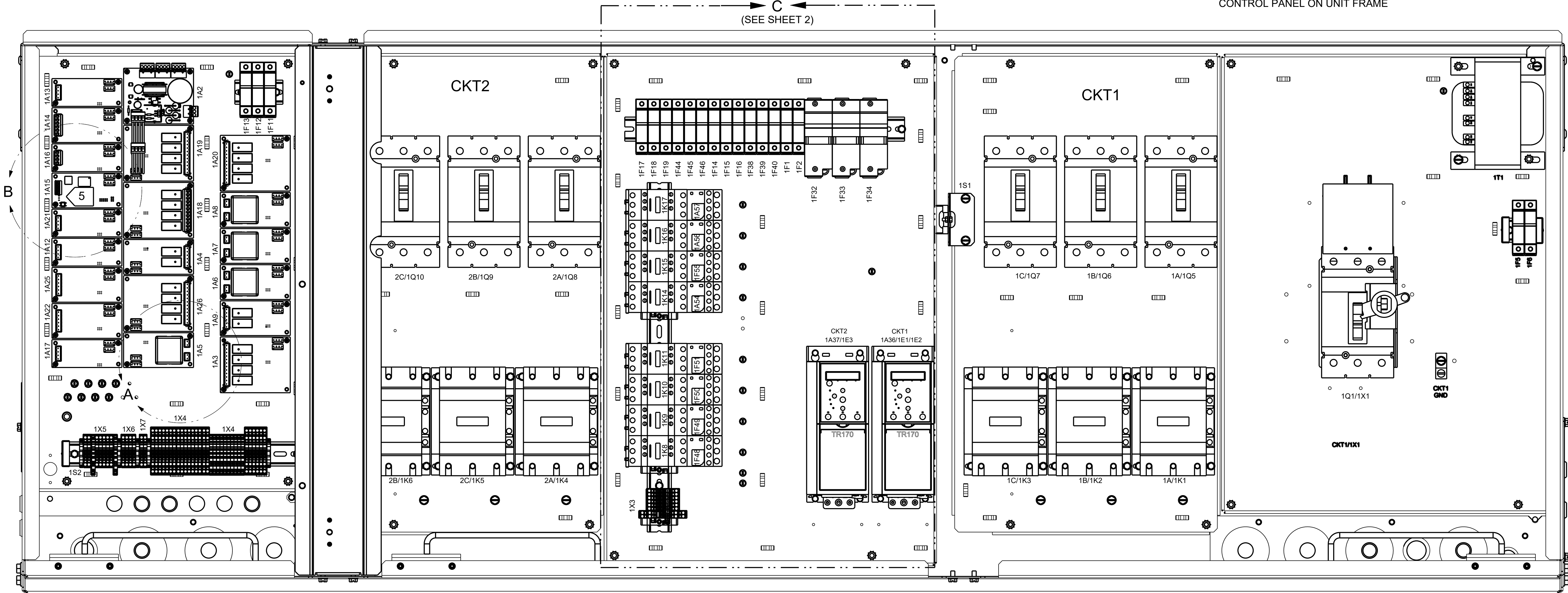
DETAIL B 6 (1A41 BACnet MODULE SHOWN 1A15 LCI MODULE REMOVED)
