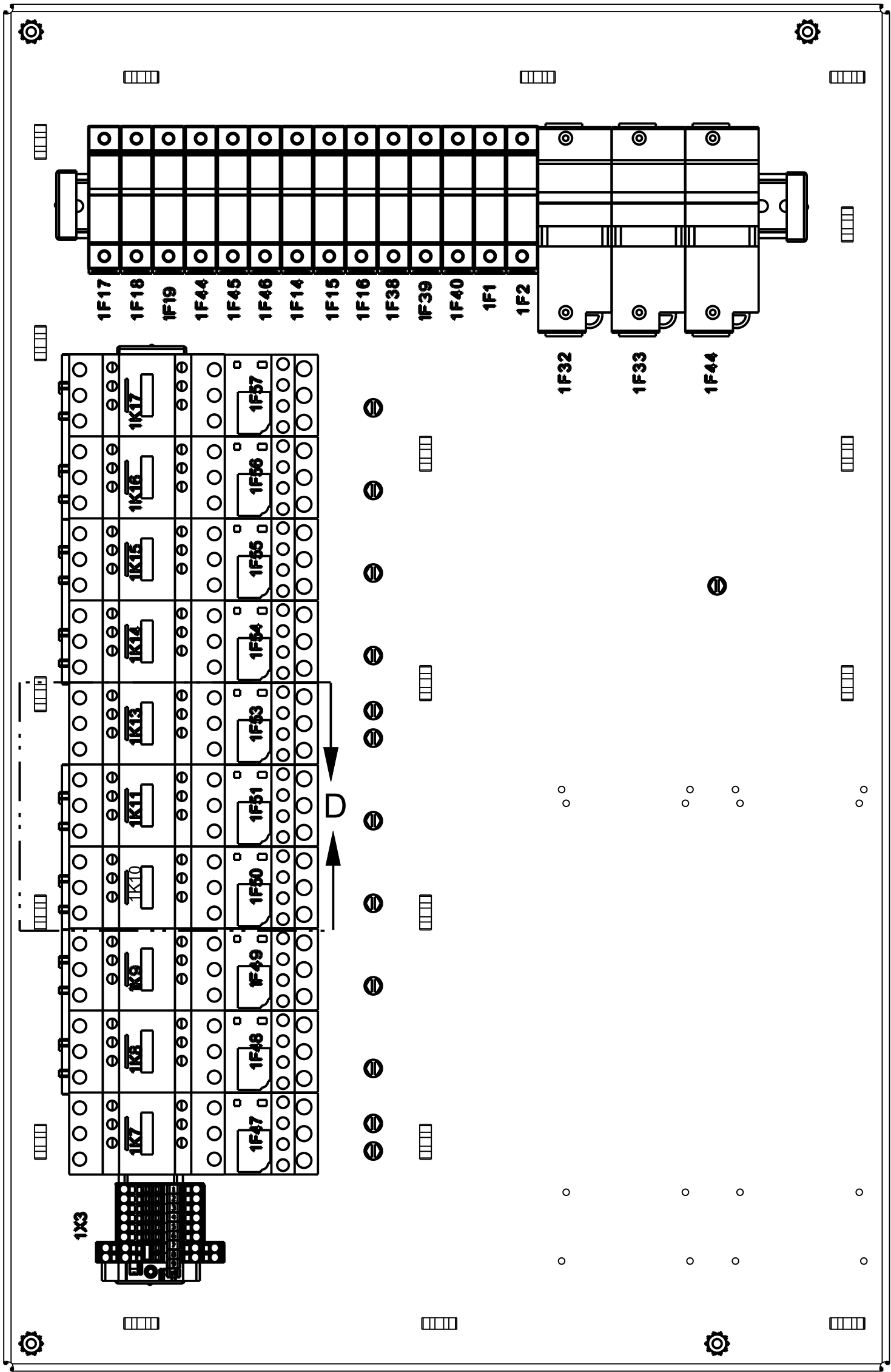
DETAIL C WO VFD 1SP, 4 OR 5 FANS/CKT
