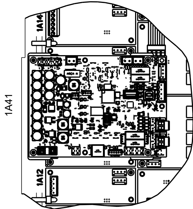
DETAIL B 6 (1A41 BACnet MODULE SHOWN 1A15 LCI MODULE REMOVED)
