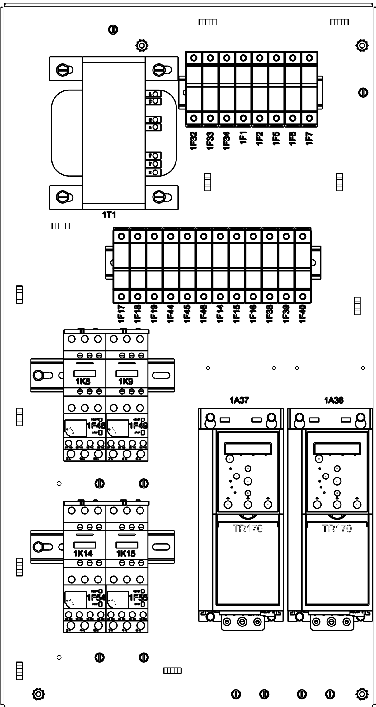
DETAIL C WITH VFD
