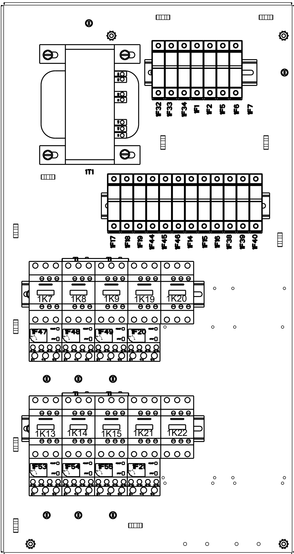
DETAIL C 2SP FAN, WO VFD
