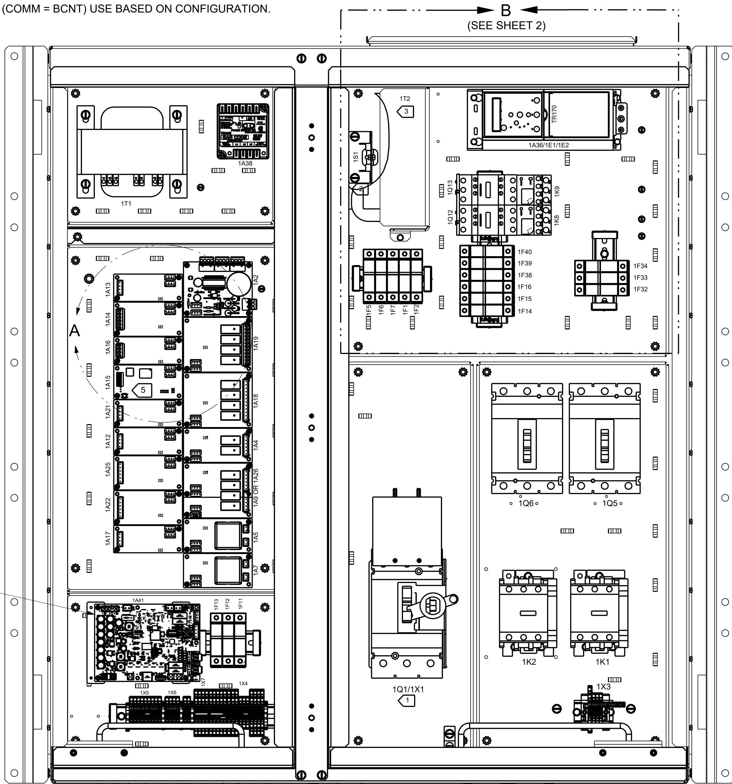
DOORS SHOWN OFF (WITH VENTILATED PANEL)
