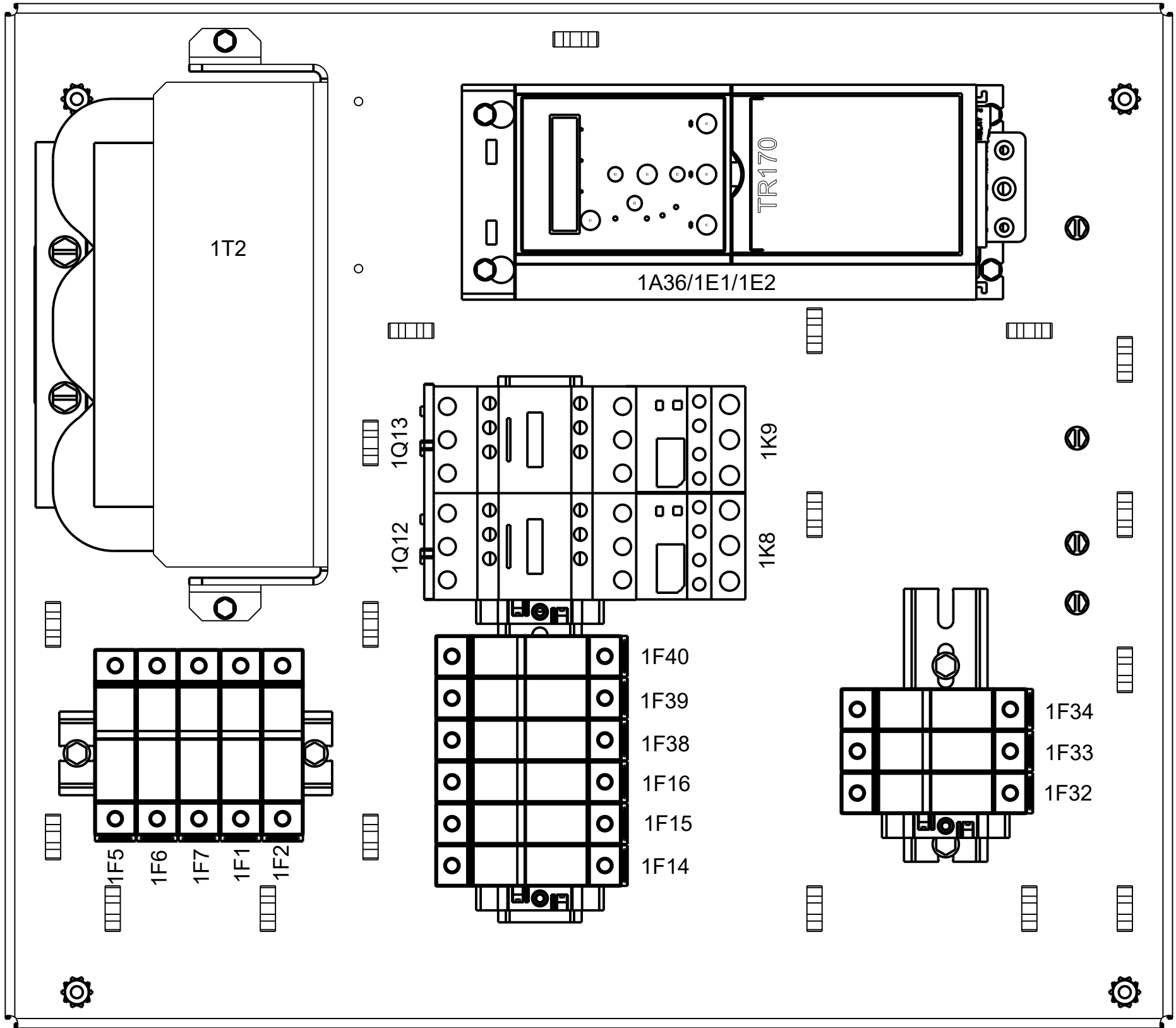
DETAIL B 3 FAN, W VFD
