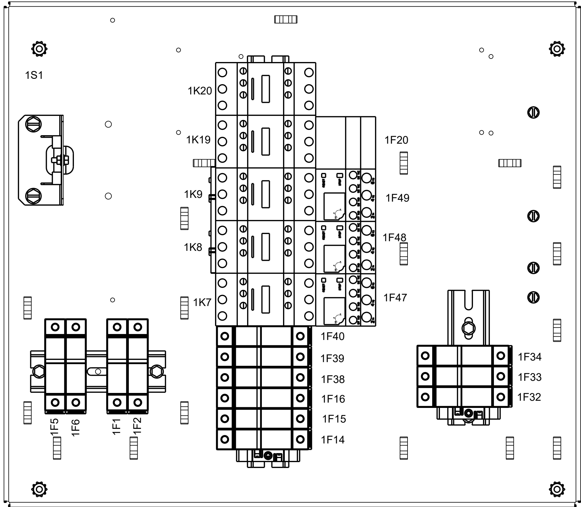
DETAIL B 3 FAN,WO VFD
