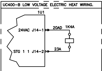
SINGLE STAGE LOW VOLTAGE ONE ELEMENT ELECTRIC HEAT WIRING
