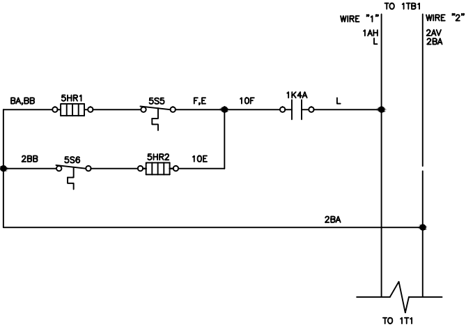
TWO ELEMENT HIGH VOLTAGE ELECTRIC HEAT WIRING
