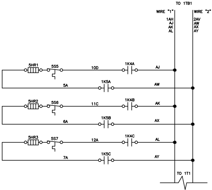
HIGH VOLTAGE ELECTRIC HEAT WIRING
