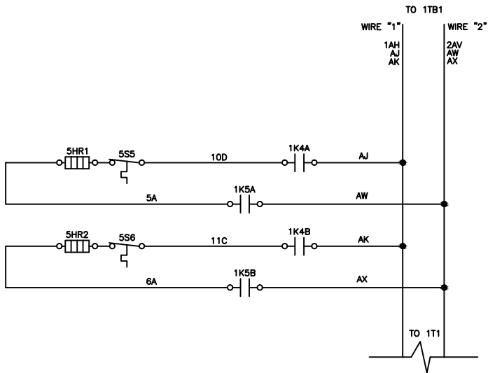
HIGH VOLTAGE ELECTRIC HEAT WIRING
