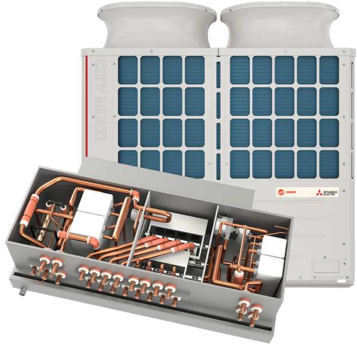
Figure 3. The hybrid branch controller exchanges heat between refrigerant and water in order to reduce the use of refrigerant in VRF systems.
