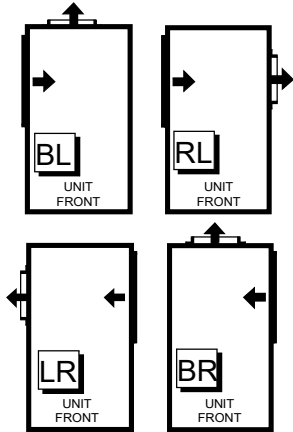
Figure 15. Horizontal Supply/Return Air Configuration
