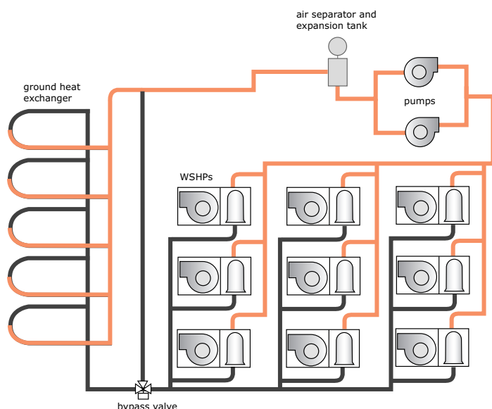
Figure 11. Ground source heat pump system
