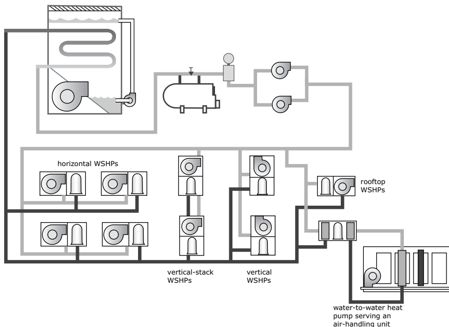
Figure 10. Conventional water-source heat pump system
