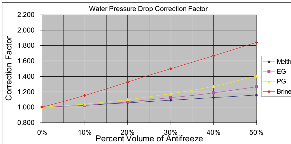
Figure 19. Water pressure drop correction factor
