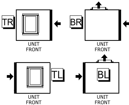
Figure 16. Vertical Supply/Return Air Configuration
