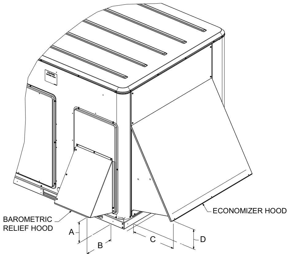
Figure 35. 3 to 10 ton cabinet – standard economizer, manual or motorized fresh air damper
