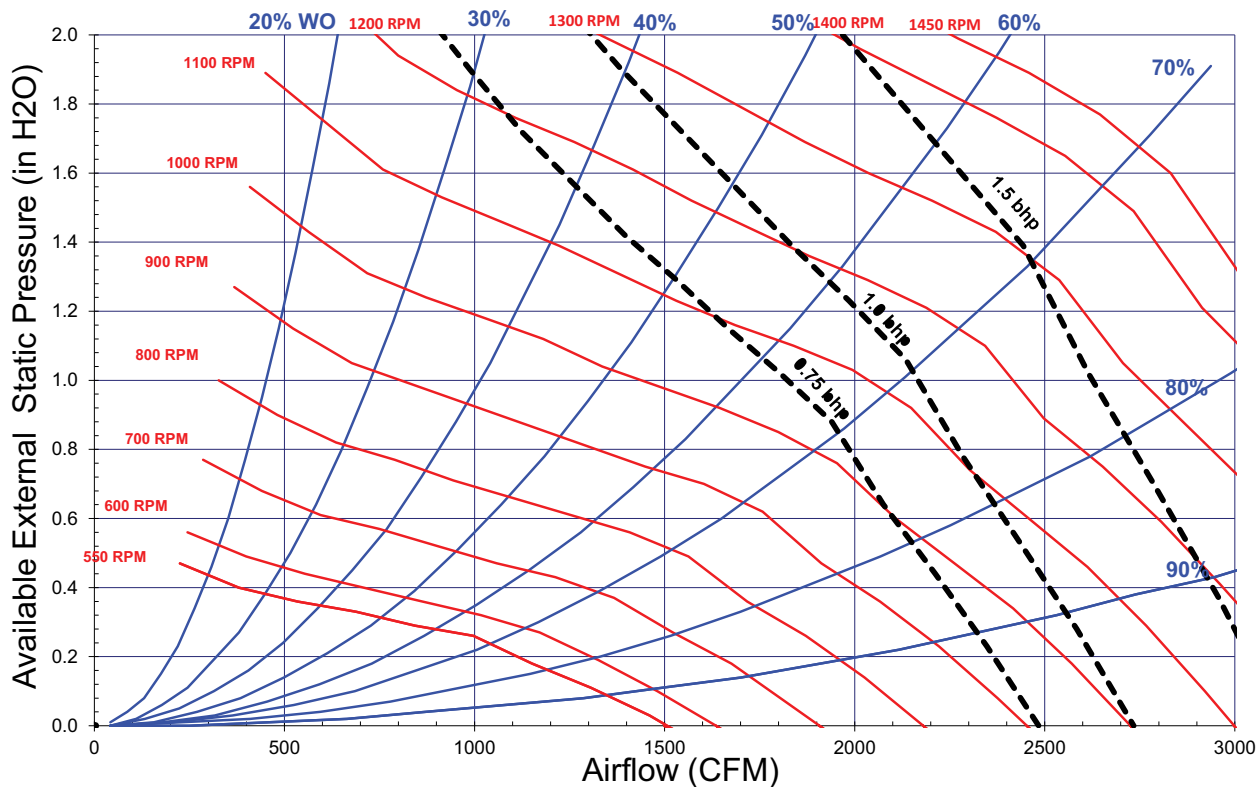
Figure 9. Fan curves – 3 to 5 tons (model GSK), horizontal
