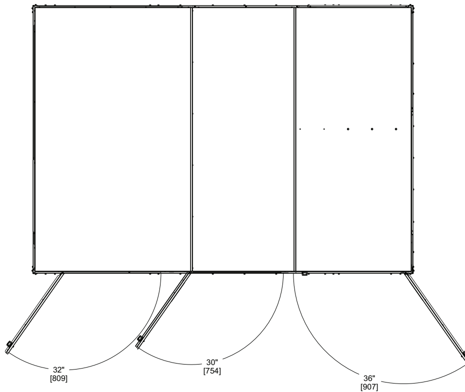
Figure 44. 12.5 to 25 ton cabinets – swing diameter for hinged door(s) option
