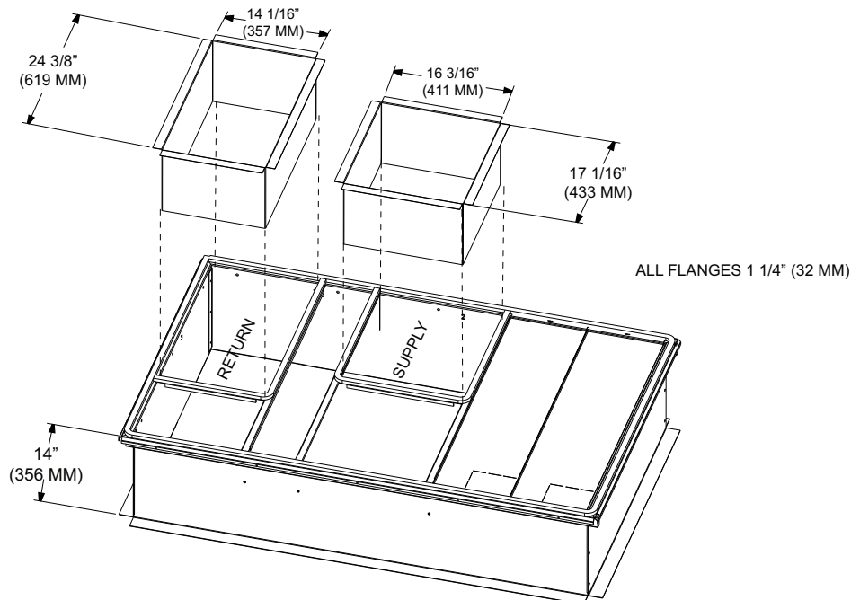
Figure 25. 3 to 5 ton cabinet – downflow duct connections, field fabricated
