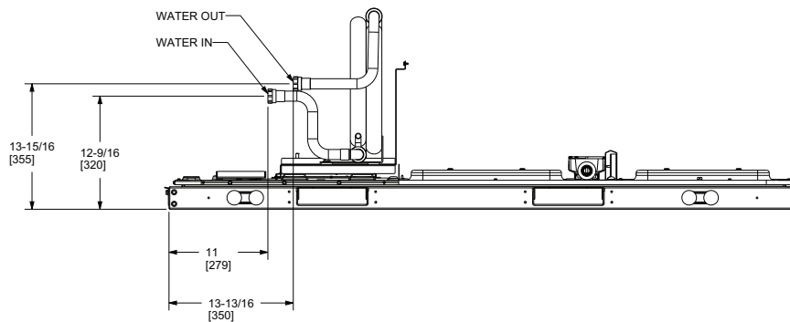
Figure 23. 3 to 5 ton cabinet – unit clearance and roof opening
