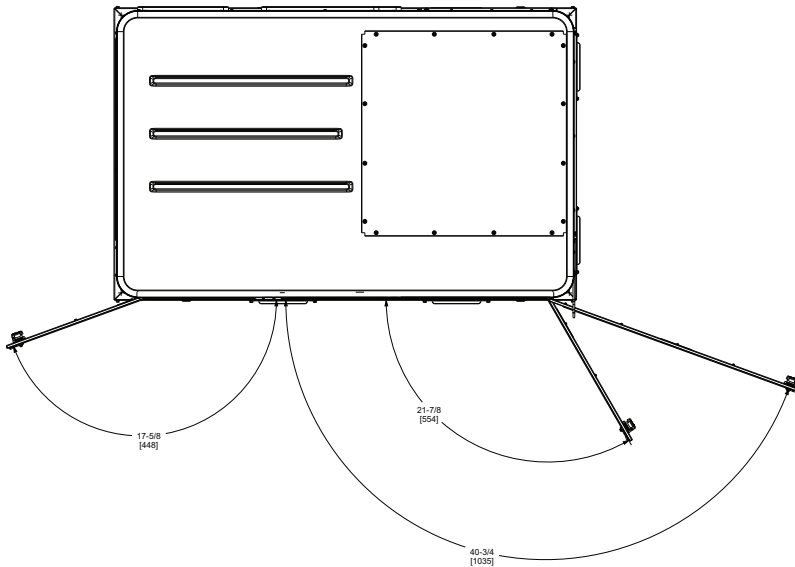
Figure 27. 6 to 10 ton cabinet
