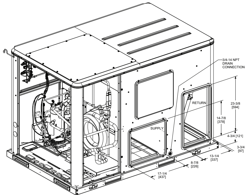
Figure 22. 3 to 5 ton cabinet - coaxial coil connections
