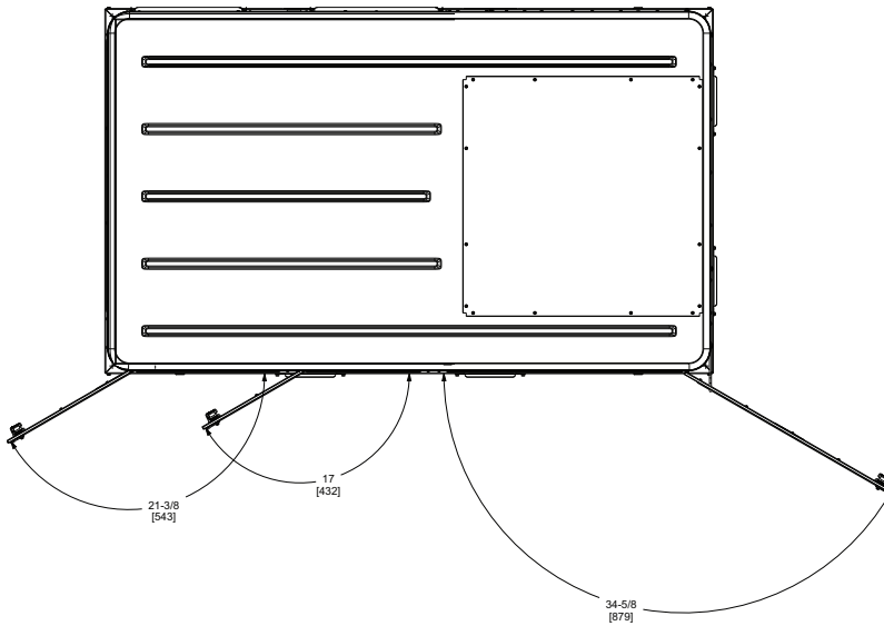
Figure 35. 3 to 10 ton cabinet – standard economizer, manual or motorized fresh air damper
