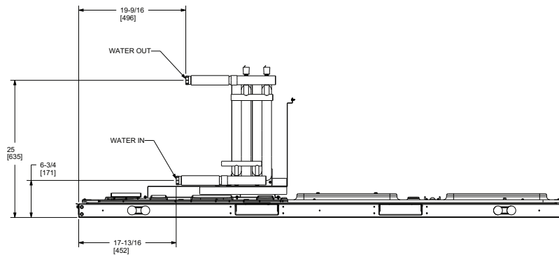
Figure 31. 6 to 10 ton cabinet – unit clearance and roof opening
