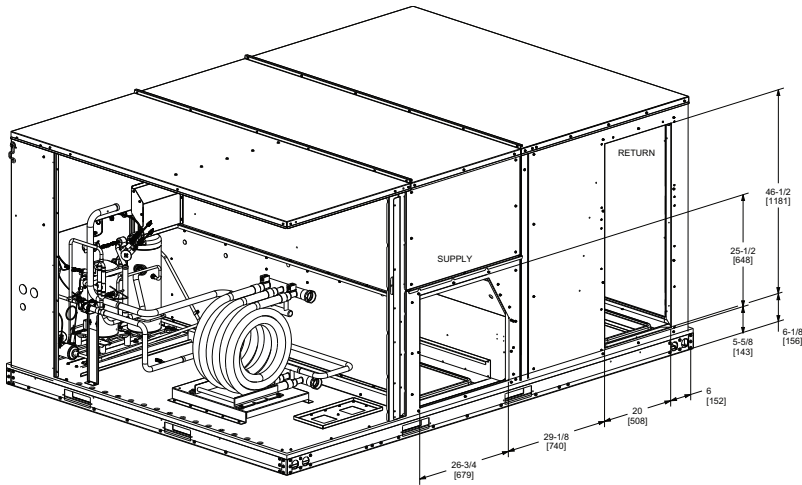
Figure 41. 12.5 to 25 ton cabinet - coaxial coil connections
