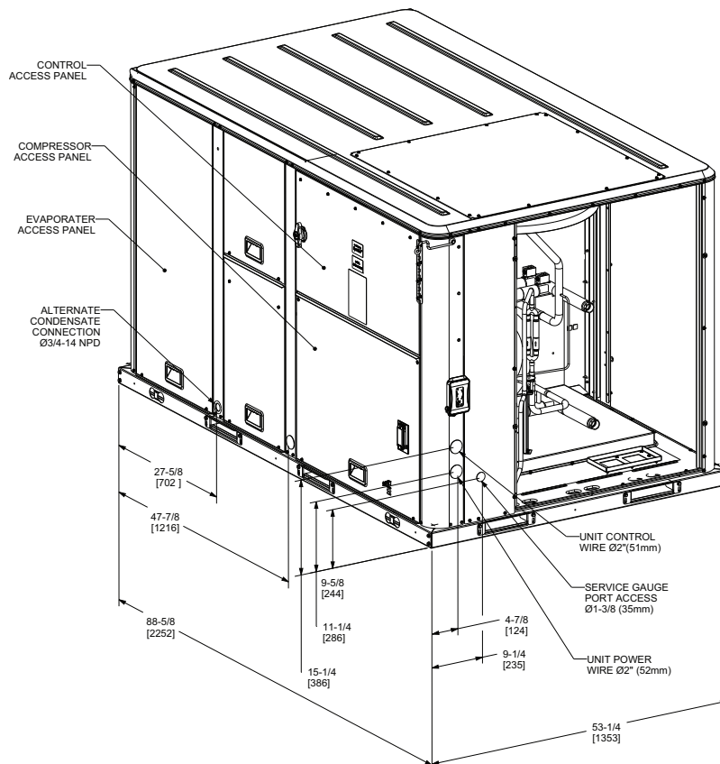
Figure 27. 6 to 10 ton cabinet
