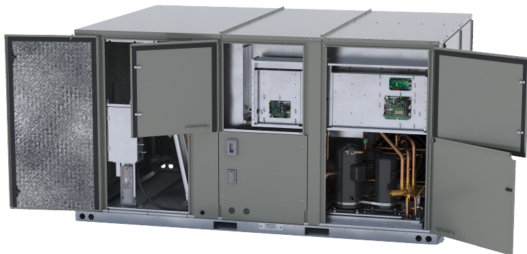
Figure 5. Hinged access doors
