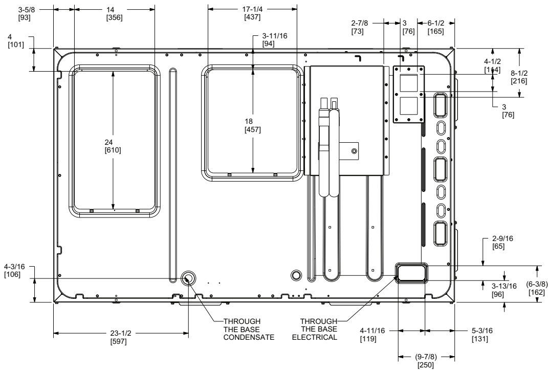
Figure 20. 3 to 5 ton cabinet – downflow airflow supply/return, through-the-base utilities
