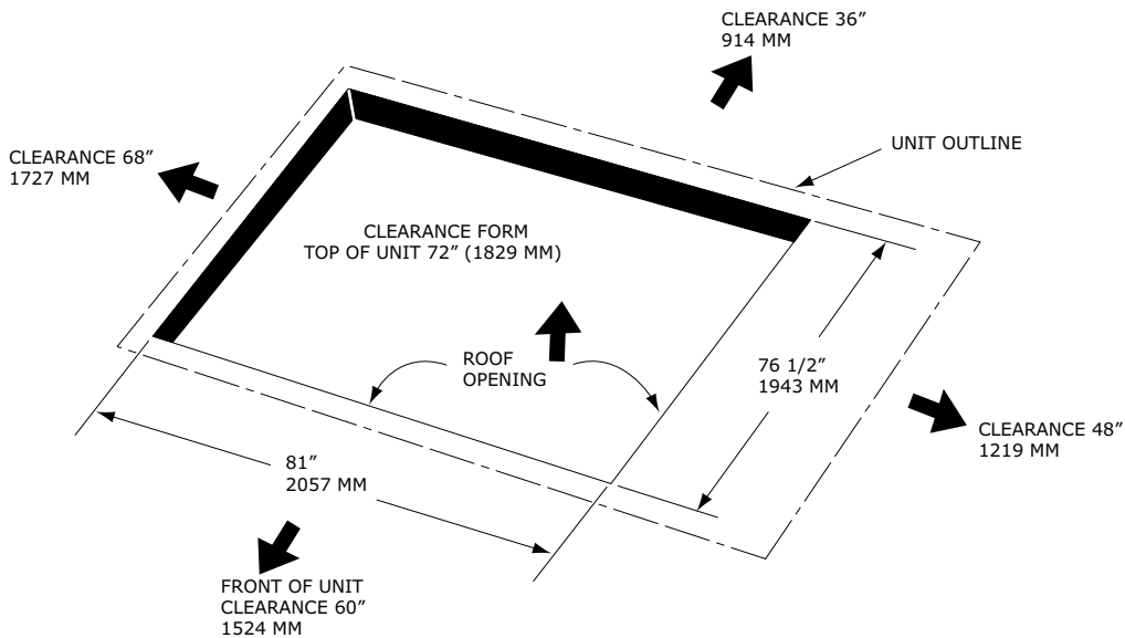
Figure 42. 12.5 to 25 ton cabinets – unit clearance and roof opening
