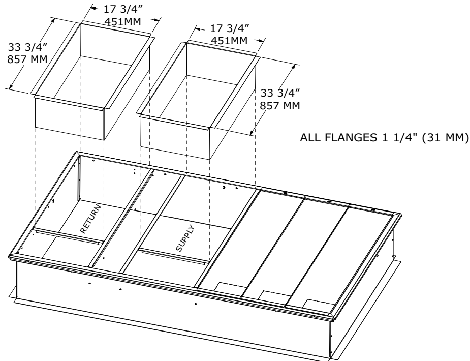
Figure 33. 6 to 10 ton cabinet – downflow duct connections, field fabricated
