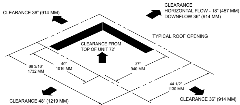
Figure 23. 3 to 5 ton cabinet – unit clearance and roof opening
