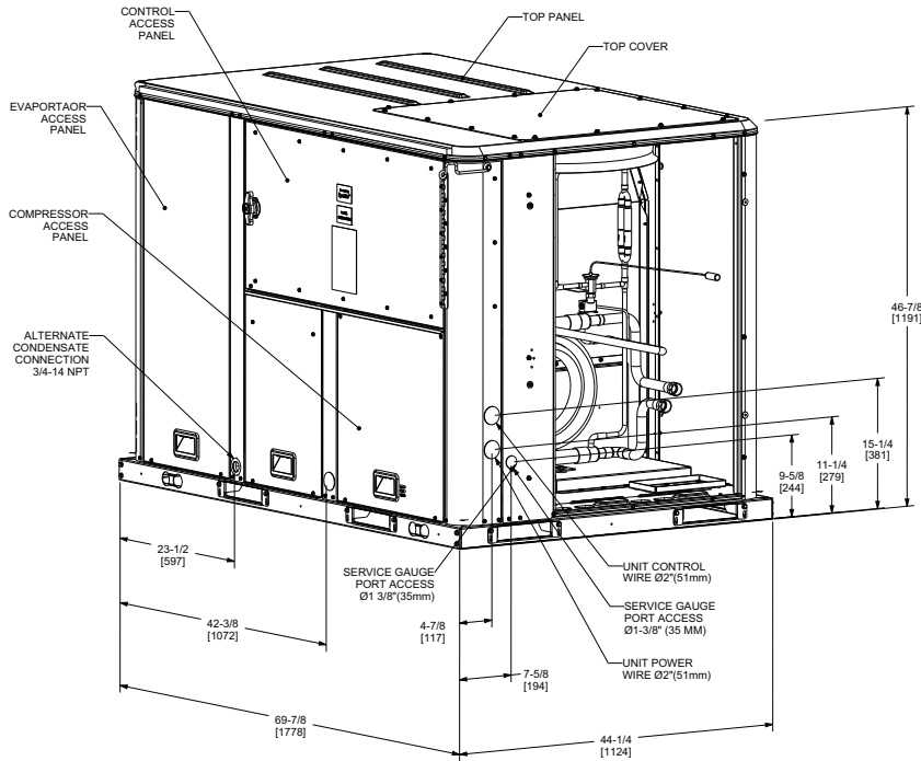
Figure 20. 3 to 5 ton cabinet – downflow airflow supply/return, through-the-base utilities
