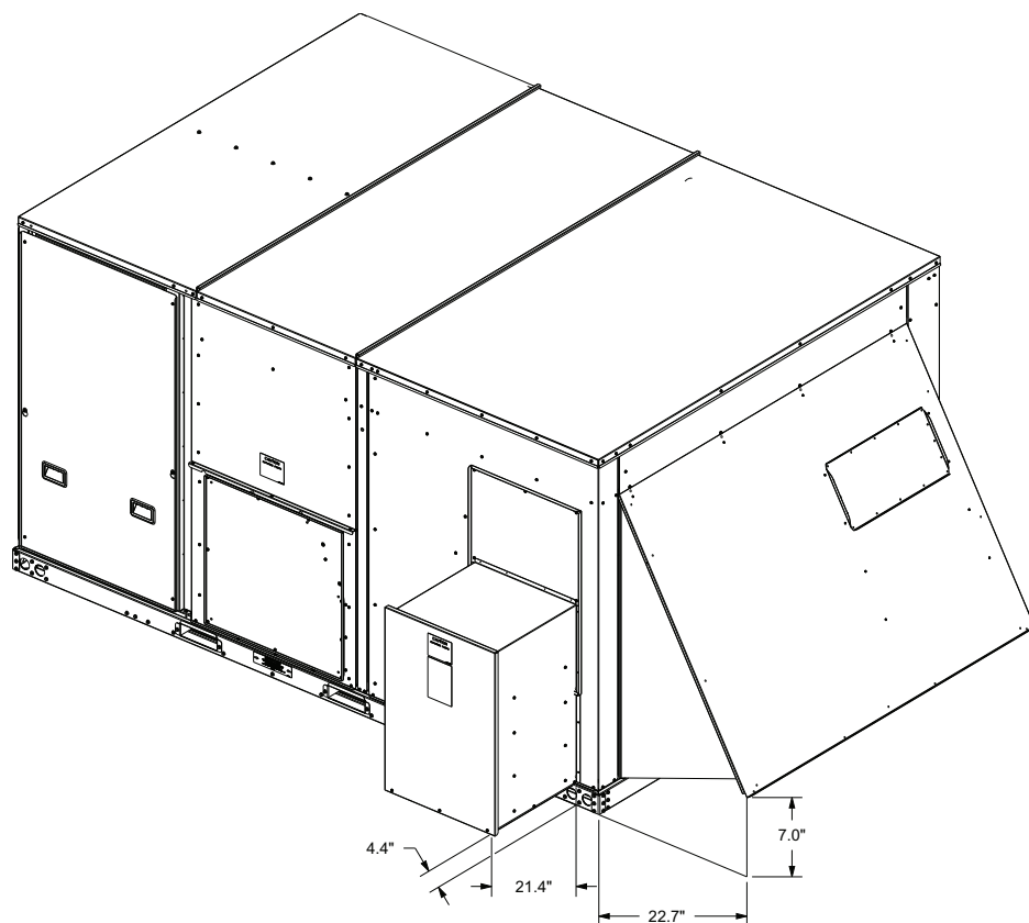
Figure 45. 12.5 to 25 ton cabinets – power exhaust
