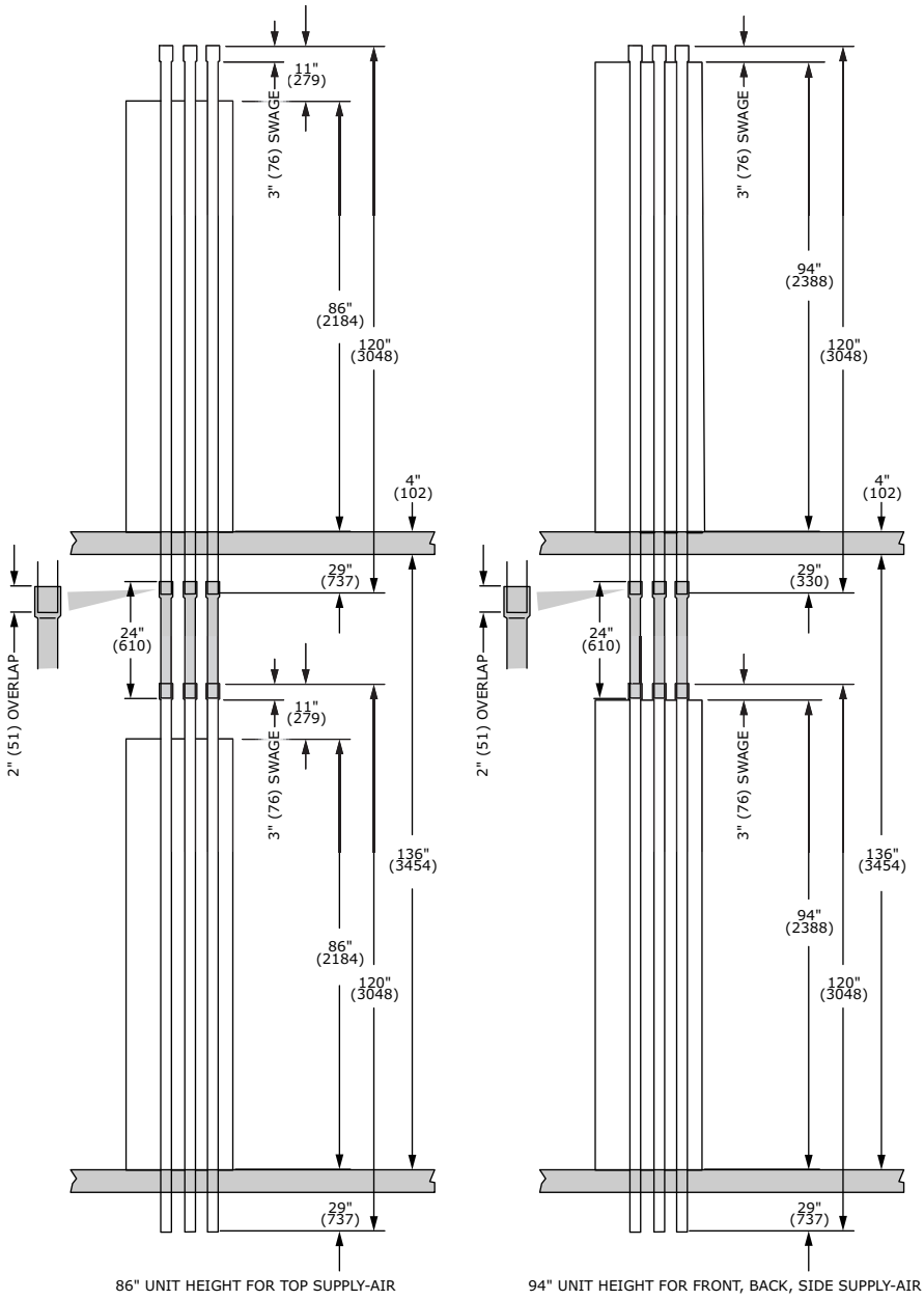
Figure 17. Riser extensions with 6-inch extended base
