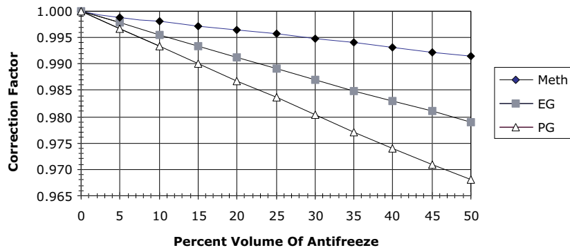
Figure 12. Cooling capacity correction factor
