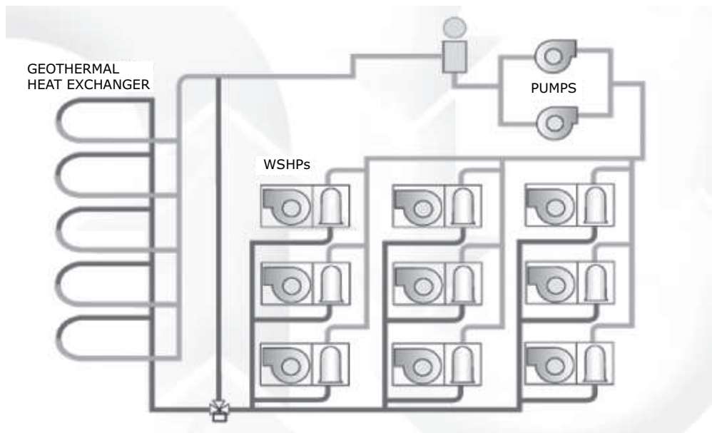
Figure 4. Ground source heat pump system
