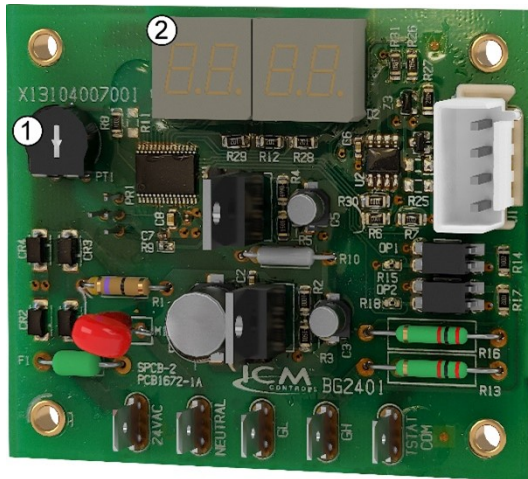
Figure 15. ECM control board
