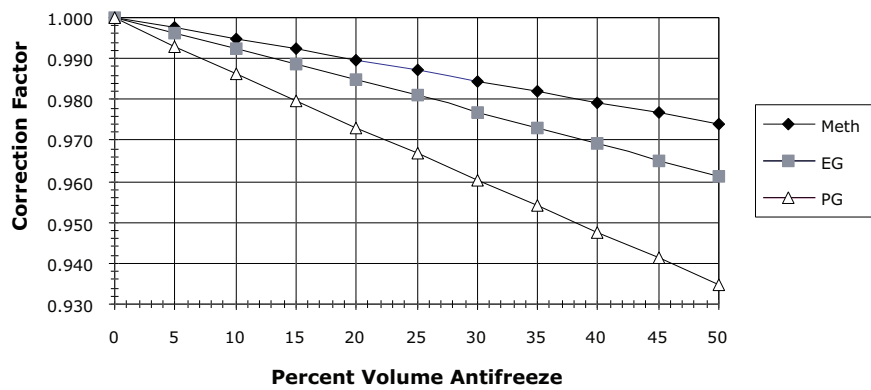
Figure 14. Water pressure drop correction factor
