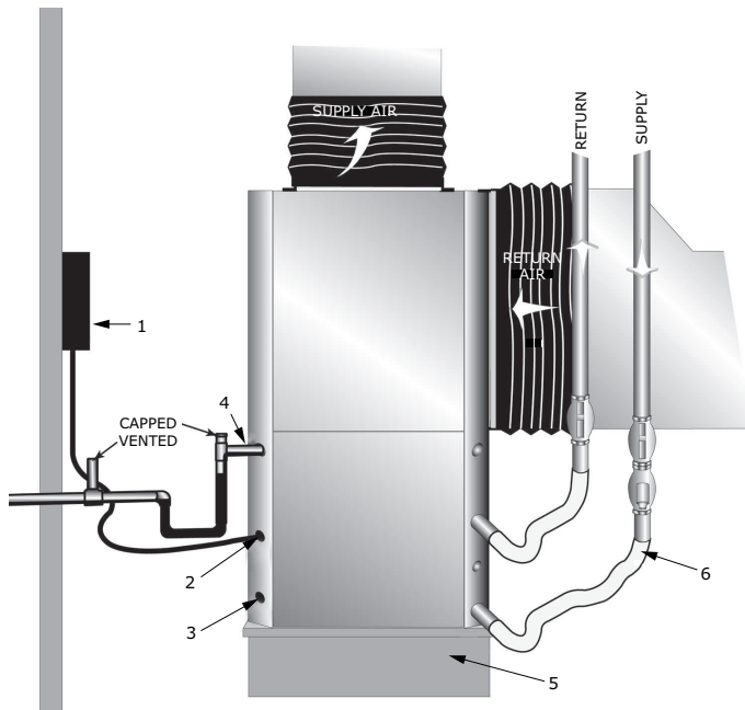
Figure 8. Installation of the 0.75 to 6 tons vertical
