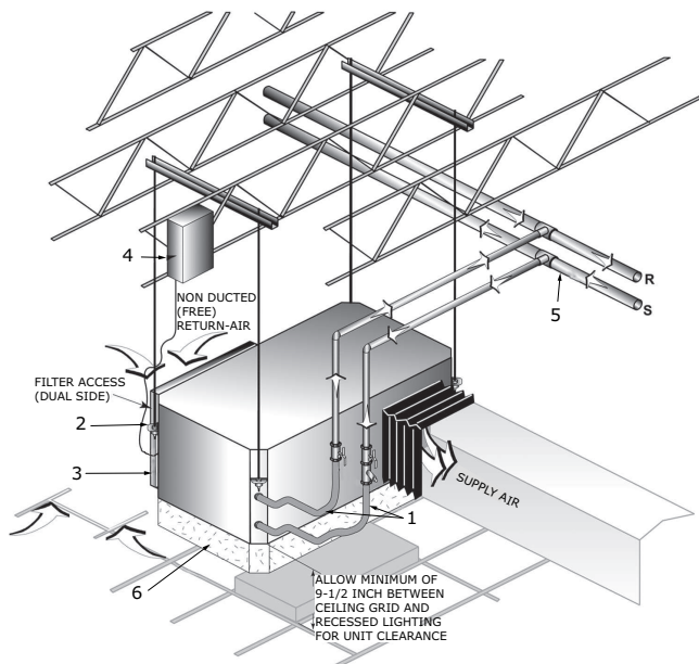
Figure 6. Central pumping system
