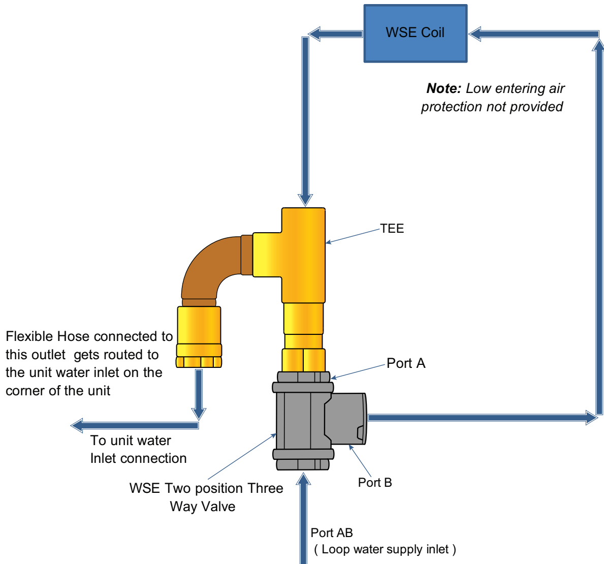
Figure 33. Waterside economizer coil piping diagram
