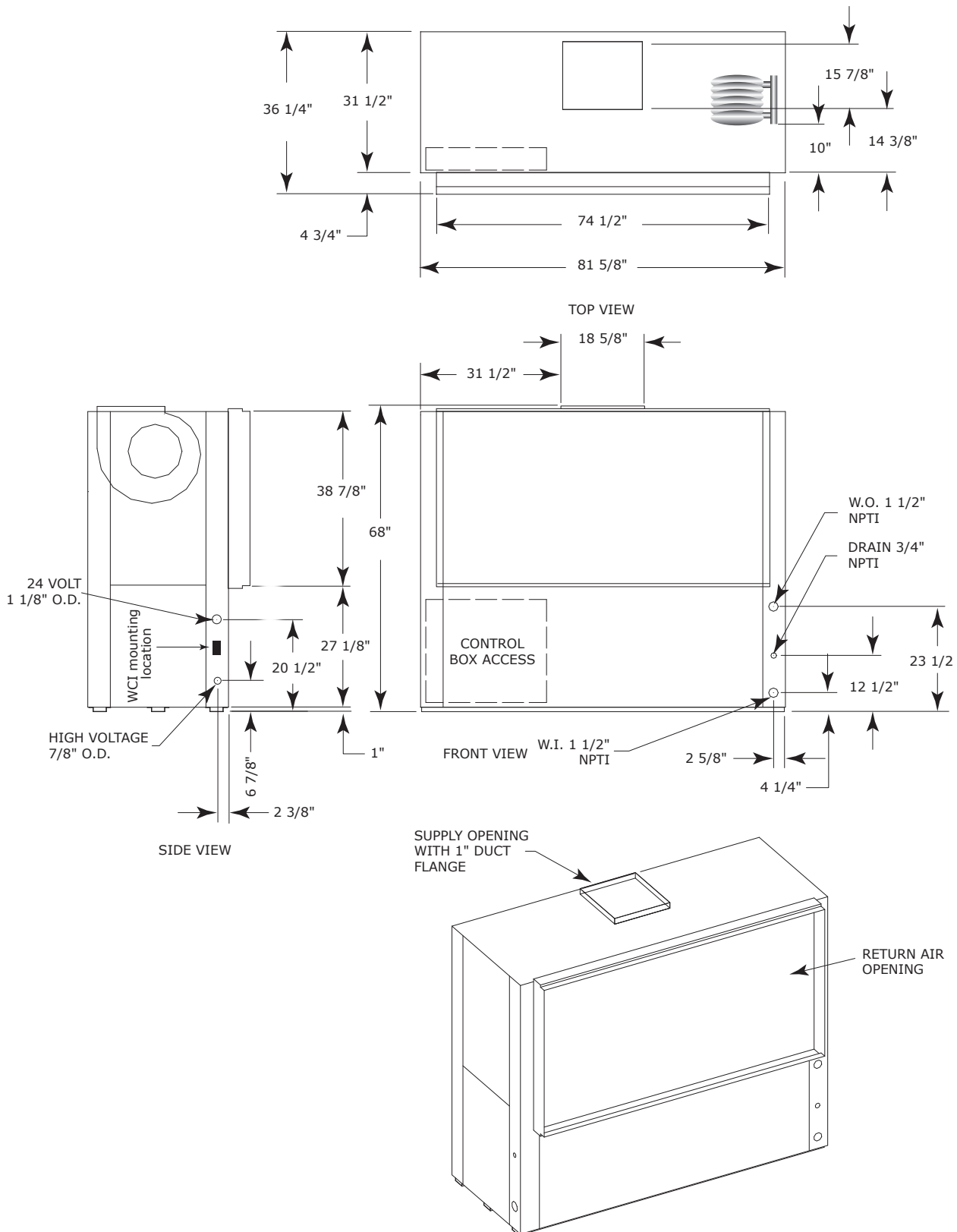
Figure 85. Front return/top supply 30 GEVK 12.5 to 15 tons (60 Hz); GEVK 10 and 12.5 tons (50 Hz)
