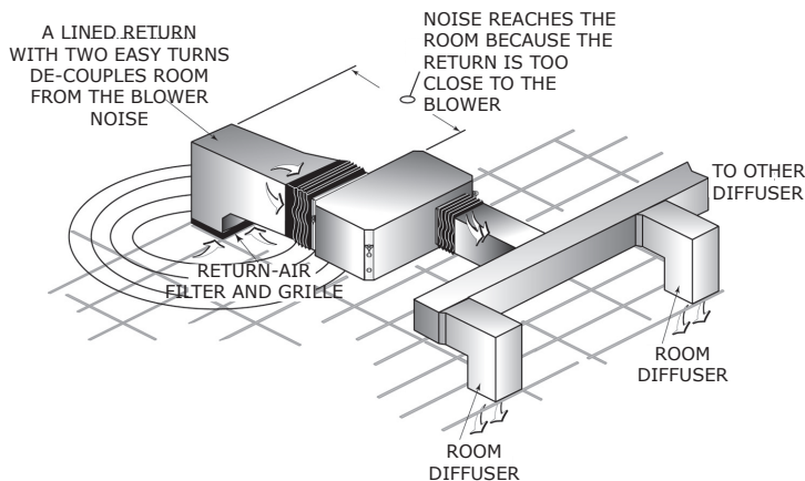
Figure 28. Improper return-air ducting
