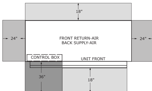
Figure 63. Clearance - GEV 12.5 to 25 tons
