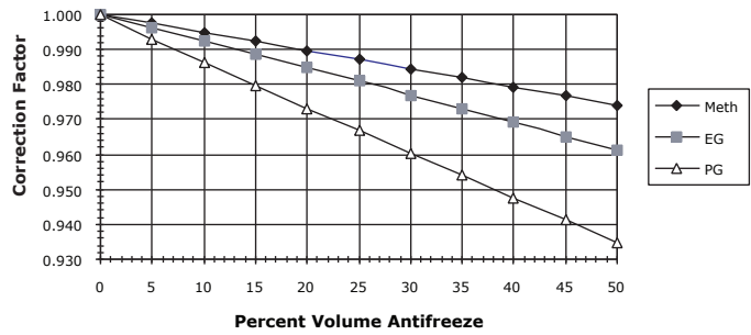
Figure 32. Water pressure drop correction factor
