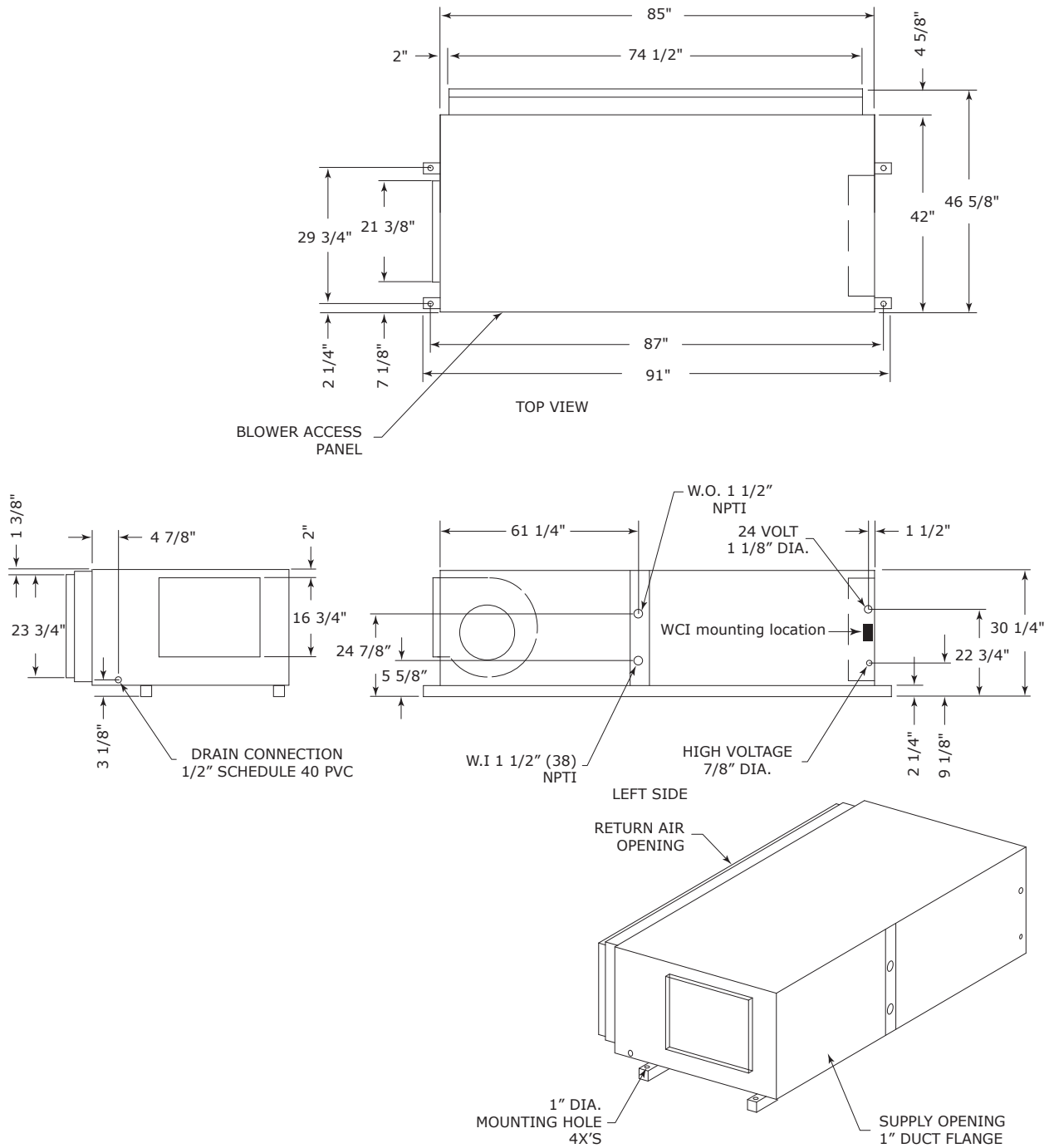
Figure 76. Right return/back supply GEHK 12.5 to 15 tons (60 Hz); GEHK 10 to 12.5 tons (50 Hz)
