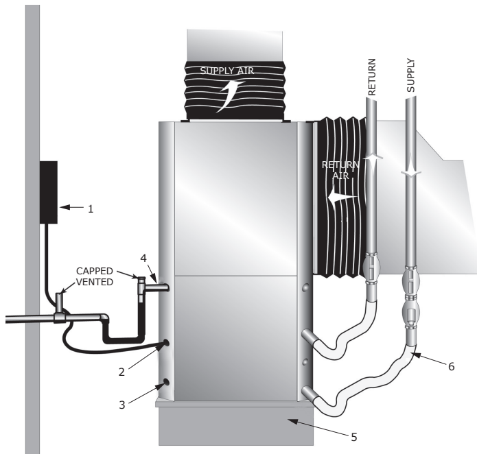
Figure 26. Installation of the 0.5 to 5 tons vertical
