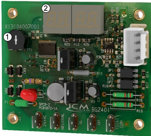
Figure 33. ECM control board
