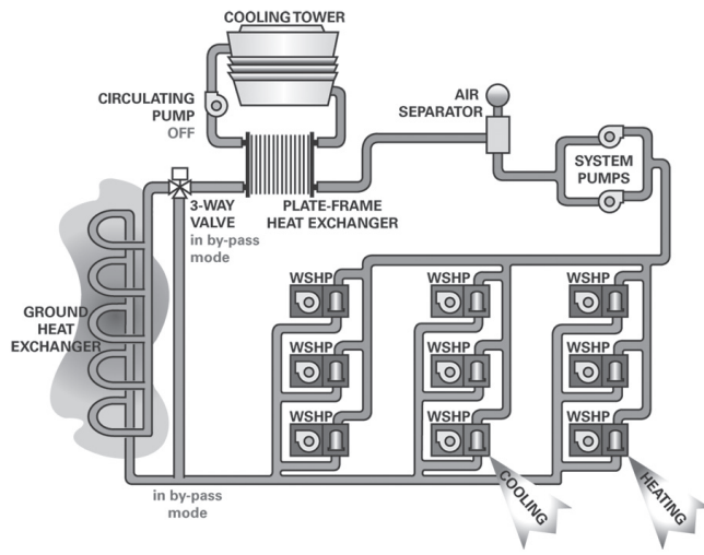
Figure 20. Waterside economizer system
