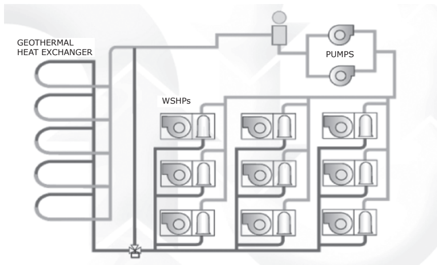
Figure 22. Ground source heat pump system
