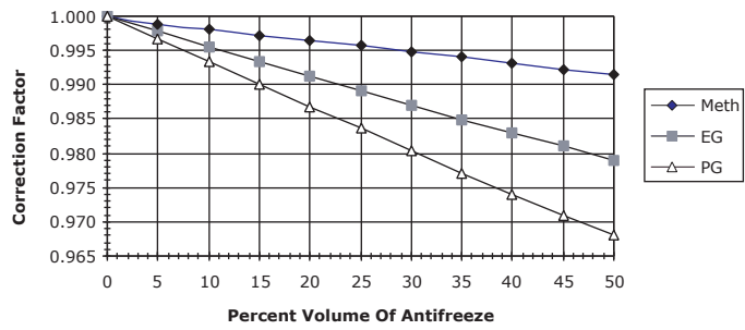
Figure 30. Cooling capacity correction factor
