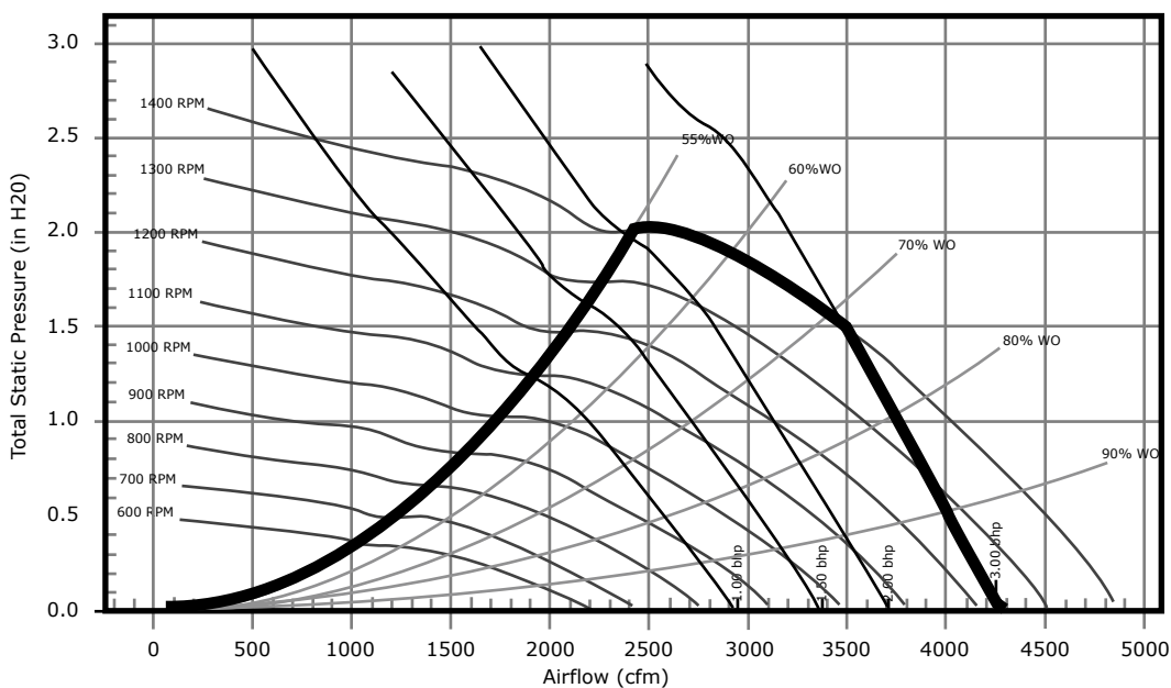
Figure 37. Fan performance curve 7.5 tons GEH090 6
