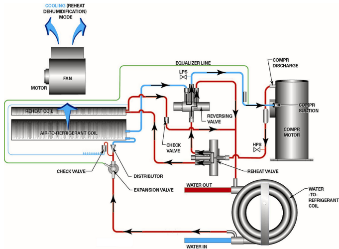
Figure 14. Hot gas reheat
