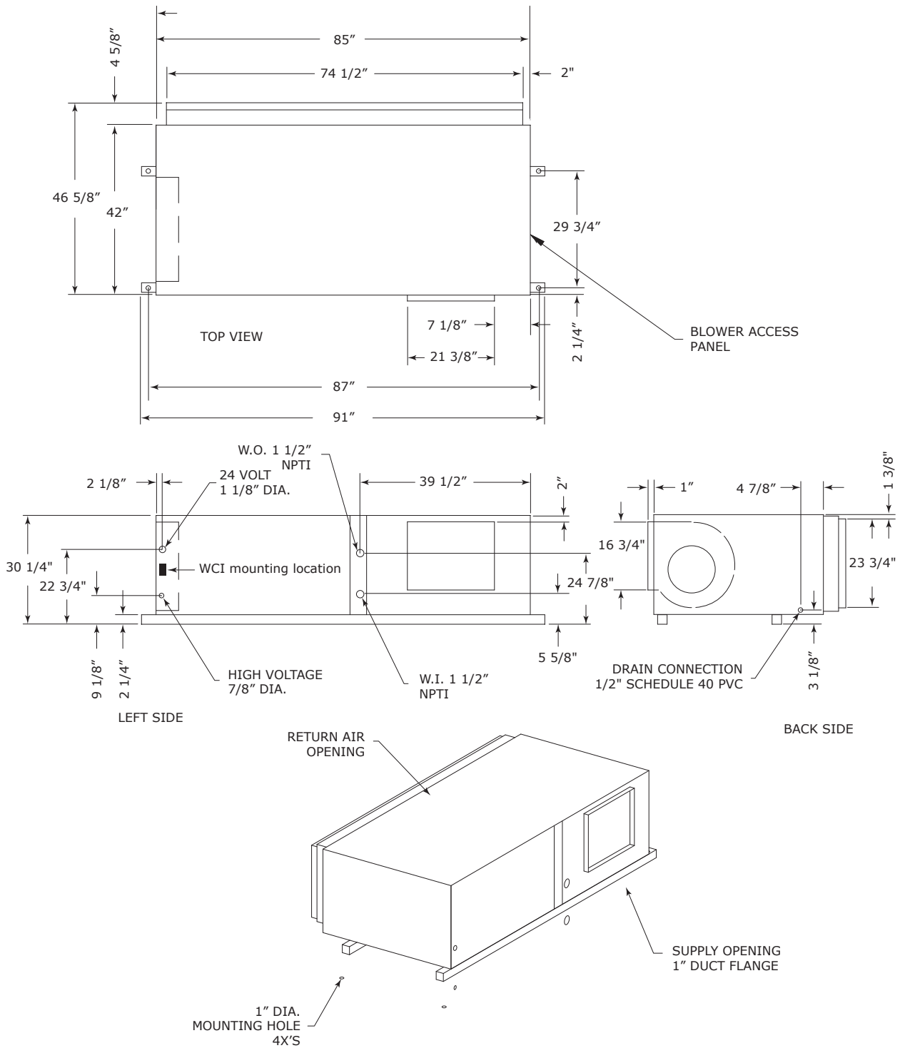
Figure 77. Left return/right supply GEHK 12.5 to 15 tons (60 Hz); GEHK 10 to 12.5 tons (50 Hz)
