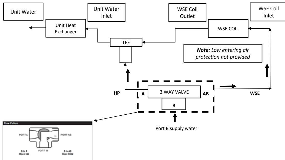
Figure 100. Waterside economizer piping diagram (6 to 25 tons)
