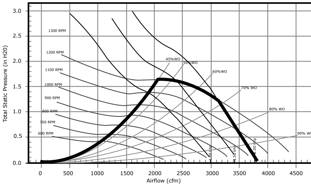
Figure 36. Fan performance curve (front/back supply) 6 tons GEV072 5
