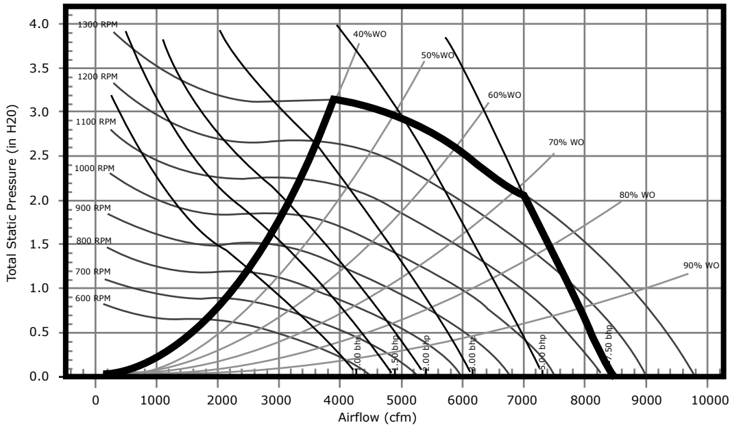
Figure 46. Fan performance curve 15 tons GEH180 15
