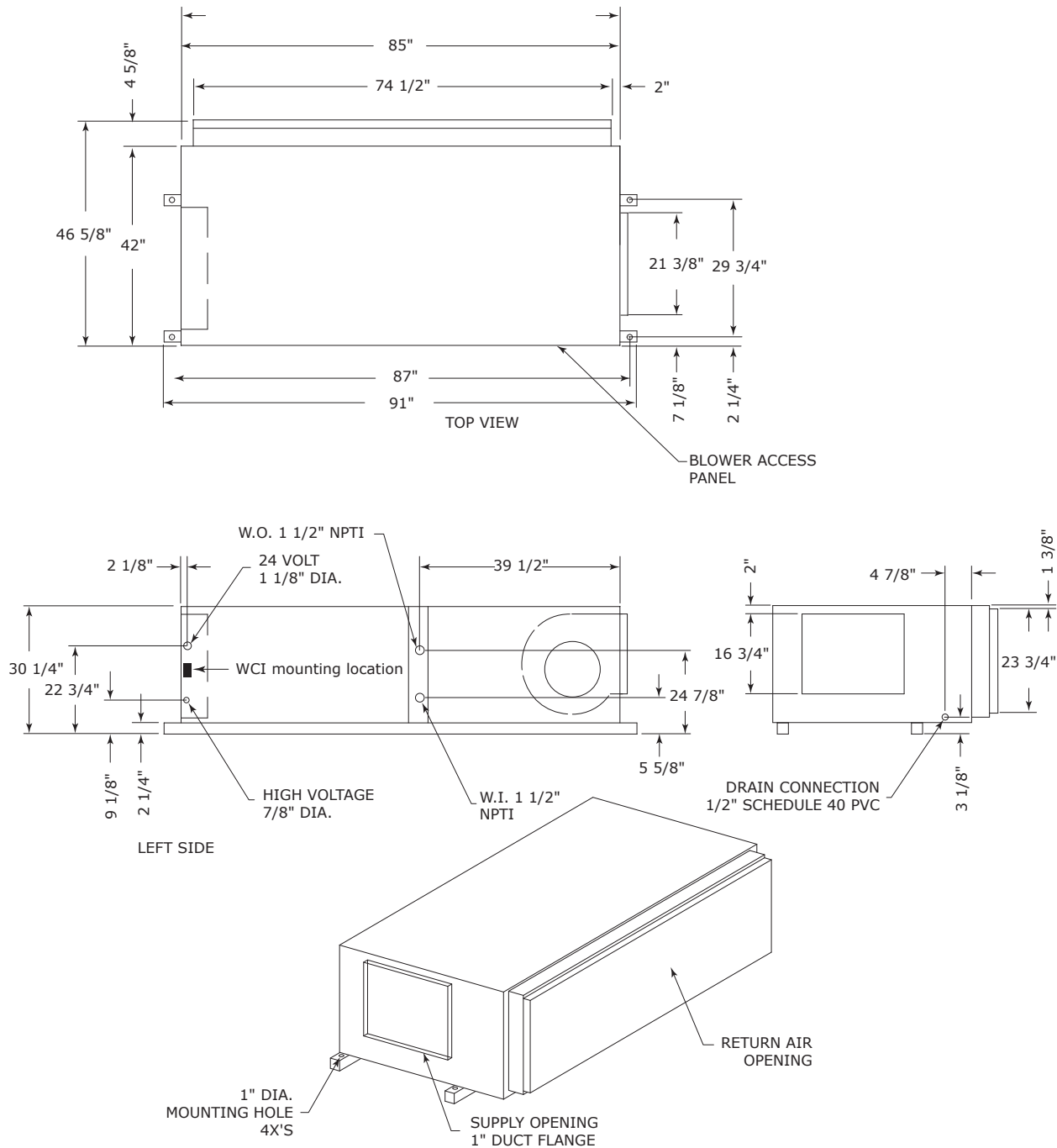
Figure 78. Left return/back supply GEHK 12.5 to 15 tons (60 Hz); GEHK 10 to 12.5 tons (50 Hz)
