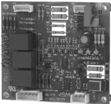
Figure 55. Deluxe 24V control board
