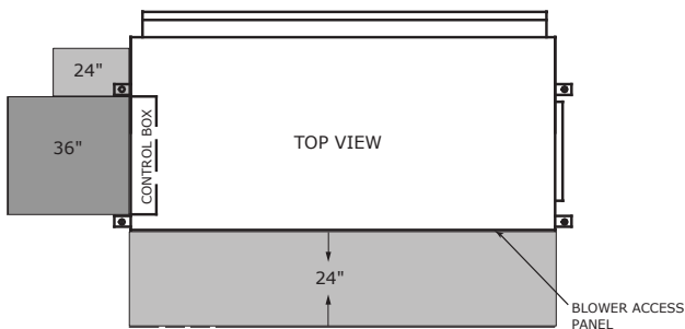
Figure 60. Clearance - GEH 6 to 15 tons
