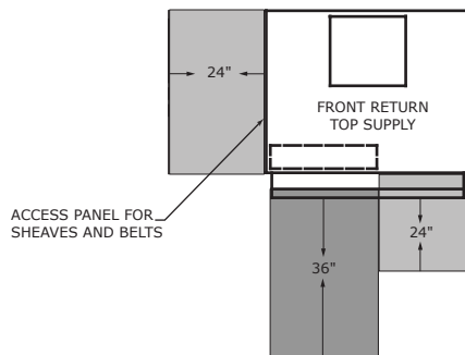
Figure 62. Clearance - GEV 6 to 10 tons
