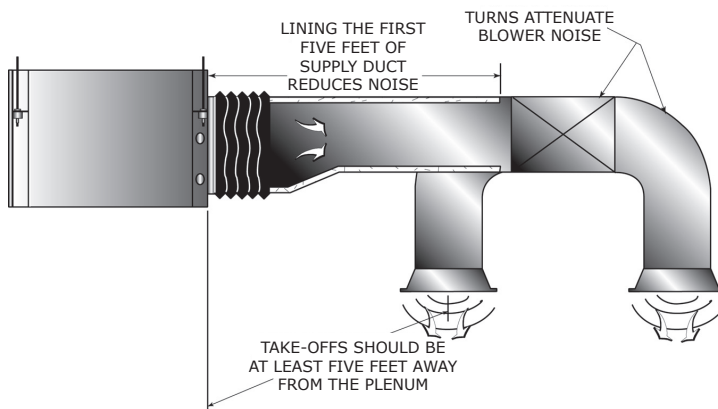
Figure 27. Desired supply air ducting
