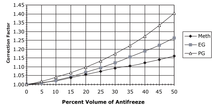
Figure 32. Water pressure drop correction factor
