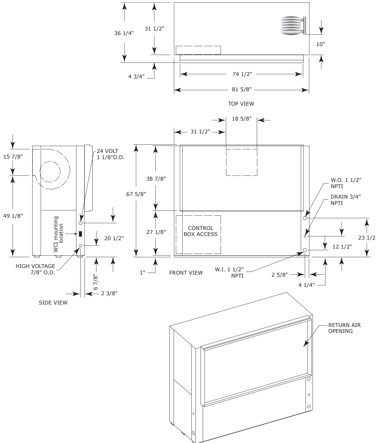
Figure 83. Front return/back supply 29 GEVK 12.5 to 15 tons (60 Hz); GEVK 10 and 12.5 tons (50 Hz)
