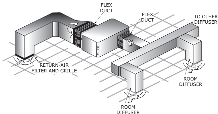
Figure 29. Proper return-air ducting
