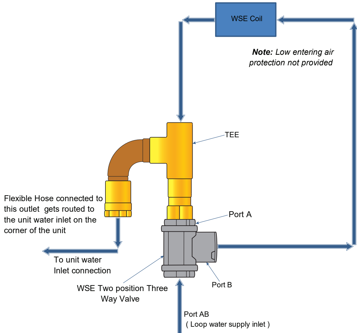
Figure 101. Waterside economizer coil piping diagram (0.5 to 5 tons)
