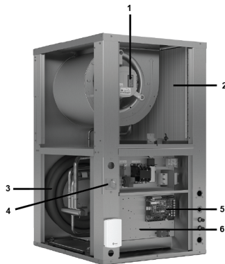
Figure 2. GEVK unit (0.5 to 5 tons)
