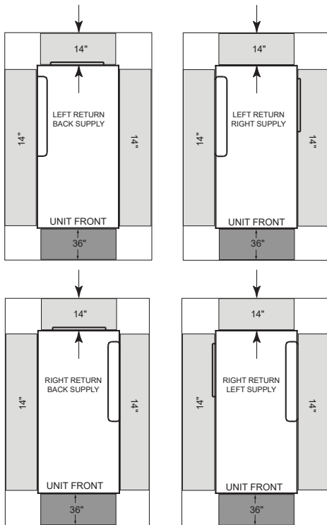
Figure 59. Clearances - GEH 0.5 to 5 tons
