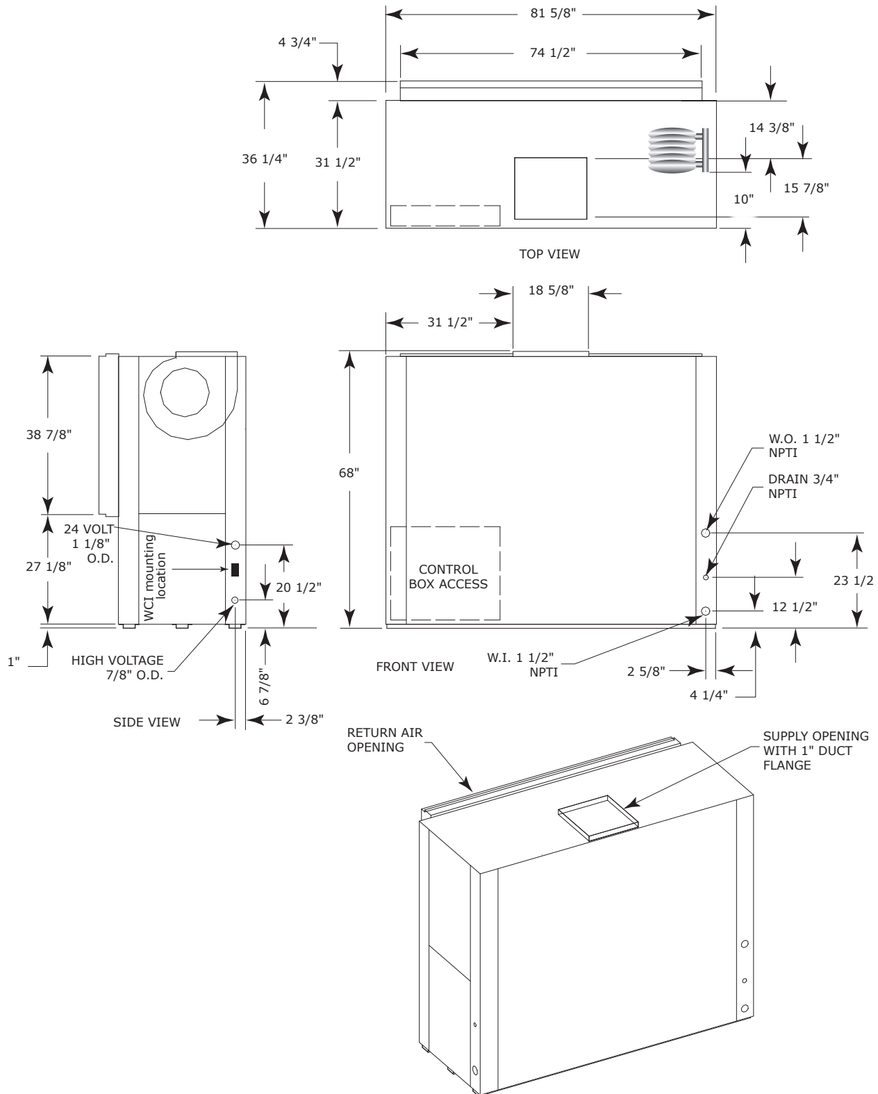
Figure 86. Back return/top supply 31 GEVK 12.5 to 15 tons (60 Hz); GEVK 10 and 12.5 tons (50 Hz)
