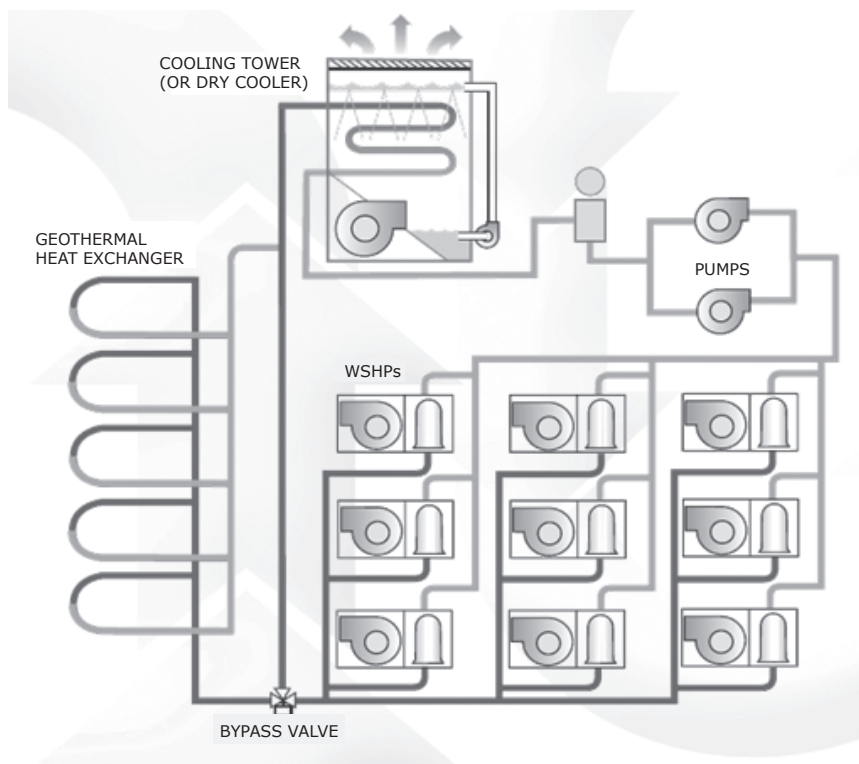
Figure 23. Hybrid system
