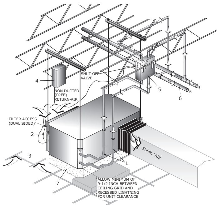
Figure 25. Distributed pumping system
