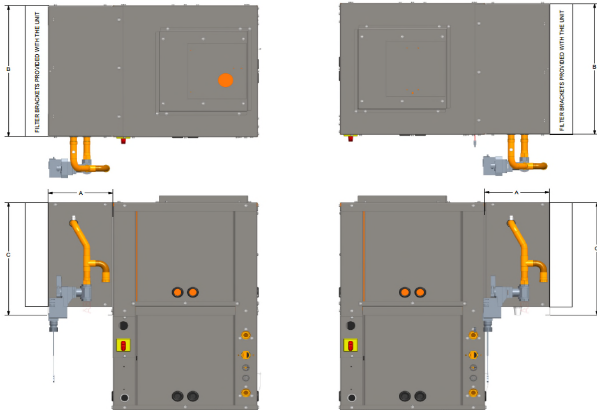
Figure 92. Waterside economizer (GEVK)
