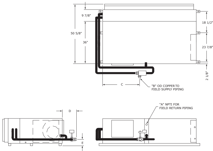
Figure 95. GEHK 6 to 10 tons (60 Hz), GEHK 6 to 7.5 tons (50 Hz) - left return with waterside economizer 37
