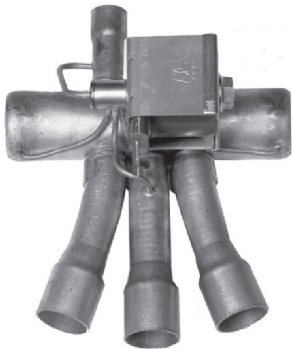
Figure 15. Reversing valve
