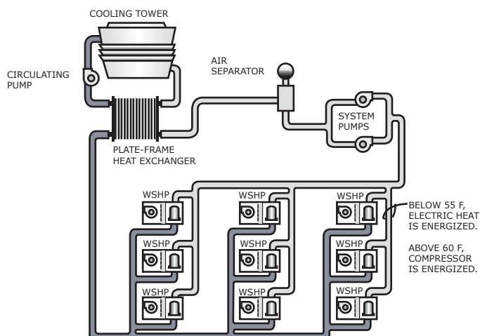
Figure 5. Electric heat system
