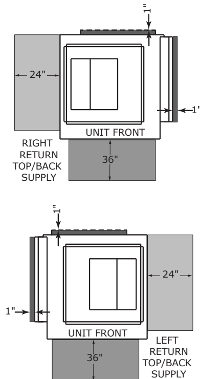
Figure 61. Clearance – GEV 0.5 to 5 tons
