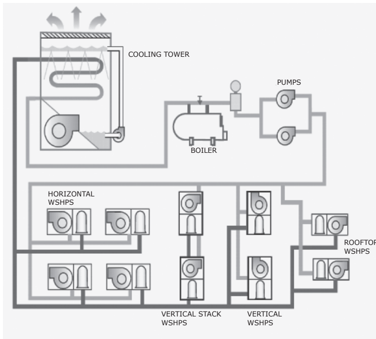
Figure 21. Conventional water-source heat pump system
