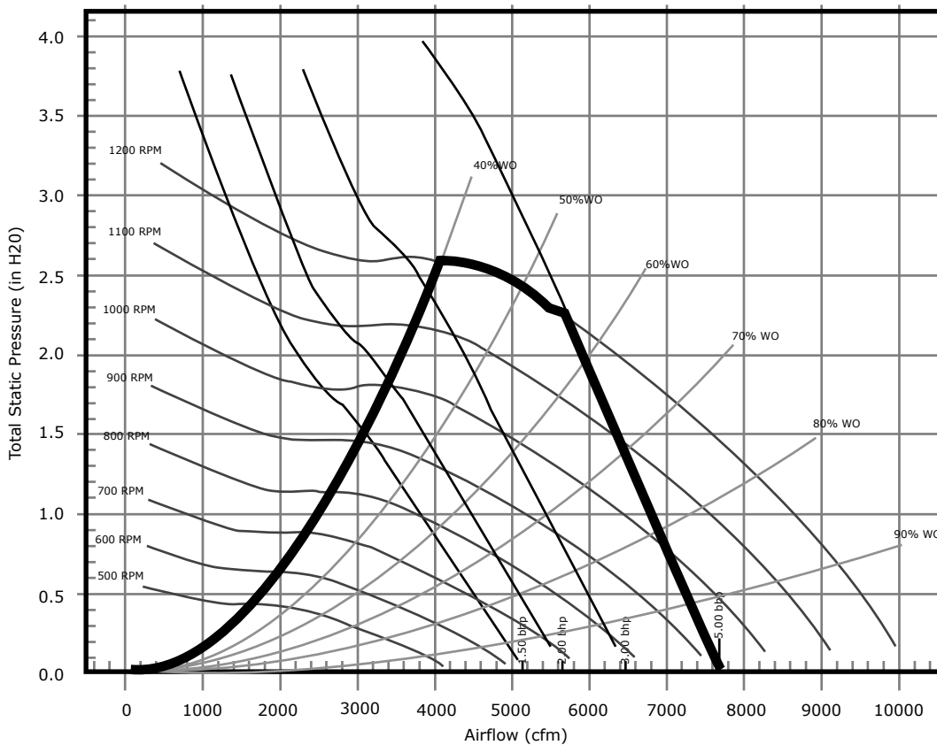
Figure 44. Fan performance curve (top supply) 12.5 tons GEV150 13
