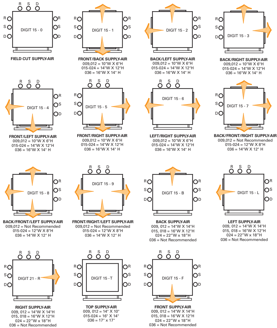
Figure 15. Supply-air arrangements
