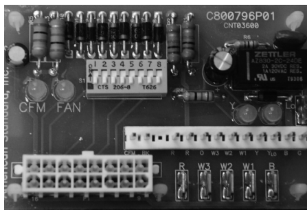
Figure 4. ECM control board and dip switch setting
