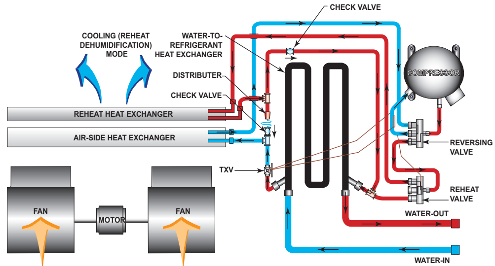
Figure 12. Hot gas reheat
