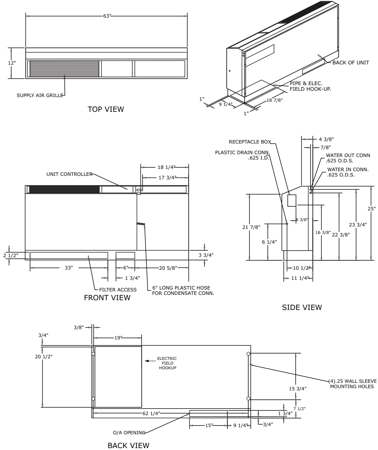
Figure 29. GEC 0.5 to 1.5 tons (60 Hz), 0.5 to 1.25 tons (50 Hz) - cabinet (RH) piping extended length
