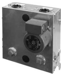
Figure 14. Pump module hose kit
