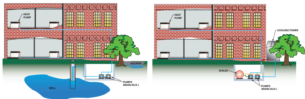
Figure 20. Geothermal systems
