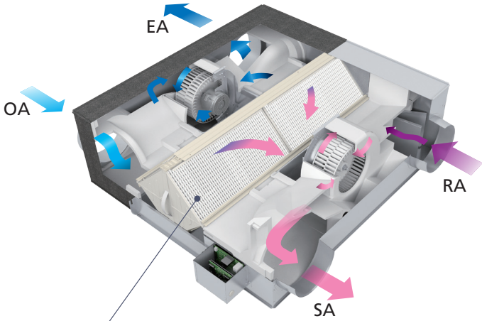
The Concept Of Sensible Heat and Latent Heat Exchange Using Lossnay Core
