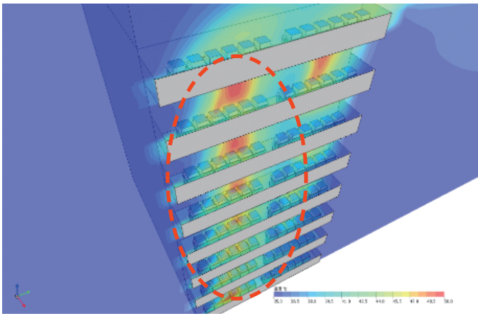
Installation on Each Floor a High-Rise Building
