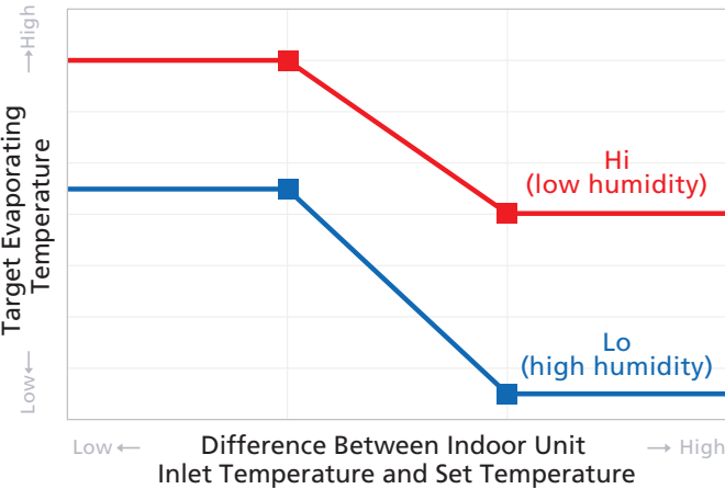
Image of Evaporating Temperature Control During High Sensible Heat Operation in Full Cooling Mode
