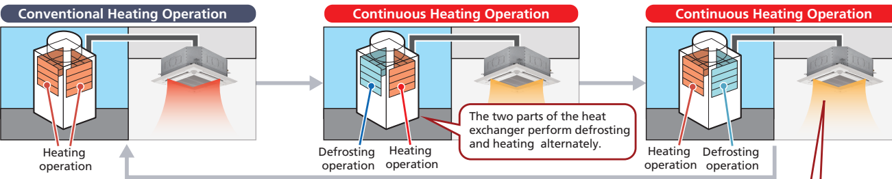
Image of Continuous Heating Operation (Combination)
