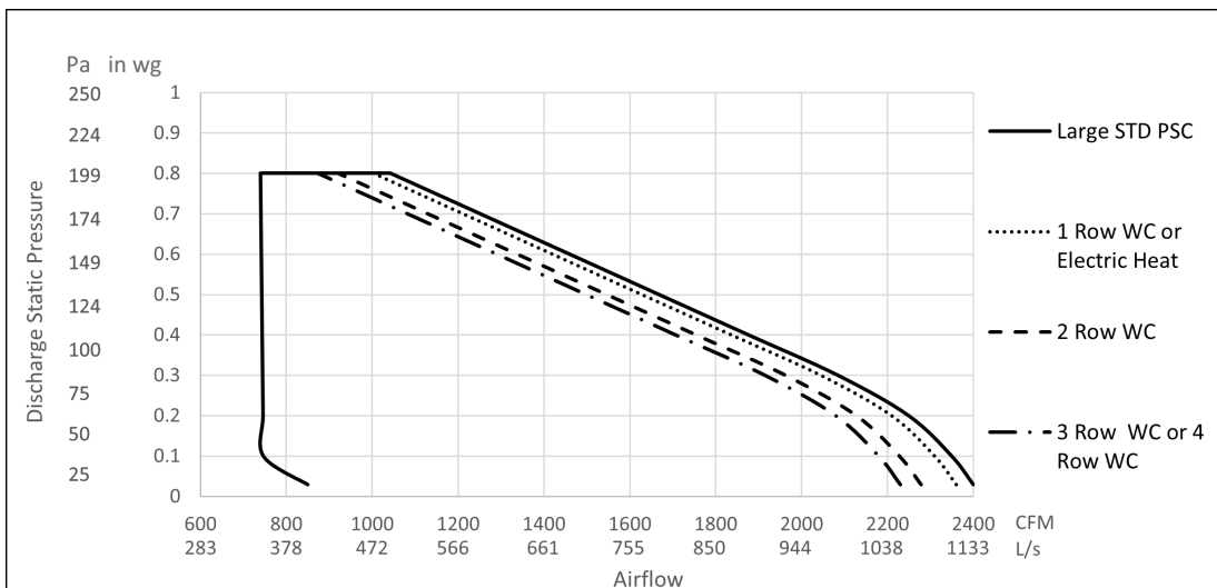
Figure 21. Performance data fan curves, series VSxG large standard – PSC
