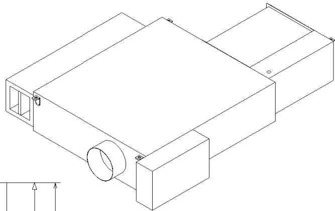
Figure 54. Low-height series – electric (LSEF) with thinline suppressor – fan sizes DS02
