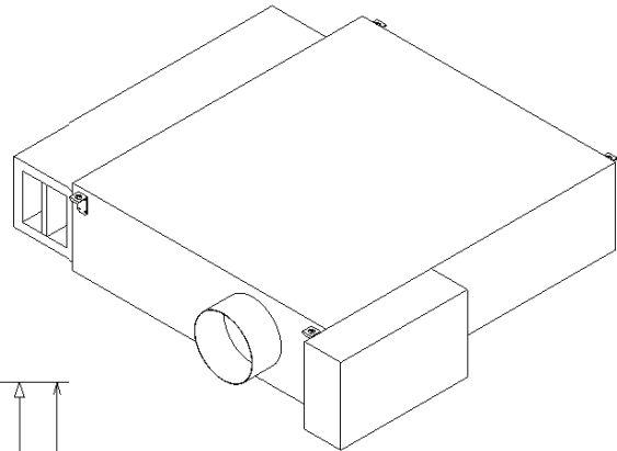
Figure 52. Low-height series – cooling only (LSCF) with thinline suppressor – fan sizes DS02
