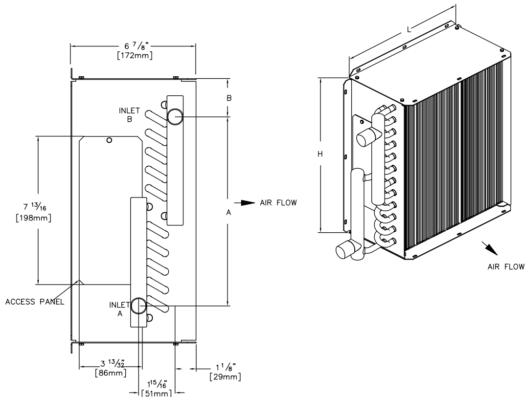
Figure 59. Low-height series coil assembly (2 row)
