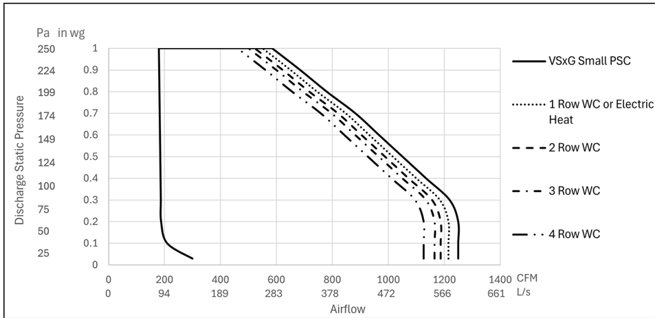
Figure 20. Performance data fan curves, series VSxG medium standard – PSC
