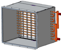
Figure 14. Hot water coil
