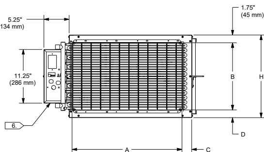
DISCHARGE VIEW
