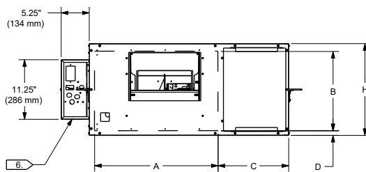
DISCHARGE VIEW
