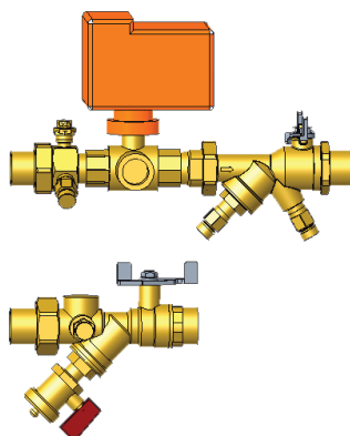
Figure 37. Belimo valve piping package
