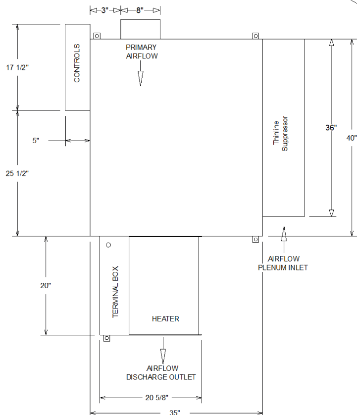
Unit Model LSEF Nominal Valve Size & Depth 8" Dia. x 4" Depth Nominal Fan Size DS02 Fan Filter Size 7" x 7" x 1"
