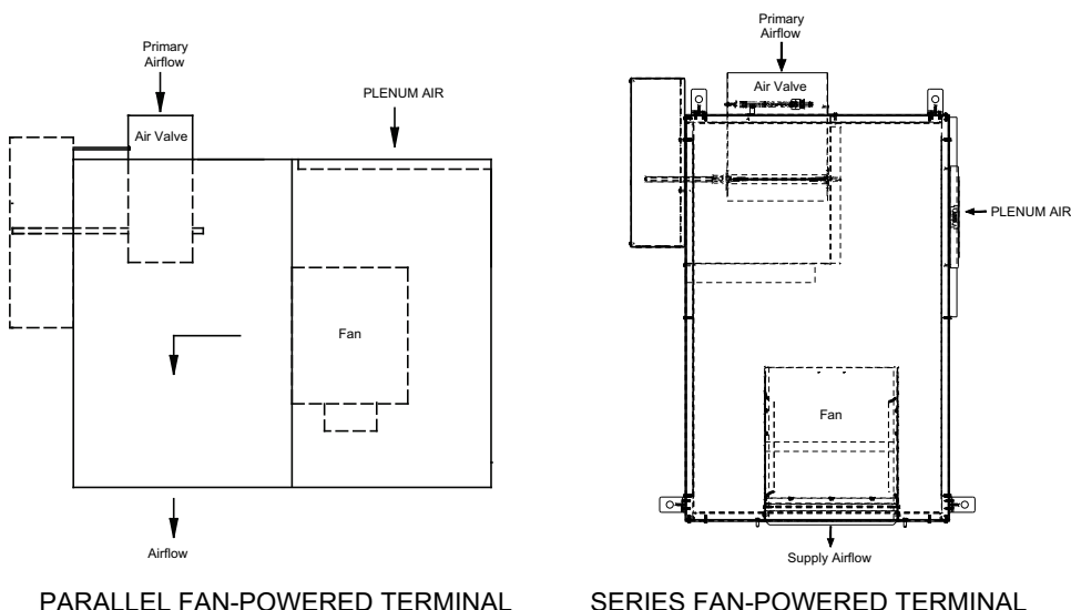
Figure 12. Parallel and series fan-powered terminal
