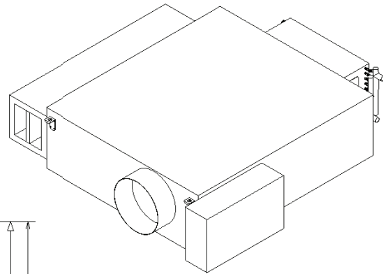
Figure 56. Low-height series – hot water (LSWF) with thinline suppressor – fan size DS03
