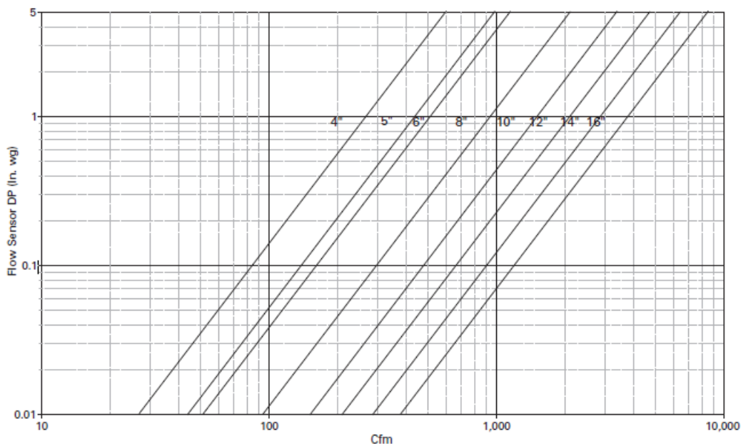
Figure 27. Flow sensor single vs. airflow delivery
