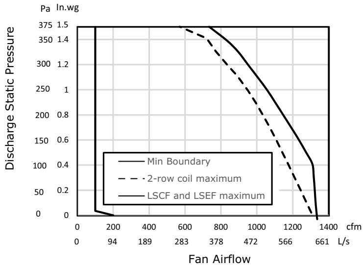
Figure 25. Performance data fan curves, LSxS DS02 – ECM
