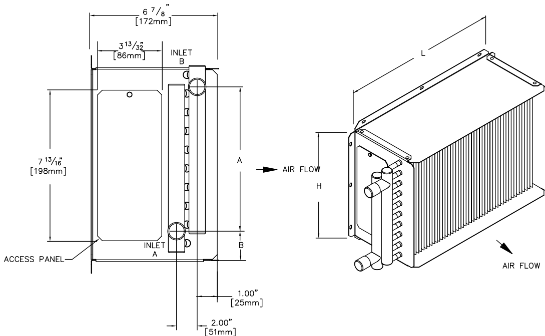
Figure 58. Low-height series coil assembly (1 row)
