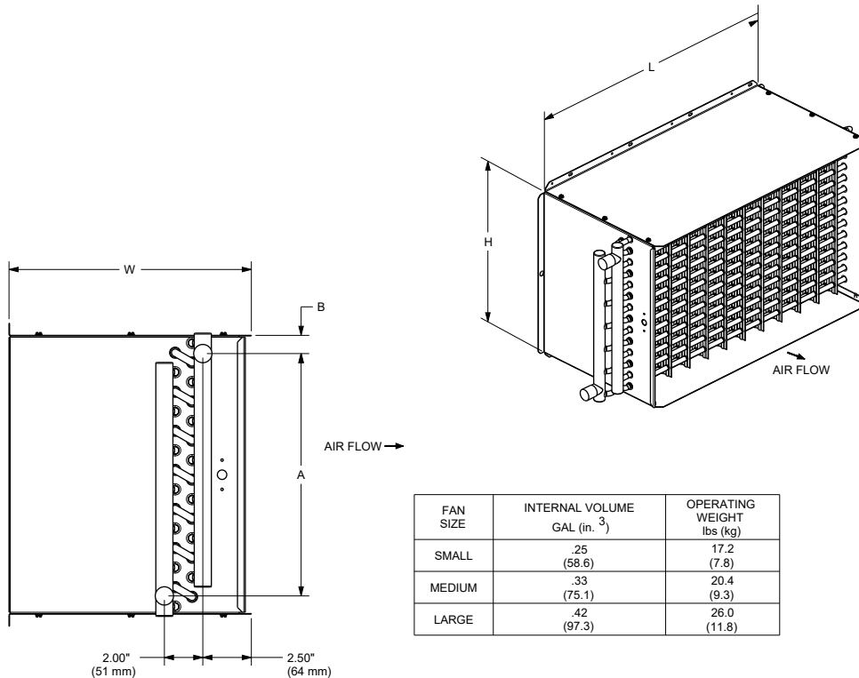
HEADER SIDE VIEW
