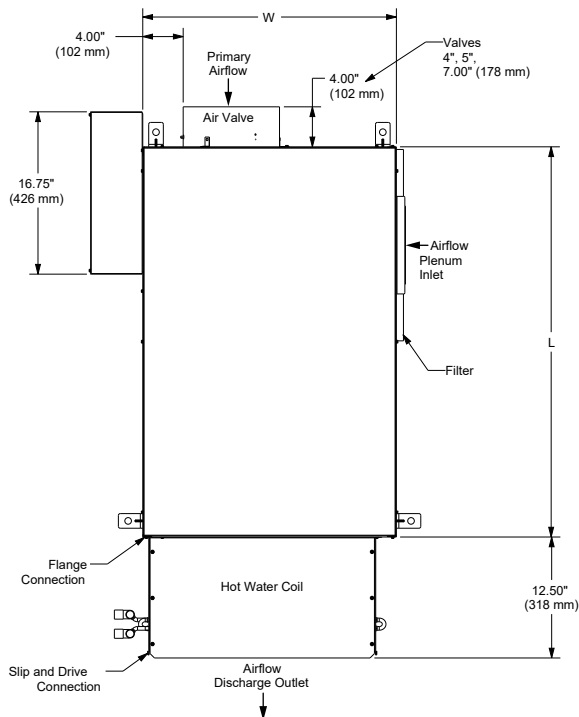
TOP VIEW
