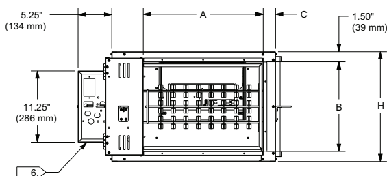
DISCHARGE VIEW
