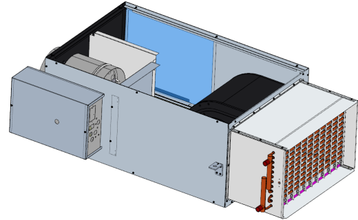
Figure 18. Series with hot water heat and ECM
