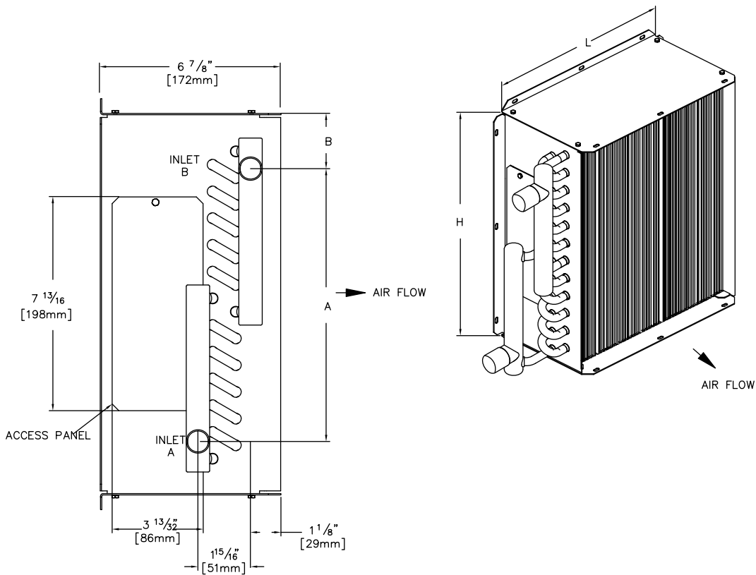
Figure 38. Low-height series coil assembly (2 row)
