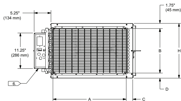
DISCHARGE VIEW
