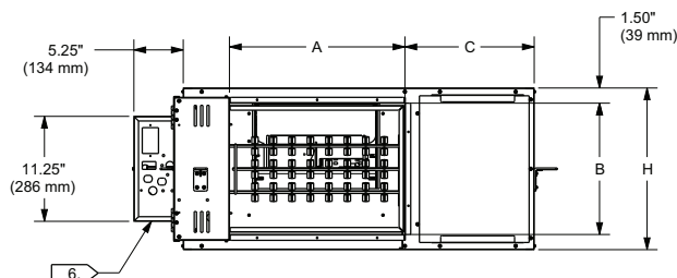
DISCHARGE VIEW
