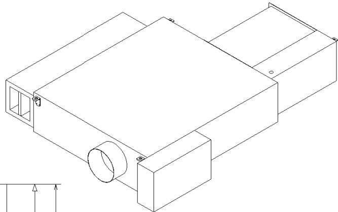
Figure 33. Low-height series — electric (LSEF) with thinline suppressor — fan sizes DS02
