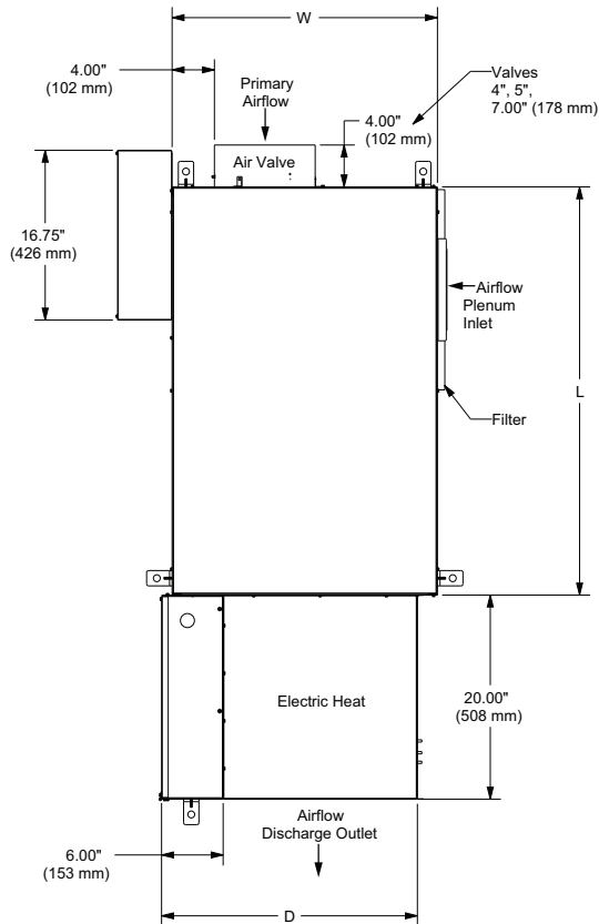
TOP VIEW
