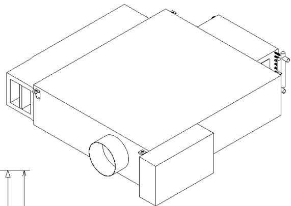
Figure 32. Low-height series — hot water (LSWF) with thinline suppressor — fan sizes DS02
