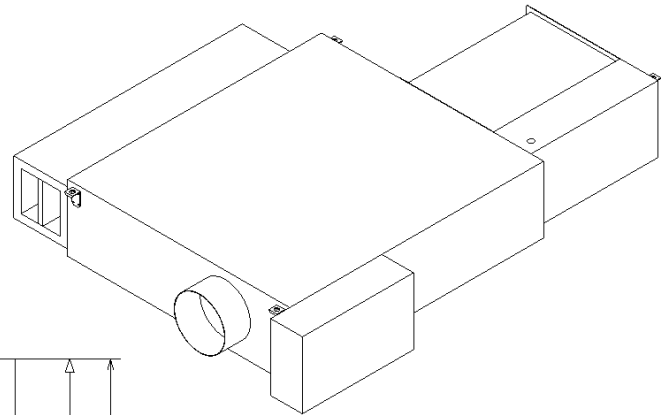
Figure 36. Low-height series — electric (LSEF) with thinline suppressor — fan size DS03
