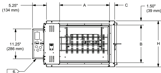
DISCHARGE VIEW
