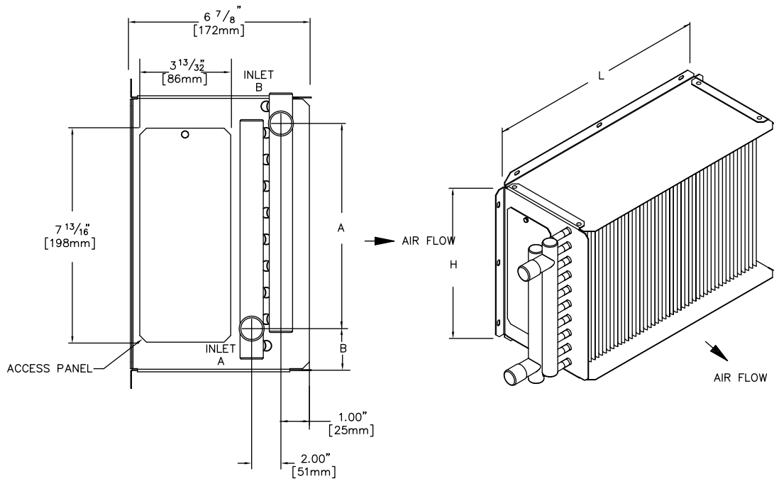
Figure 37. Low-height series coil assembly (1 row)
