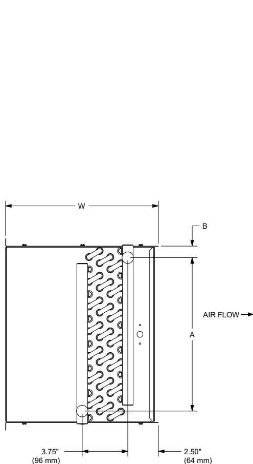
HEADER SIDE VIEW
