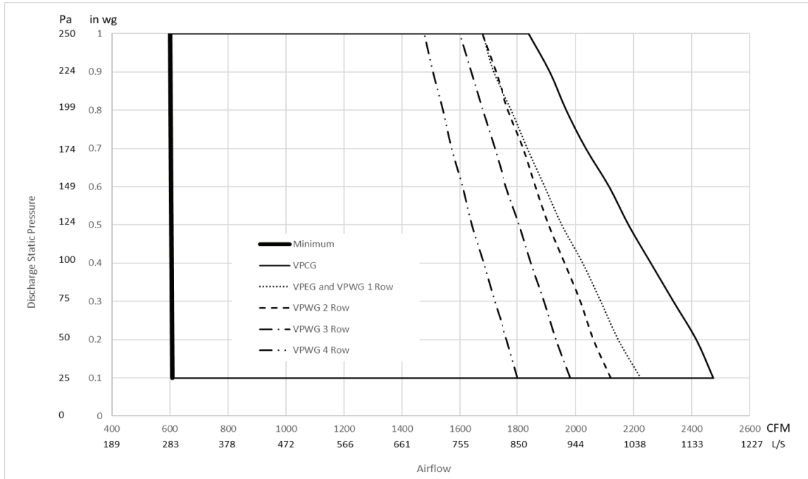
Figure 23. Performance data fan curves, parallel large – ECM
