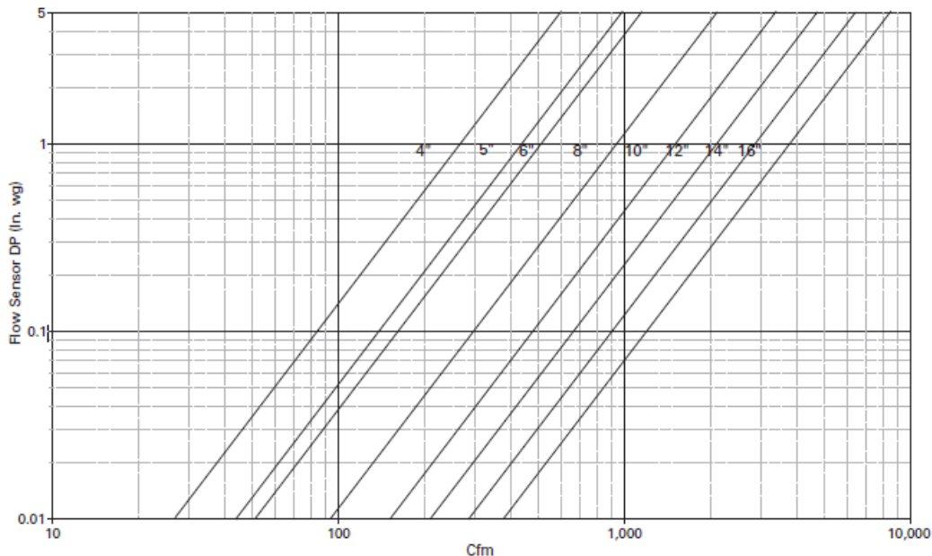
Figure 25. Flow sensor single vs. airflow delivery
