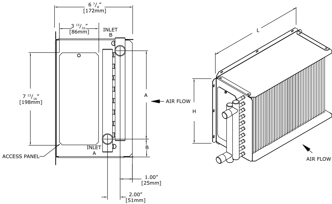
Figure 54. Low-height parallel coil assembly (1 row)
