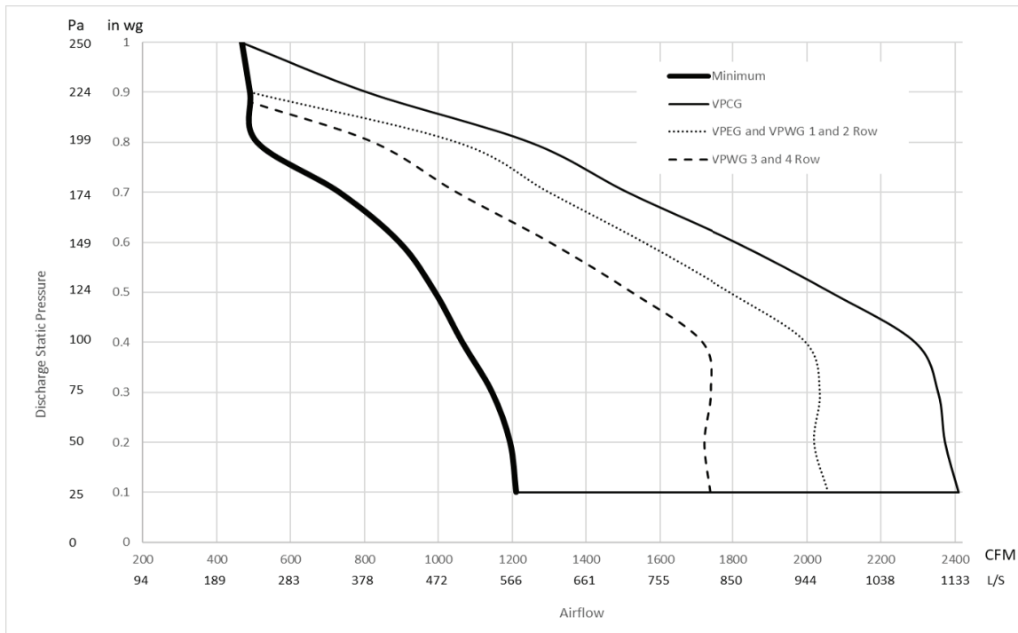
Figure 23. Performance data fan curves, parallel large – ECM
