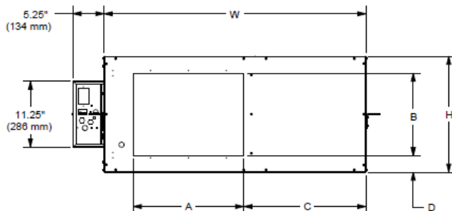
DISCHARGE VIEW
