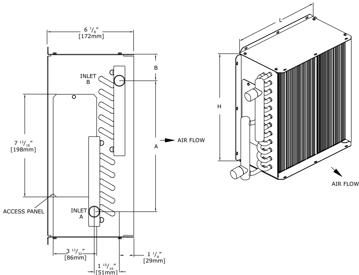
Figure 57. Low-height parallel discharge water coil assembly (2 row)
