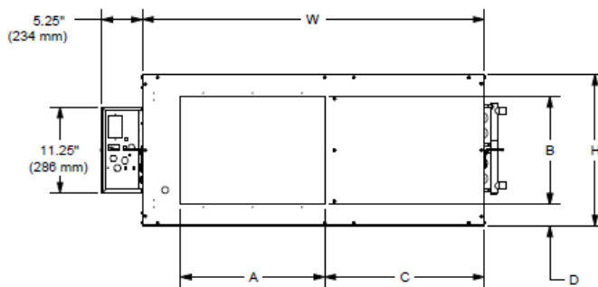
DISCHARGE VIEW
