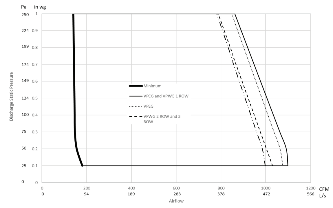
Figure 19. Performance data fan curves, parallel small – ECM
