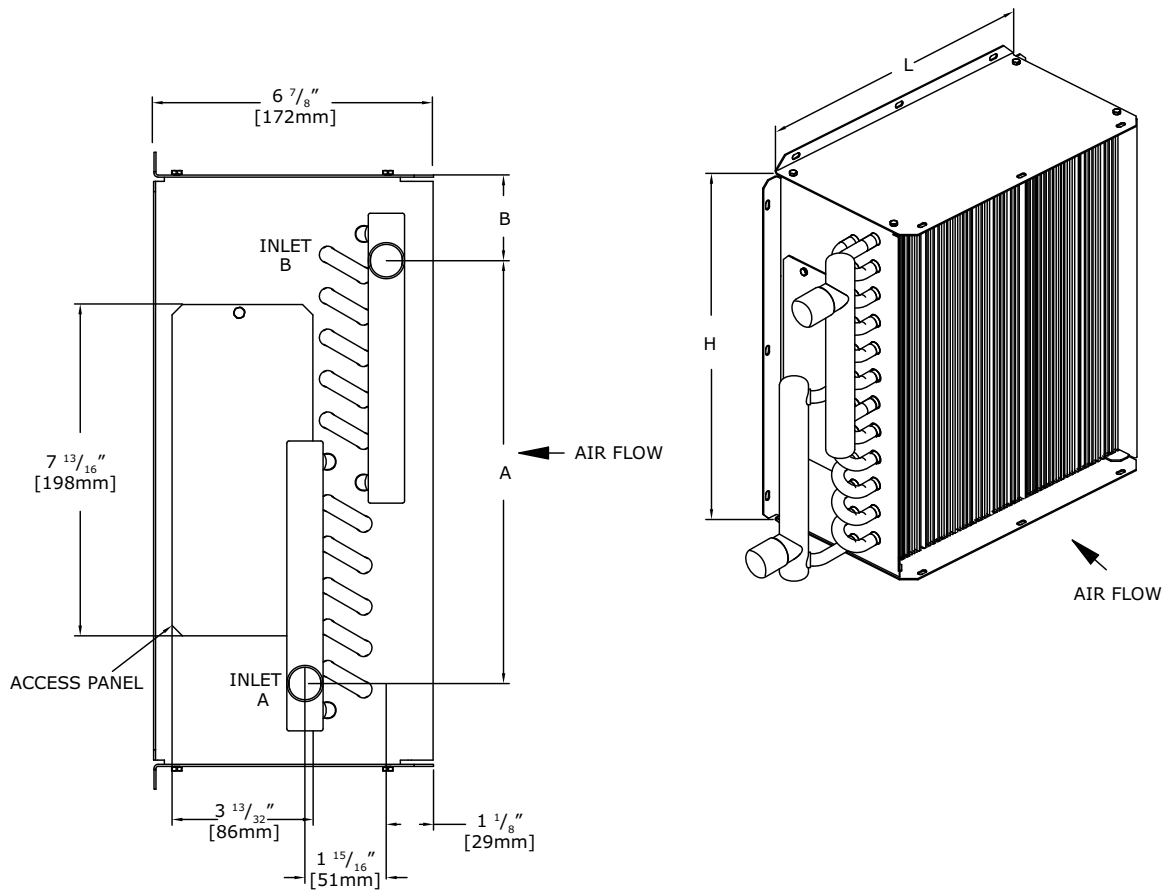
Figure 55. Low-height parallel coil assembly (2 row)
