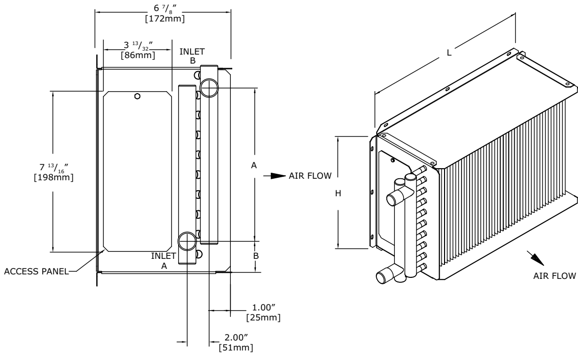
Figure 56. Low-height parallel discharge water coil assembly (1 row)
