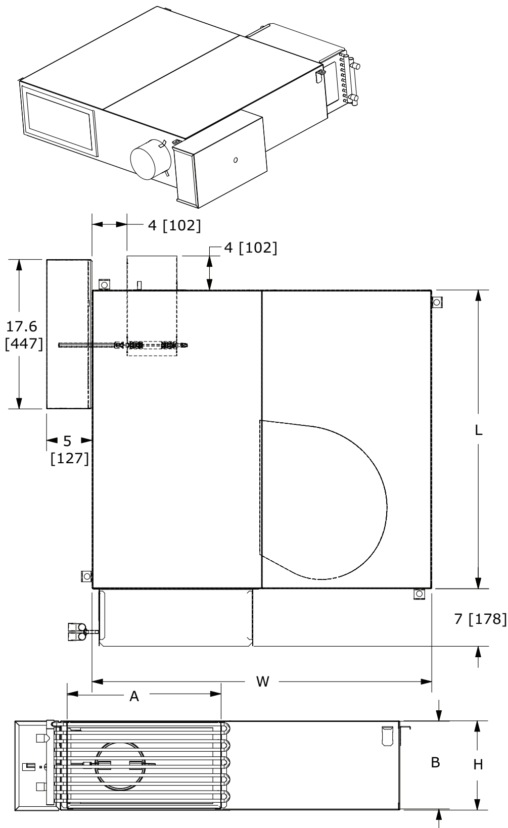
Figure 50. Low-height parallel – hot water (LPWF)
