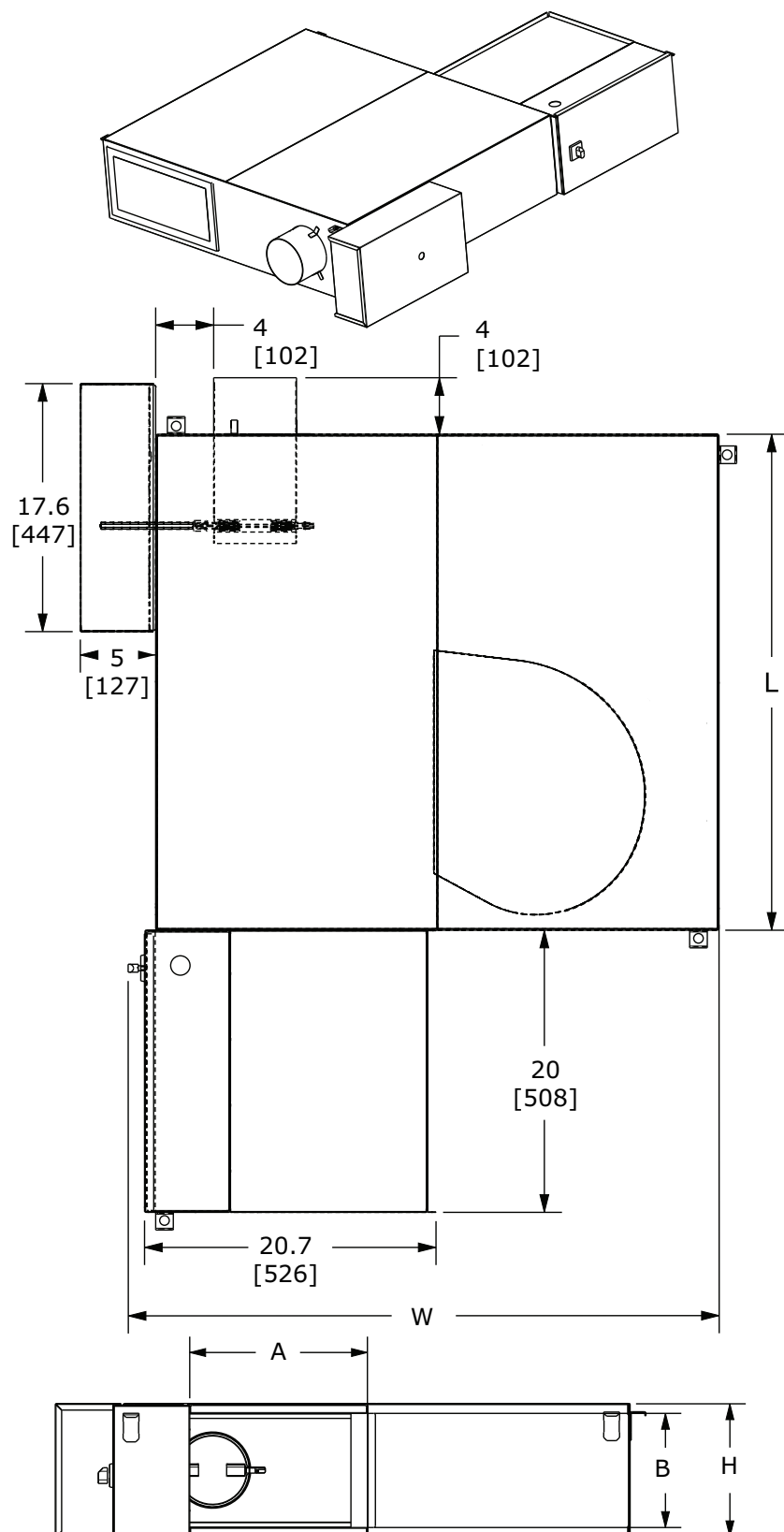
Figure 52. Low-height parallel – electric (LPEF)
