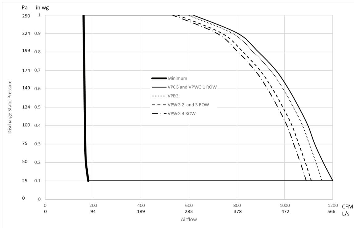
Figure 19. Performance data fan curves, parallel small – ECM
