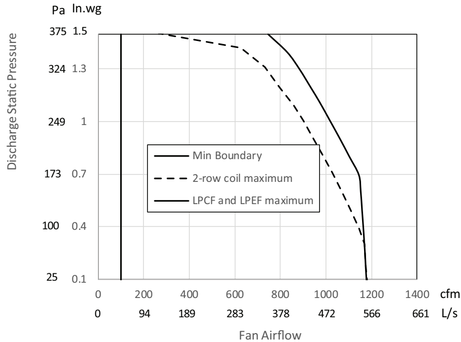
Figure 24. Performance data fan curves, LPxF DS02 — ECM
