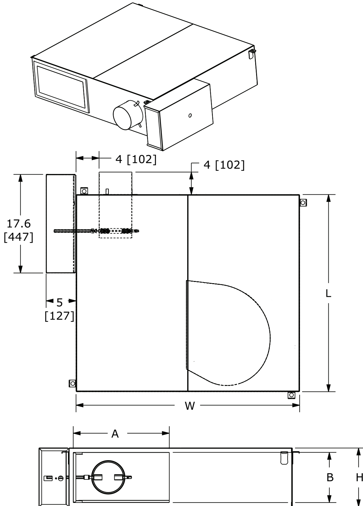
Figure 48. Low-height parallel – cooling only (LPCF)
