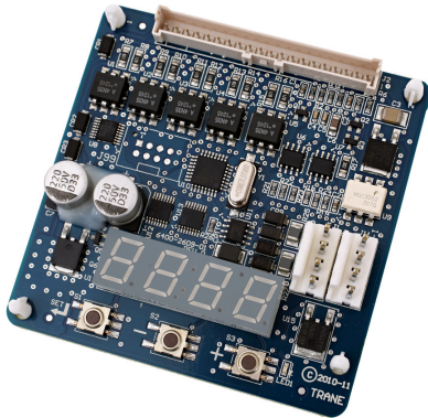
Figure 19. VelociTach motor control board
