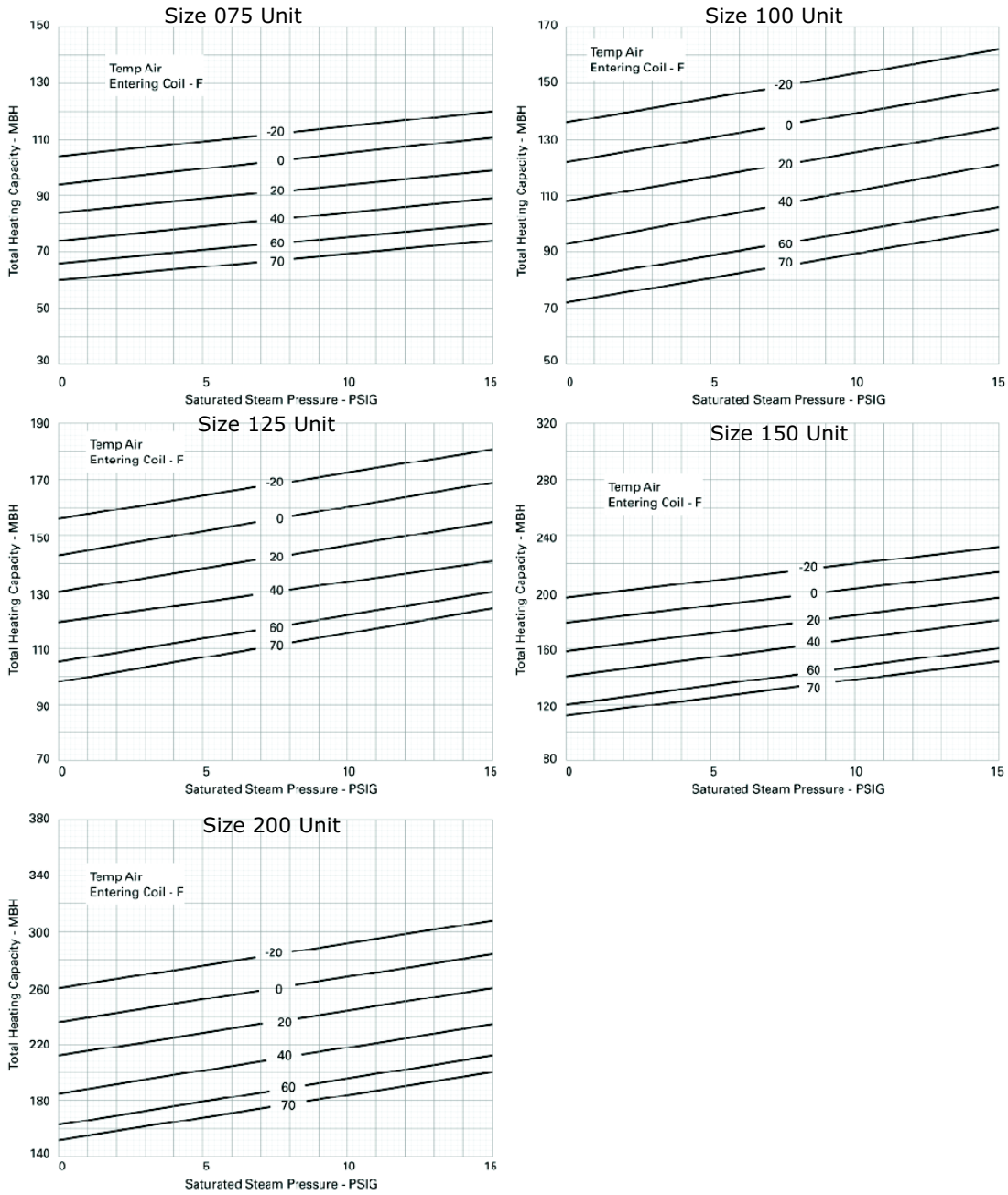
Figure 18. DK, GK Steam coils performance data
