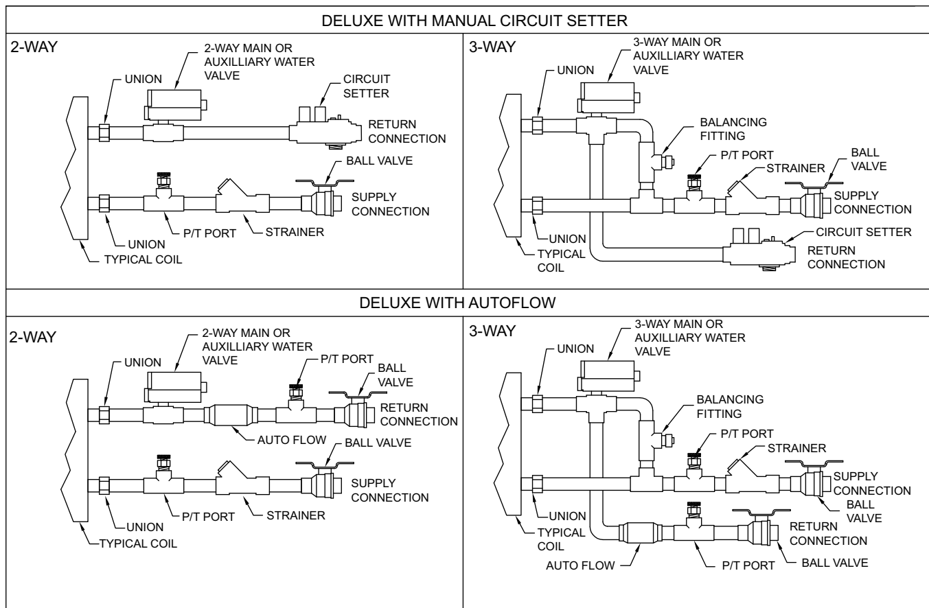
Figure 35. Deluxe piping package
