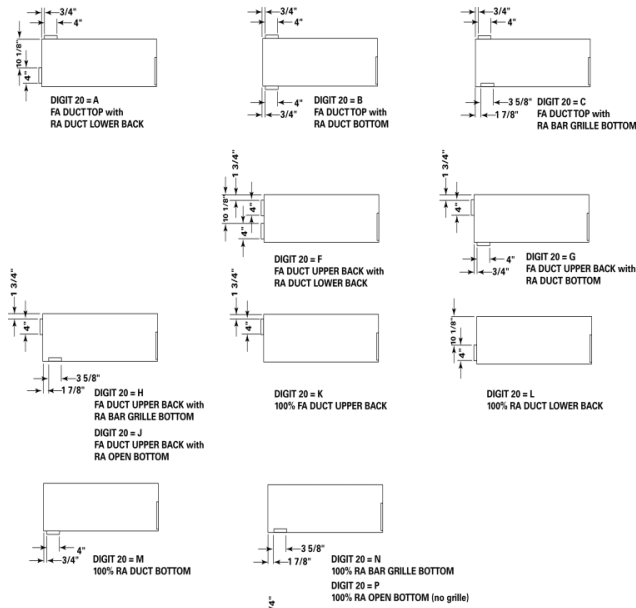
Figure 40. Horizontal unit inlet and discharge arrangements sizes 075-150
