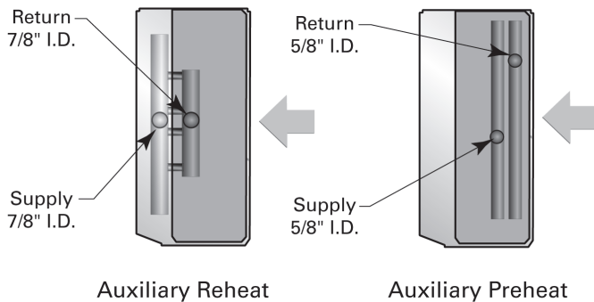
Figure 12. Hydronic auxiliary coil
