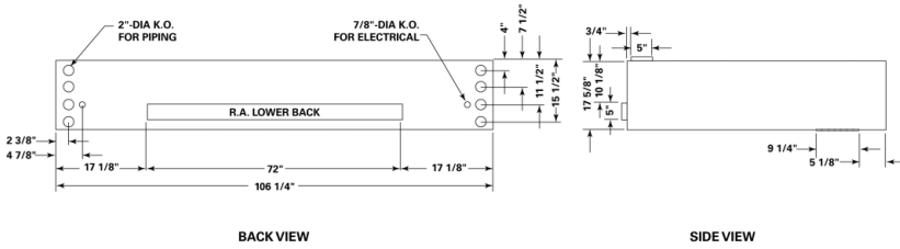
Figure 39. Horizontal unit size 200 with bottom double deflection discharge
