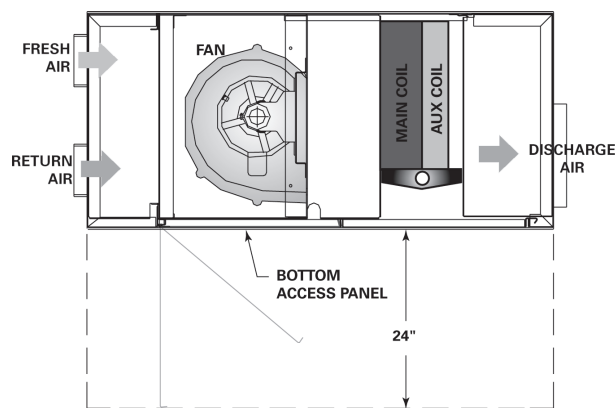
Figure 2. Cabinet access
