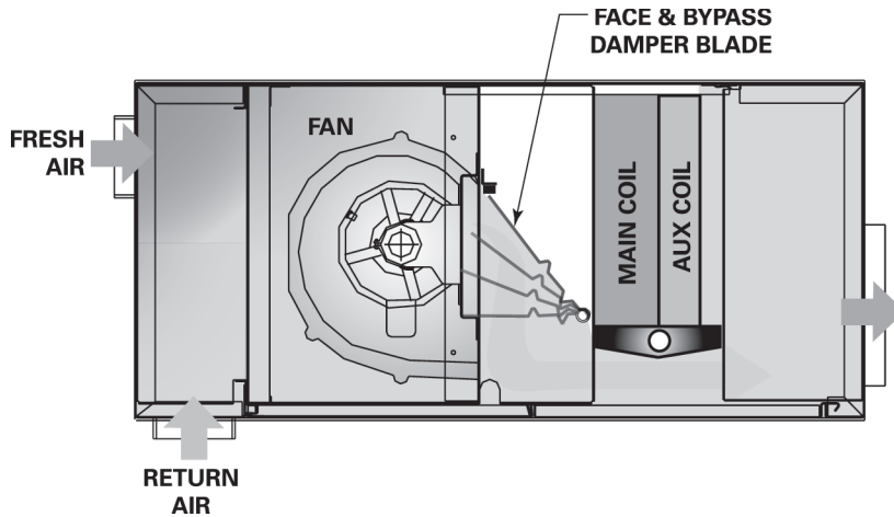
Figure 3. Face-and-bypass damper
