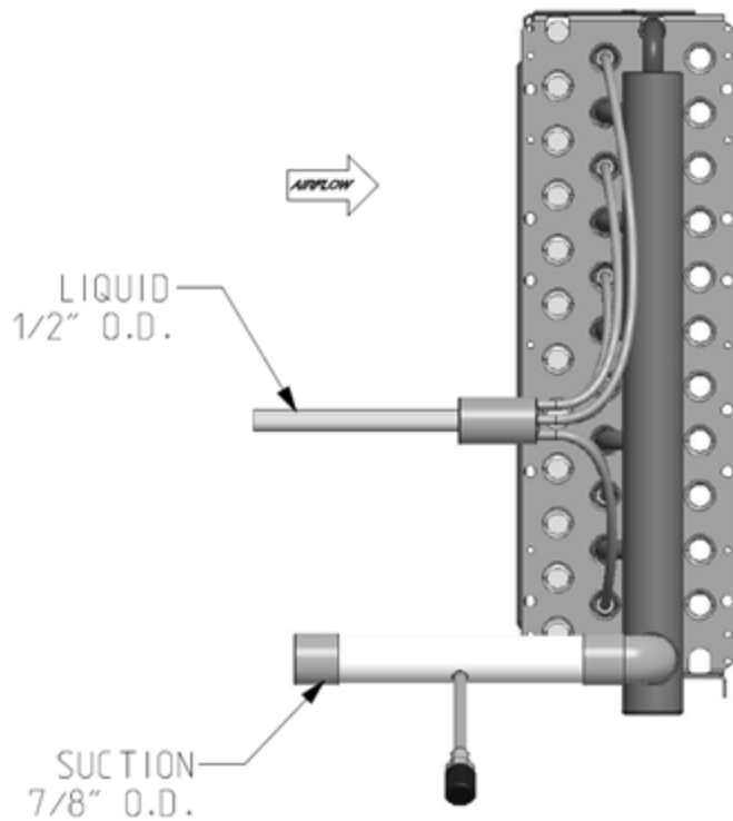
Figure 17. HUV VRF coil
