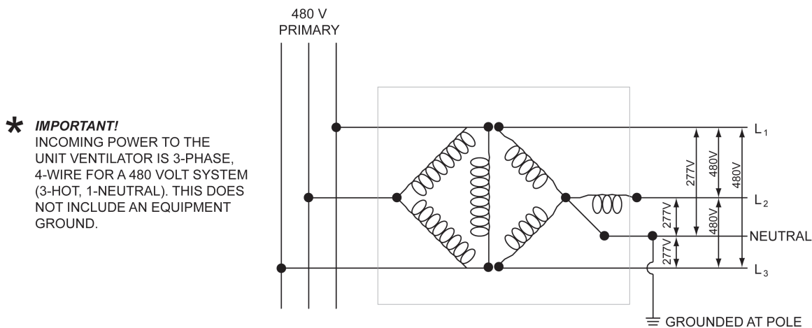
Figure 33. Electric heat
