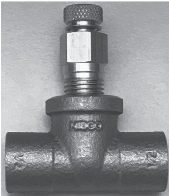
Figure 48. P/T Port
