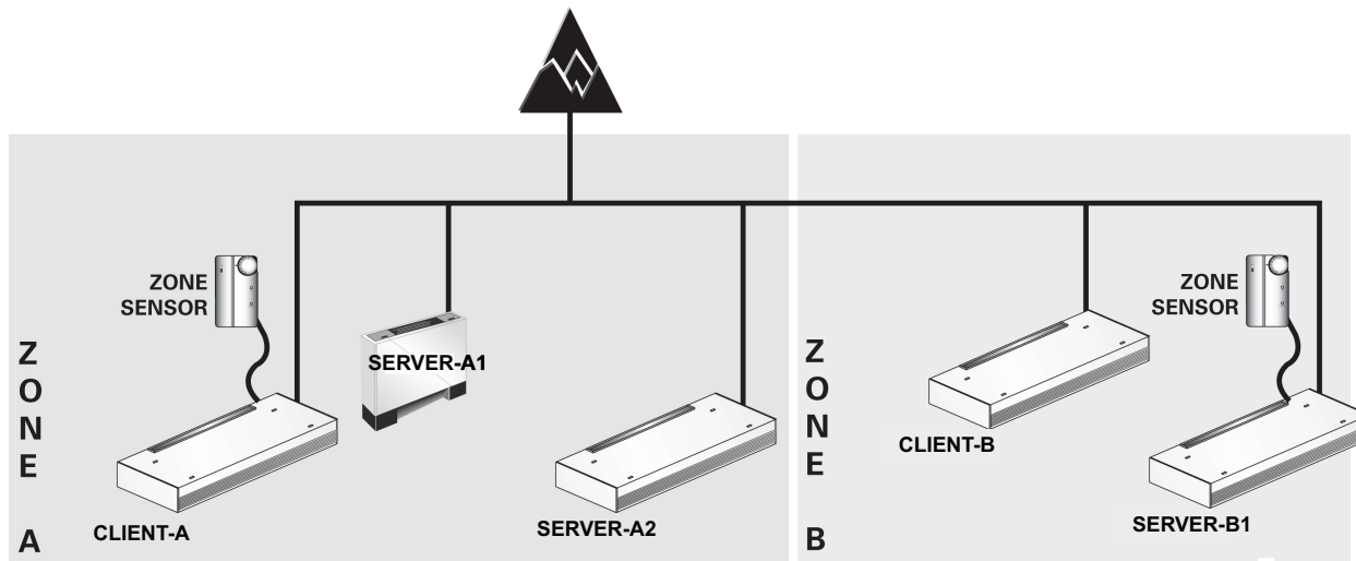
Figure 23. Client server system layout
