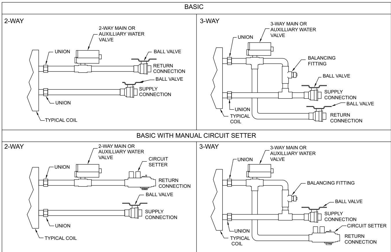
Figure 34. Basic piping package
