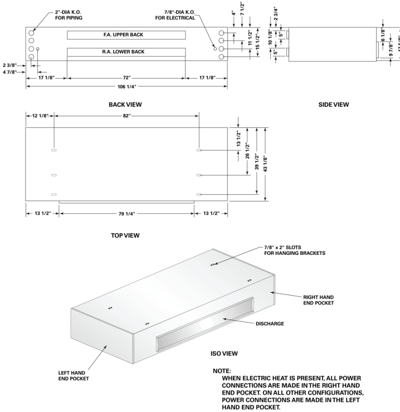
Figure 37. Horizontal unit size 200 with ducted front discharge
