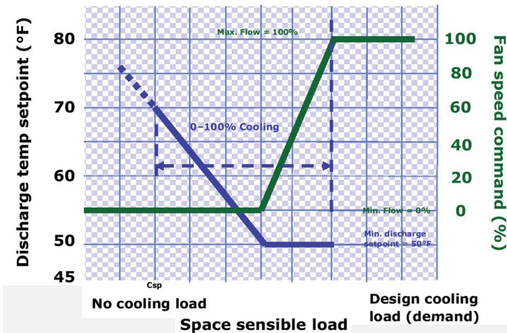
Figure 22. Cool mode nominal hydronic cooling control
