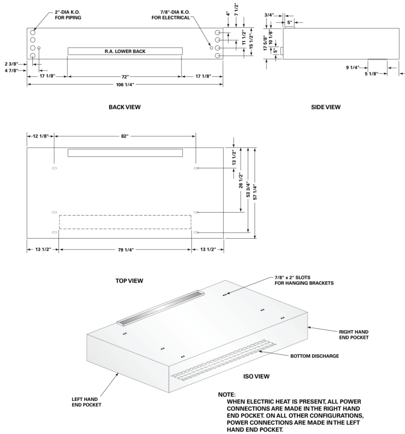
Figure 39. Horizontal unit size 200 with bottom double deflection discharge
