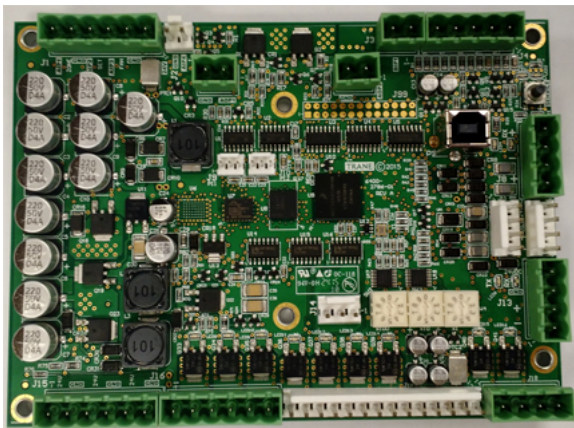
Figure 21. Tracer controller
