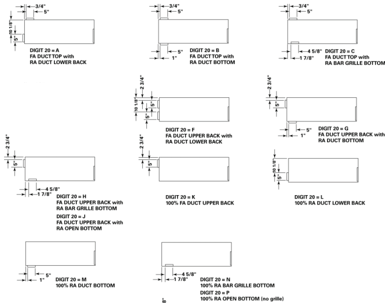
Figure 41. Horizontal unit inlet and discharge arrangements size 200
