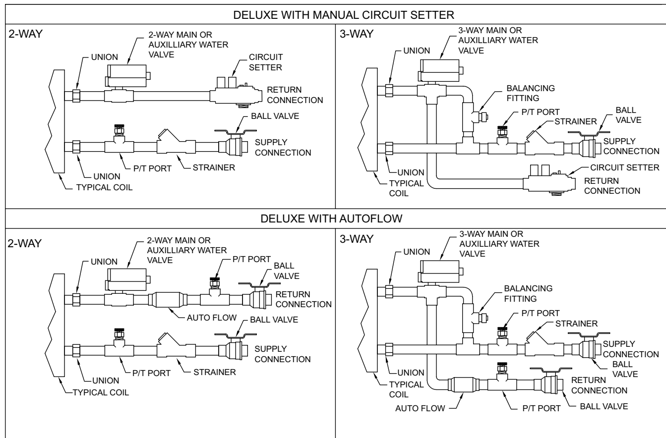
Figure 35. Deluxe piping package
