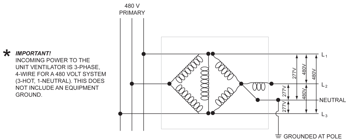
Figure 33. Electric heat
