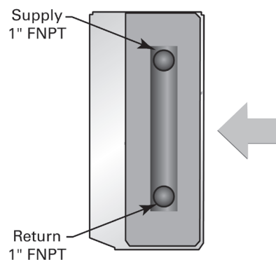
Figure 13. Steam main coil
