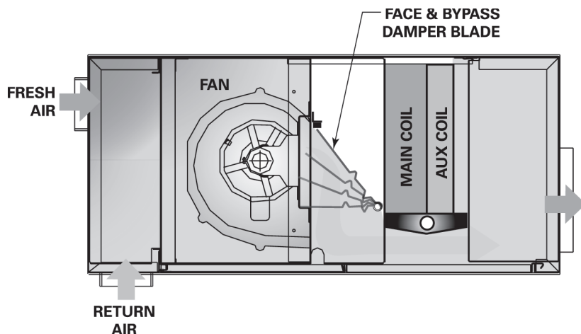
Figure 3. Face-and-bypass damper
