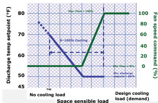
Figure 21. Cool mode nominal hydronic cooling control
