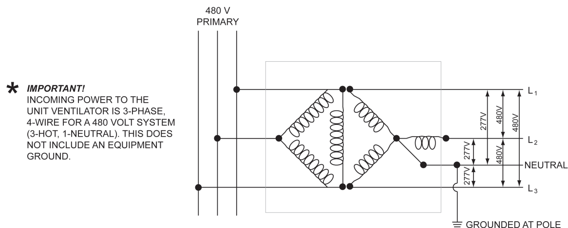
Figure 32. Electric heat
