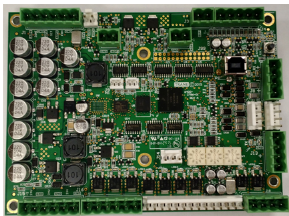
Figure 20. Tracer controller
