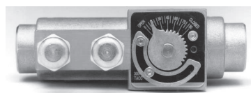
Figure 45. Manual circuit setter
