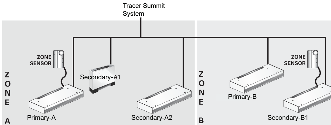
Figure 25. Data sharing system layout
