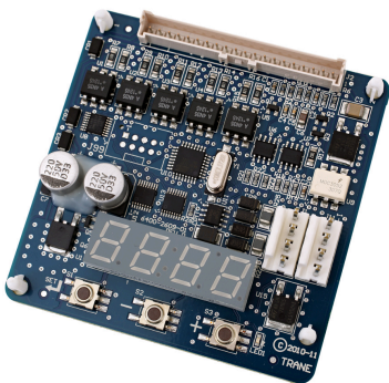
Figure 20. VelociTach motor control board
