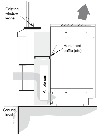
Figure 17. Step-down falseback unit
