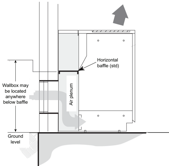
Figure 16. Falseback unit
