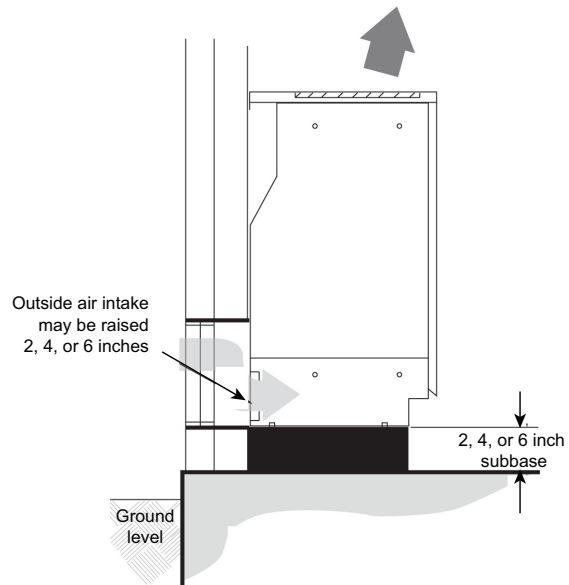
Figure 19. Subbase
