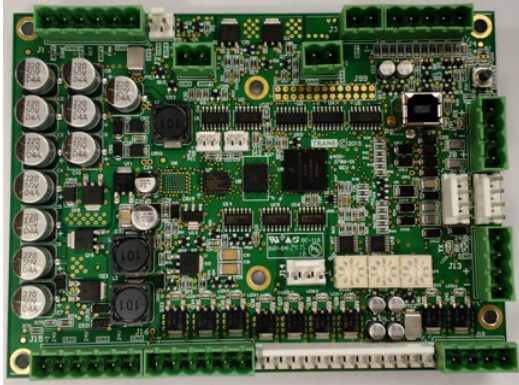
Figure 23. Tracer® Symbio 400-B controller
