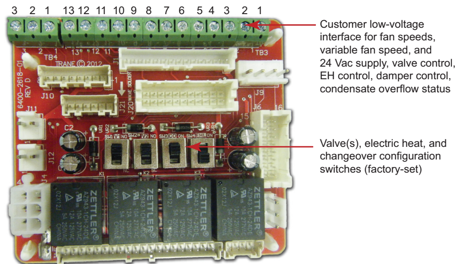
Figure 22. CSTI adapter board and field connections
