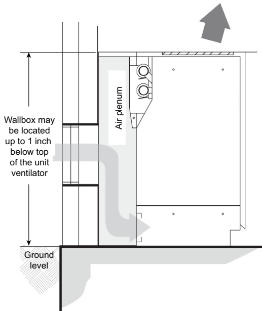
Figure 18. Insulated falseback with raised OA opening
