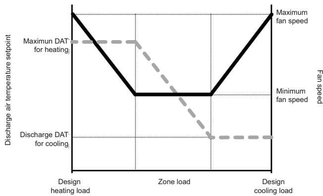
Figure 24. Single-zone VAV control
