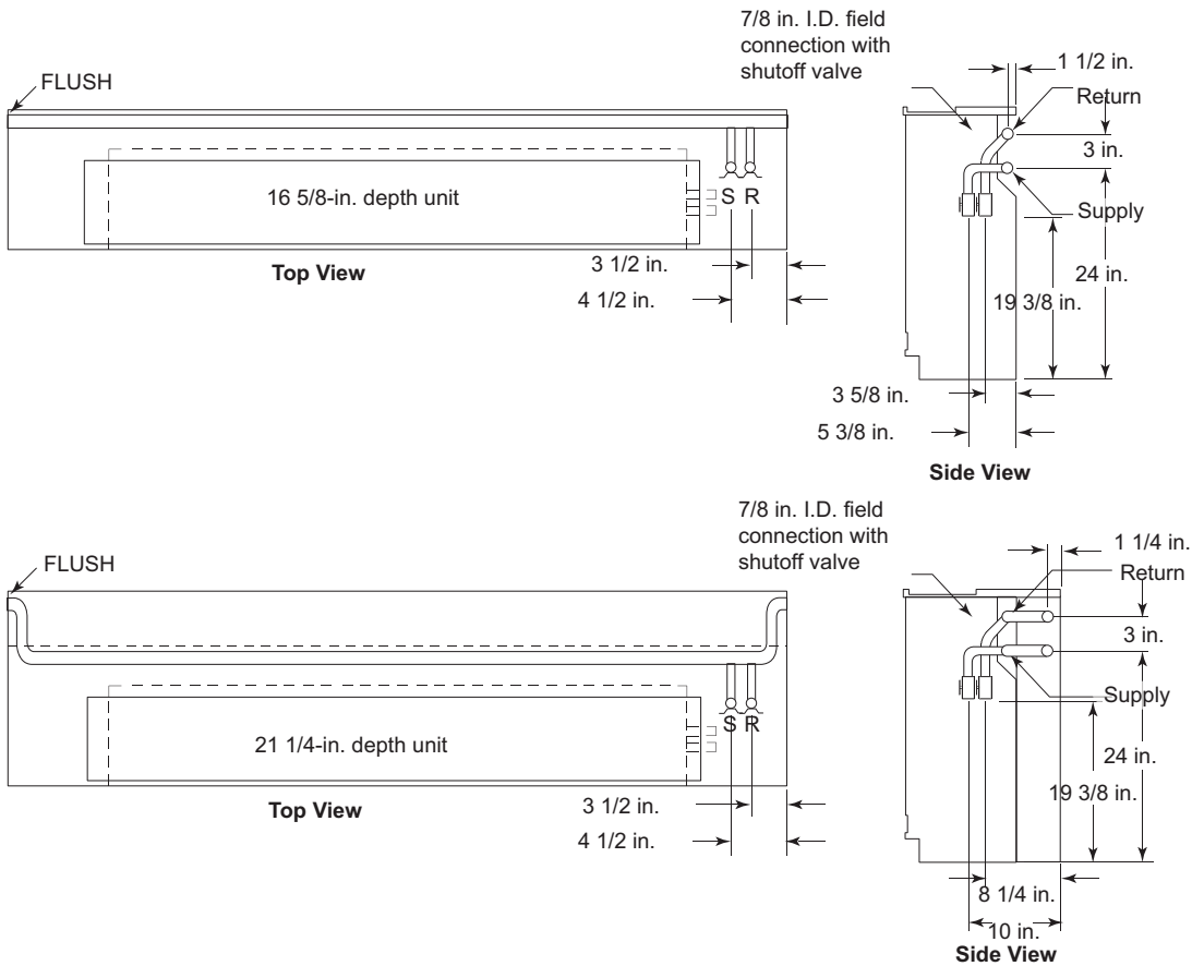
Figure 43. Crossover piping dimensions (inches)
