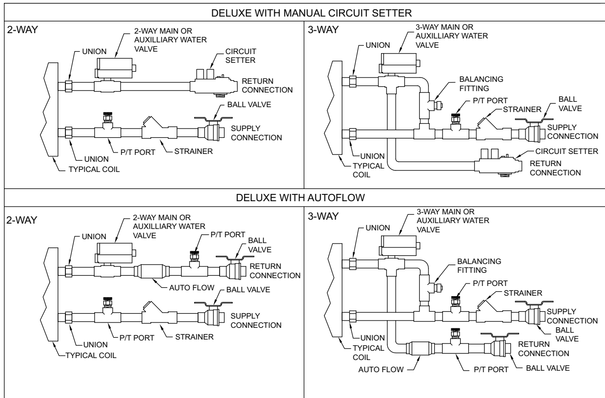
Figure 35. Deluxe piping package
