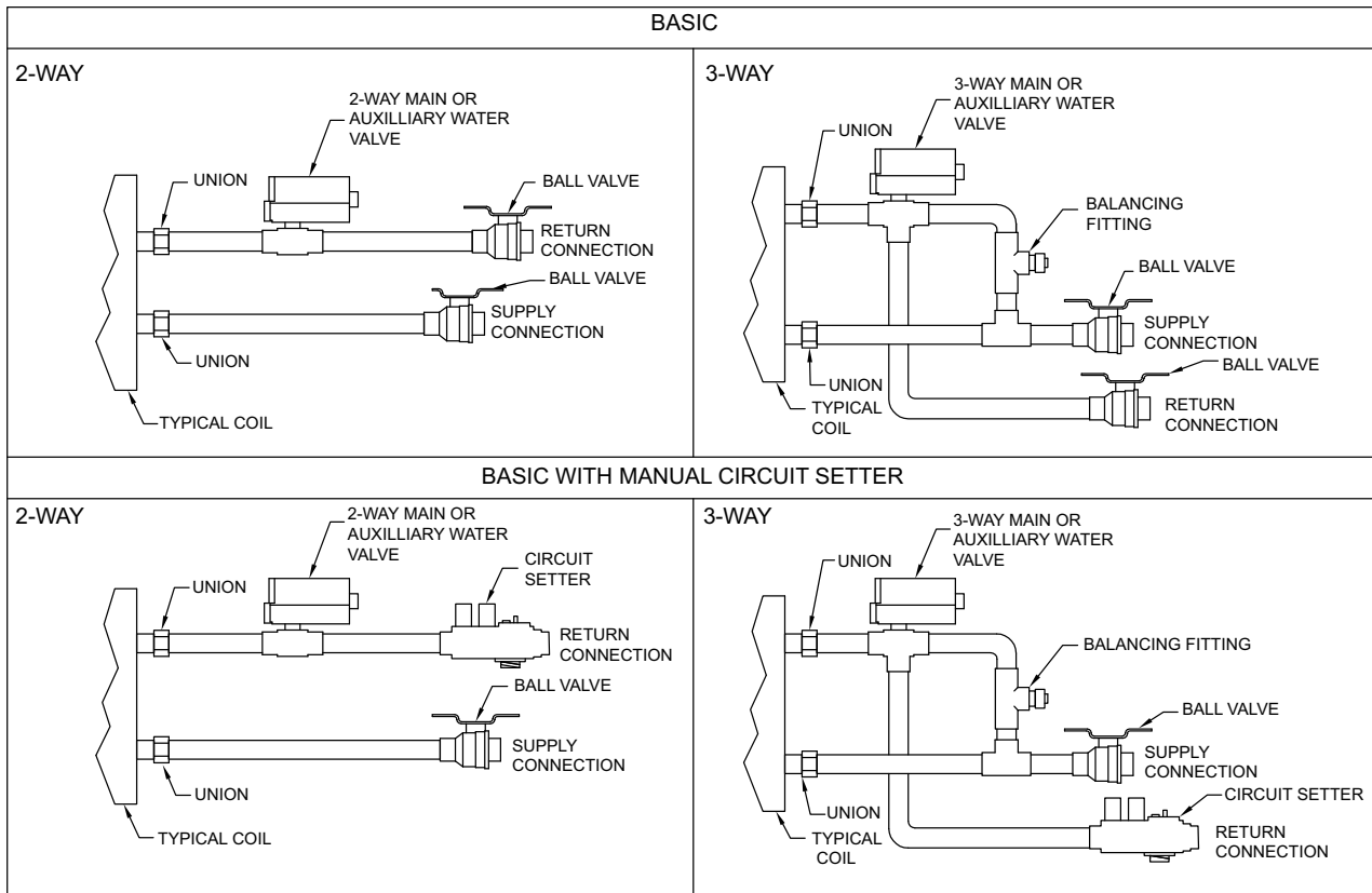
Figure 34. Basic piping package
