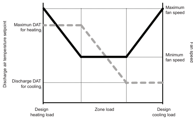
Figure 23. Single-zone VAV control
