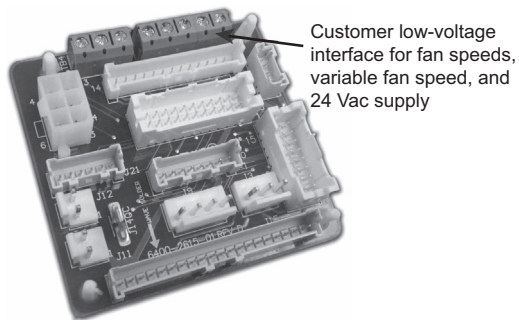
Figure 4. Standard adapter board
