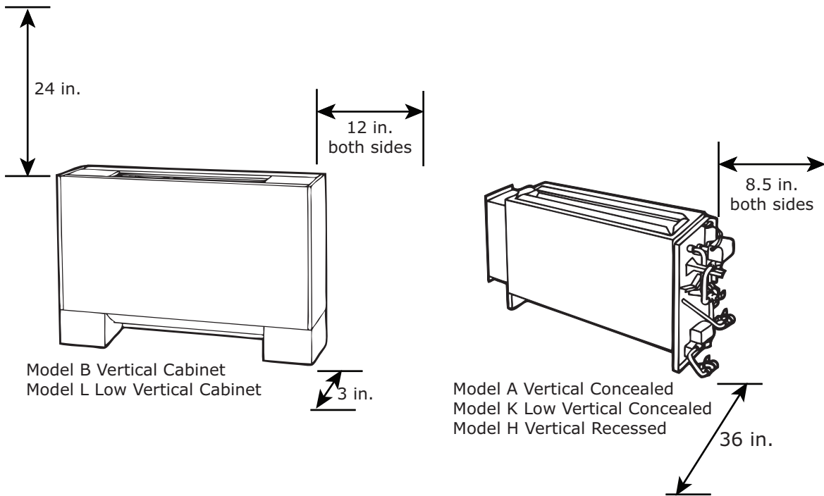
Figure 31. Recommended service clearances for vertical units
