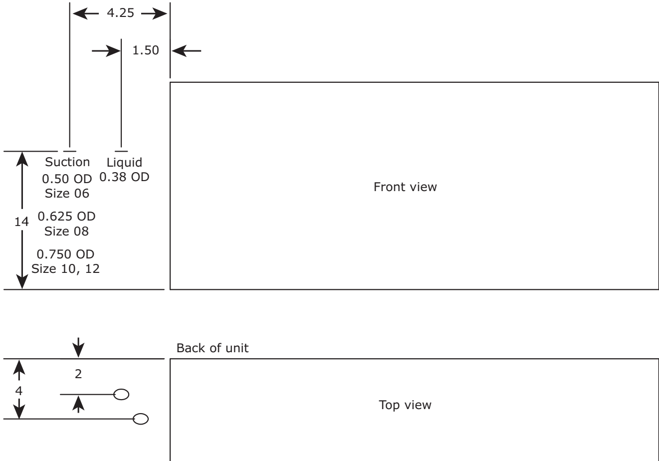
Figure 45. Coil connections for DX coil and heat pump
