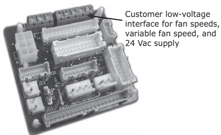
Figure 14. Standard adapter board
