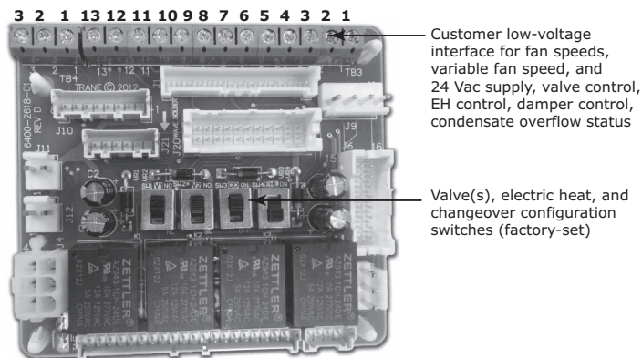
Figure 15. CSTI adapter board and field connections
