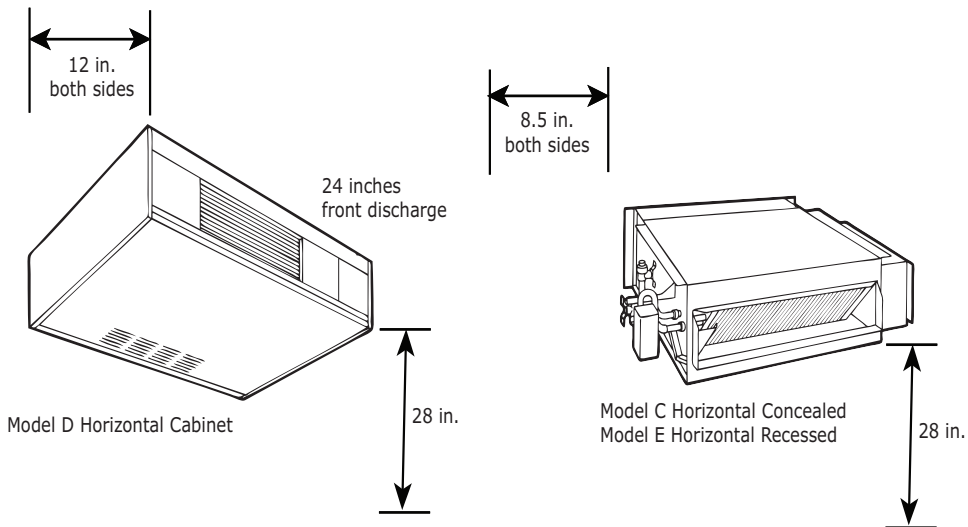
Figure 32. Recommended service clearances for horizontal units
