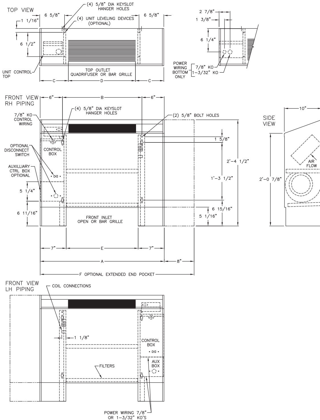
Figure 39. Model J vertical slope top
