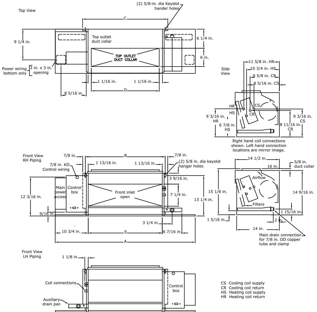
Figure 40. Model K low vertical concealed
