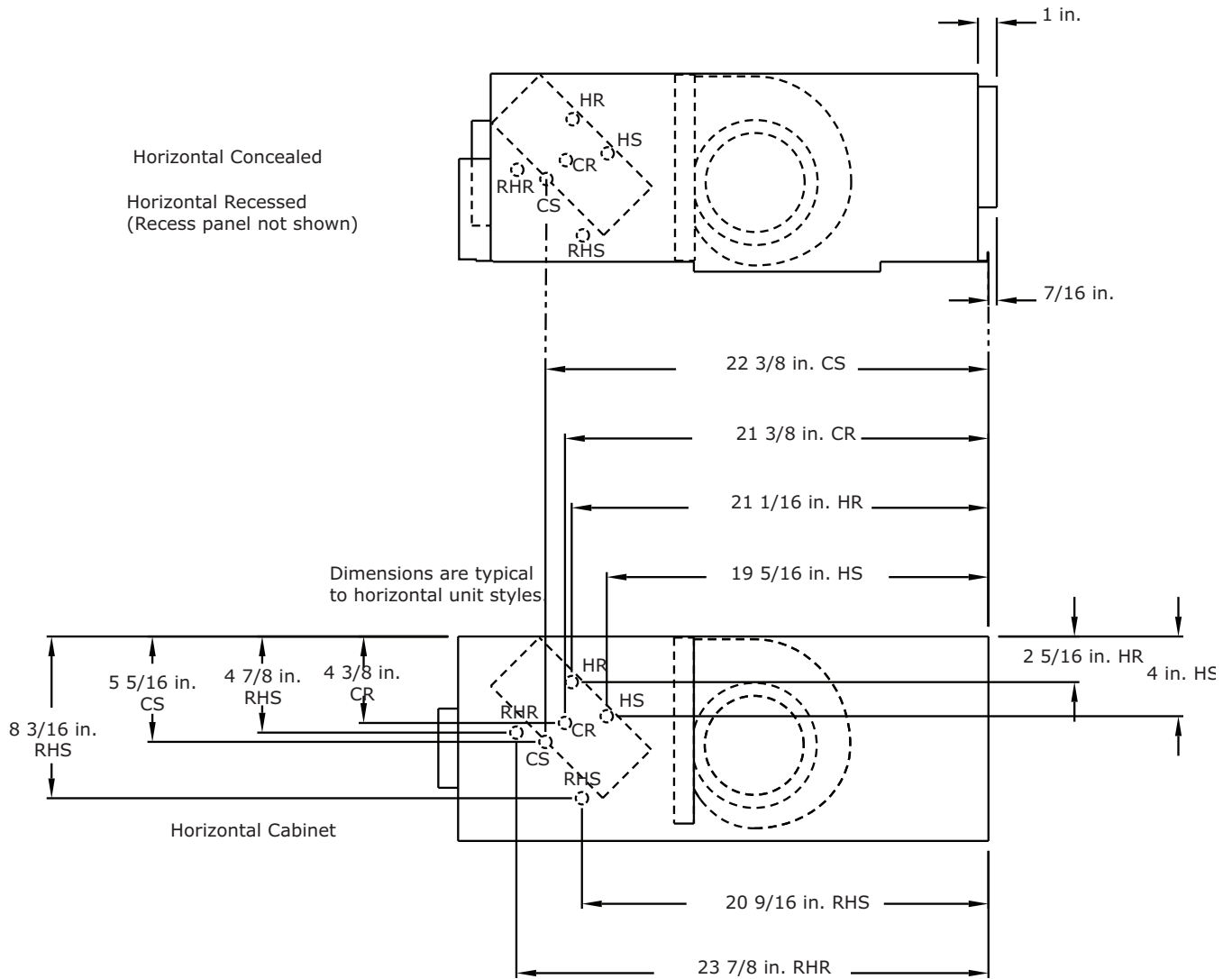
Figure 44. Coil connections for fan coil horizontal units
