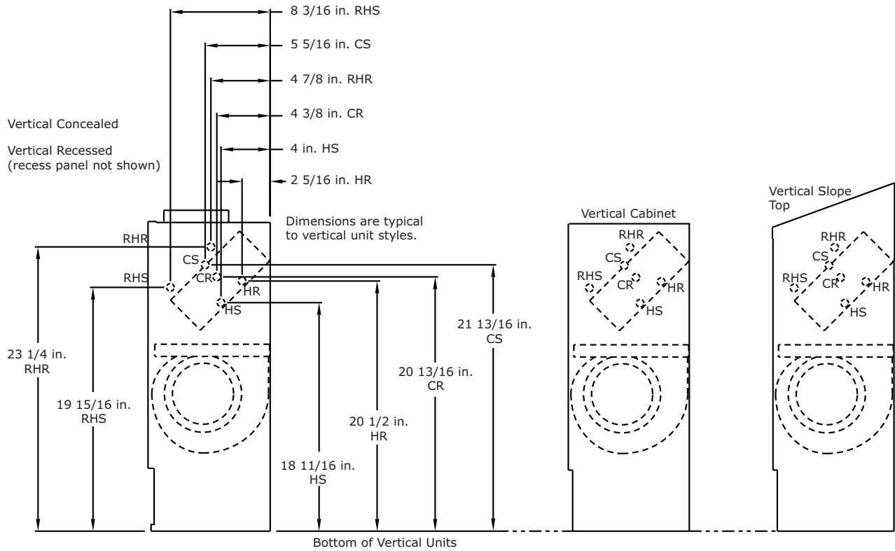
Figure 43. Coil connections for fan coil vertical units
