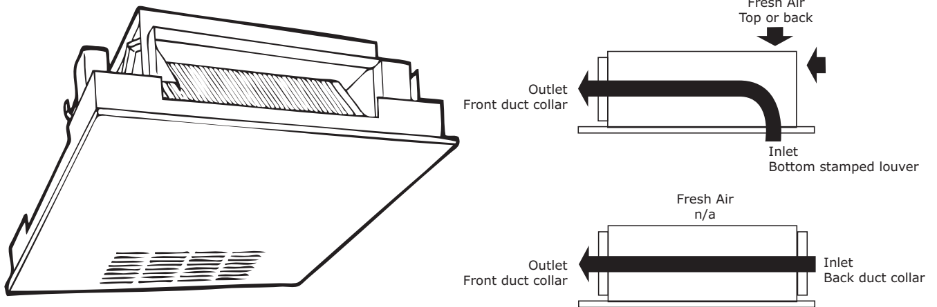
Figure 7. Model E airflow options
