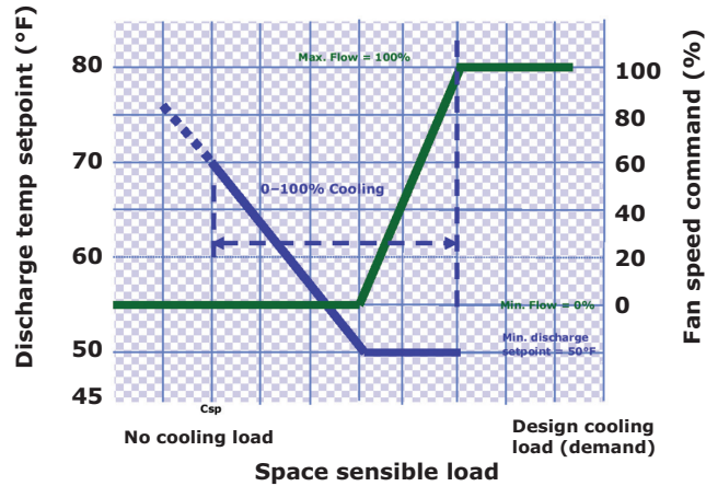
Figure 17. Cool mode nominal hydronic cooling control
