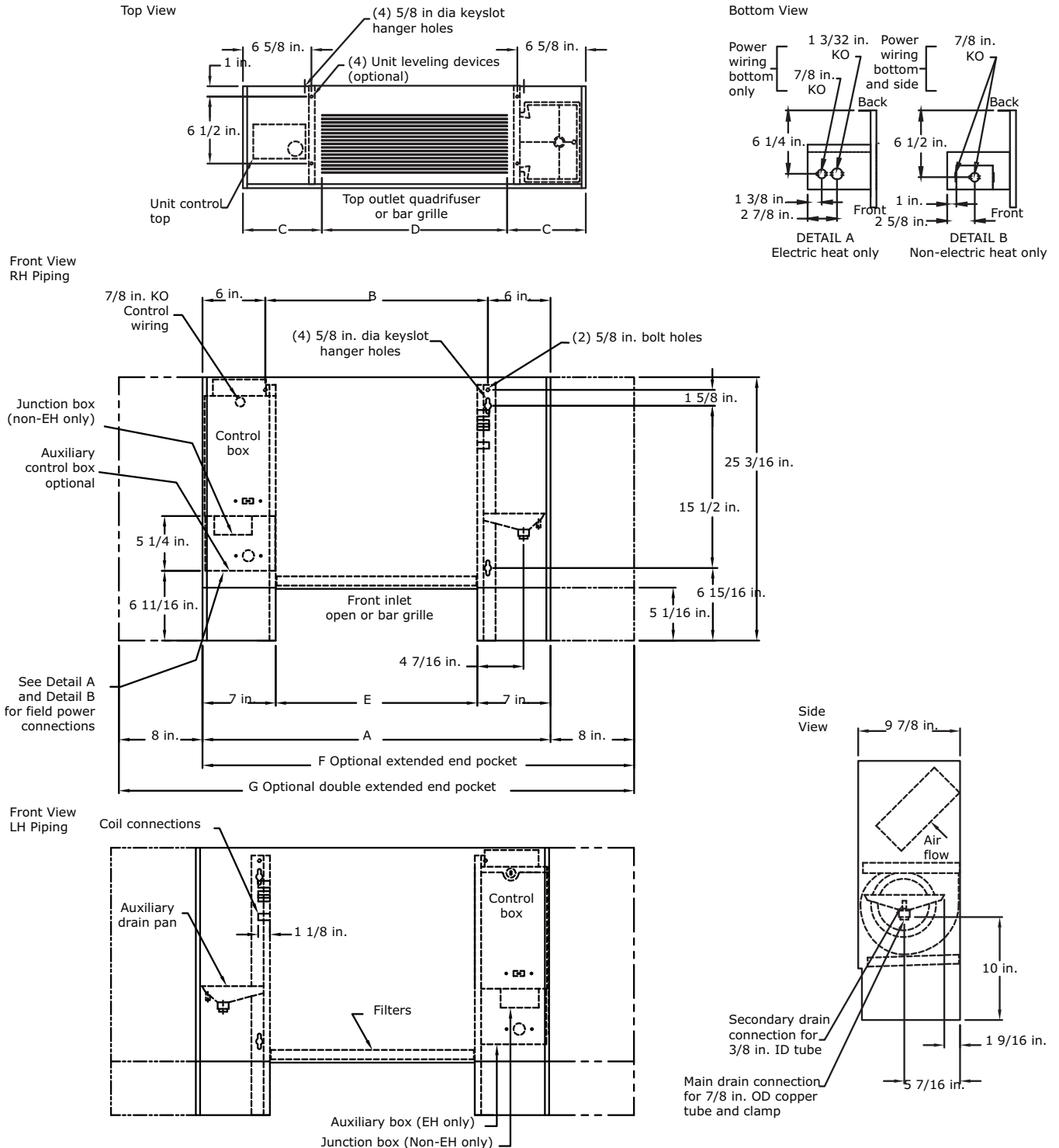
Figure 34. Model B vertical cabinet
