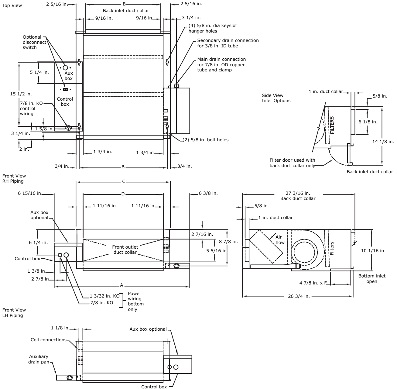
Figure 35. Model C Horizontal concealed unit
