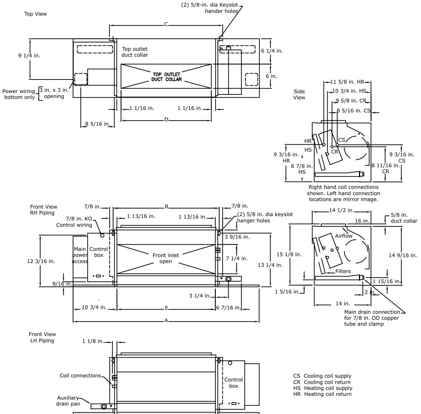
Figure 41. Model L low vertical cabinet
