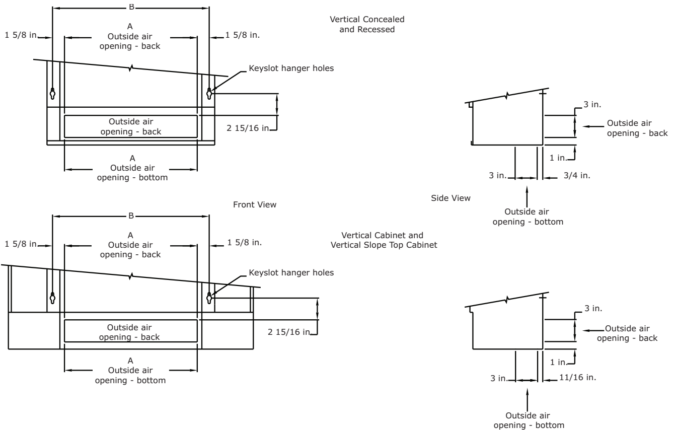
Figure 48. Fresh air openings for vertical units (models A, B, H, J, K, and L)
