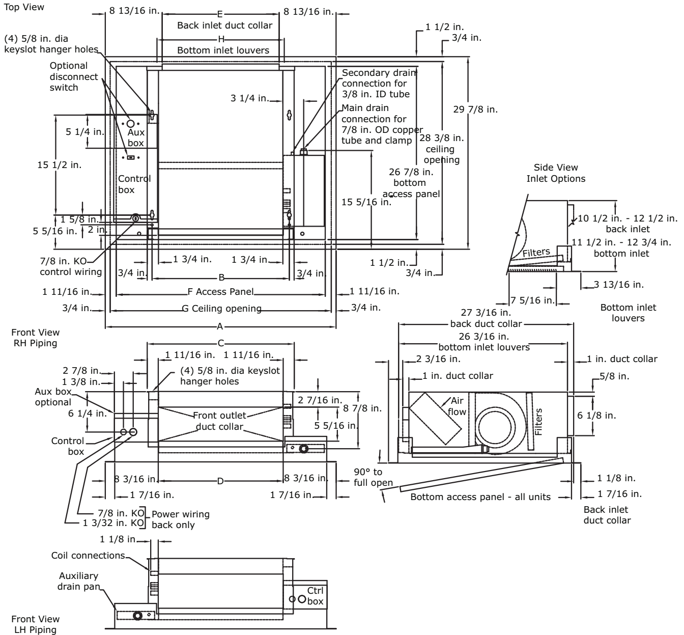
Figure 37. Model E horizontal recessed
