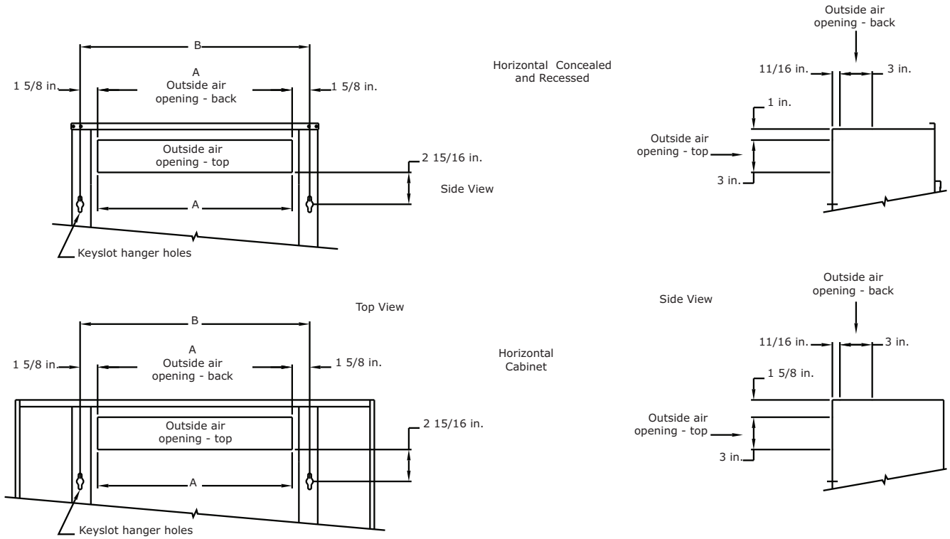
Figure 47. Fresh air openings for horizontal units (models C, D, E, and P (back duct collar only))
