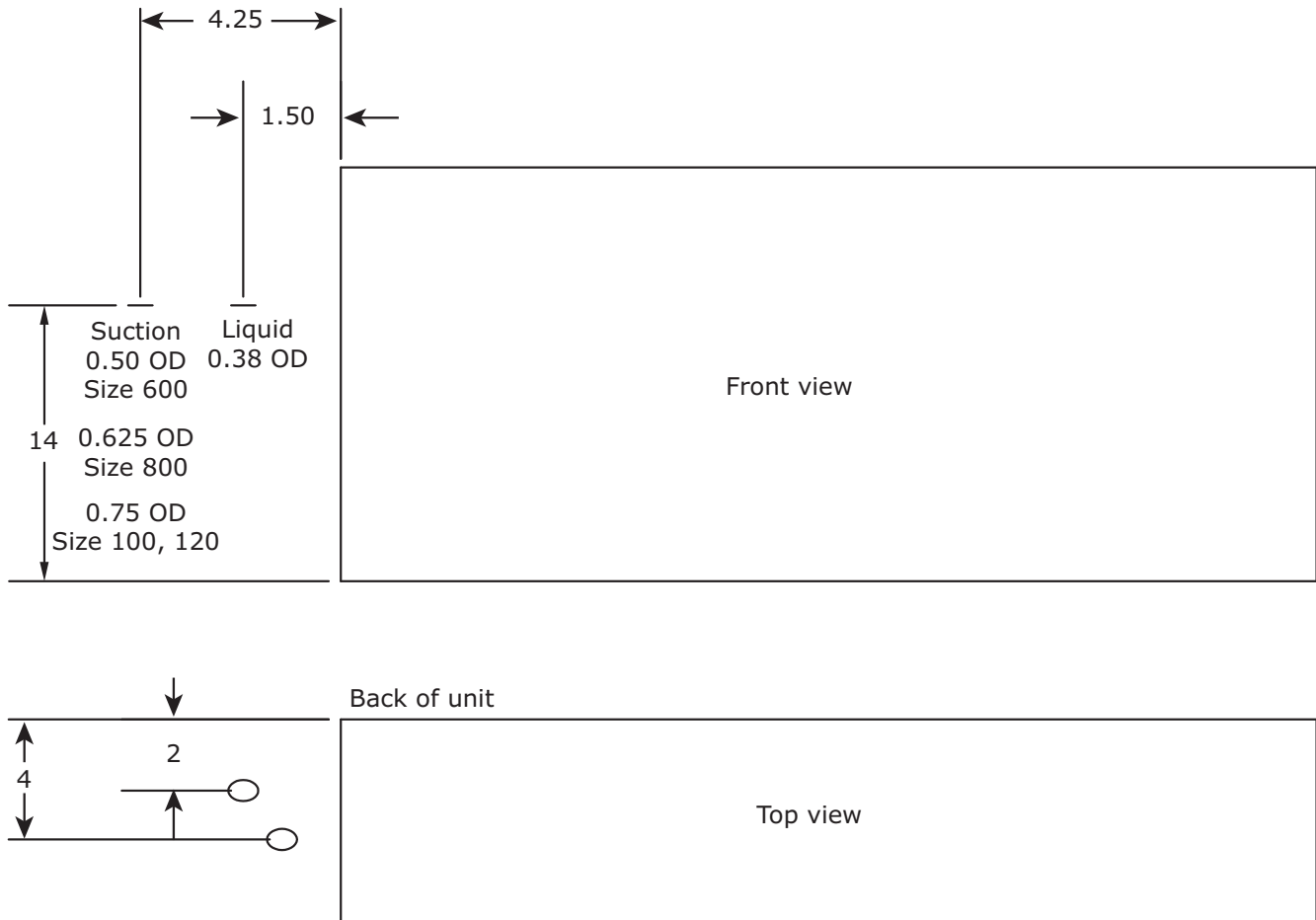
Figure 46. DX and heat pump connections
