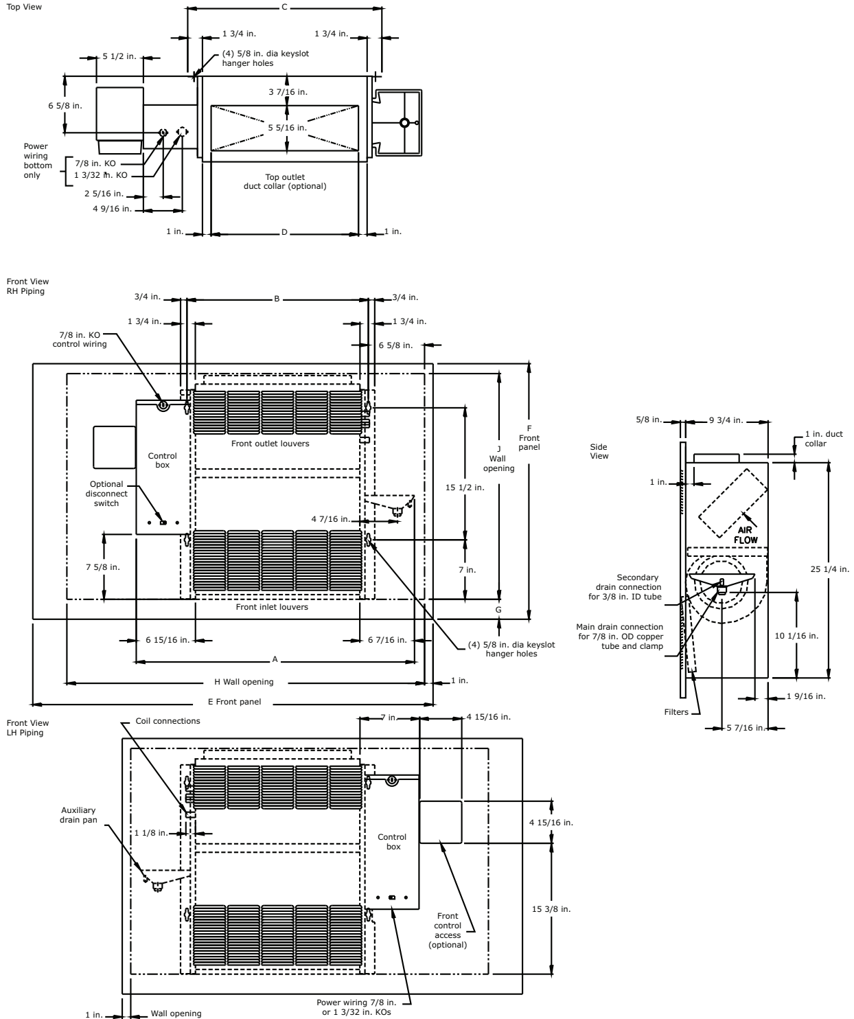
Figure 38. Model H vertical recessed
