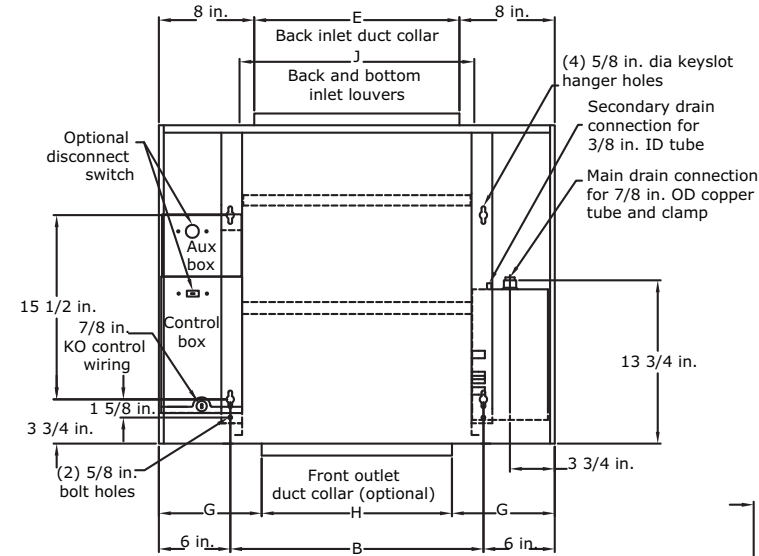
Figure 36. Model D horizontal cabinet
