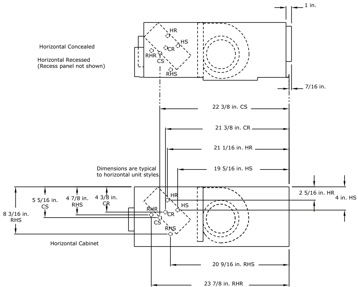
Figure 43. Coil connections for fan coil horizontal units
