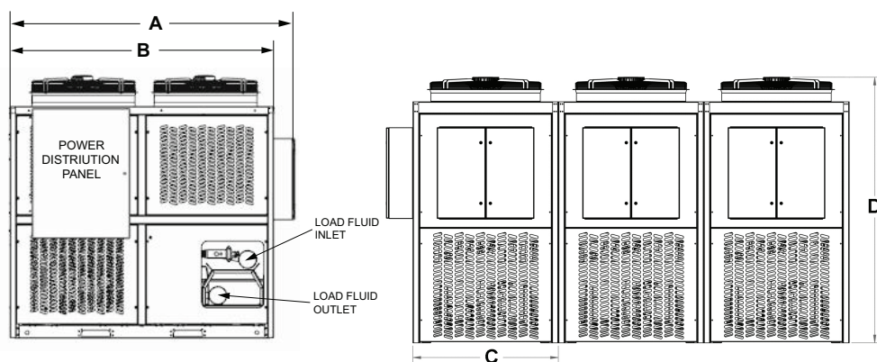
Figure 6. AXM air-to-water heat pump 30 tons
