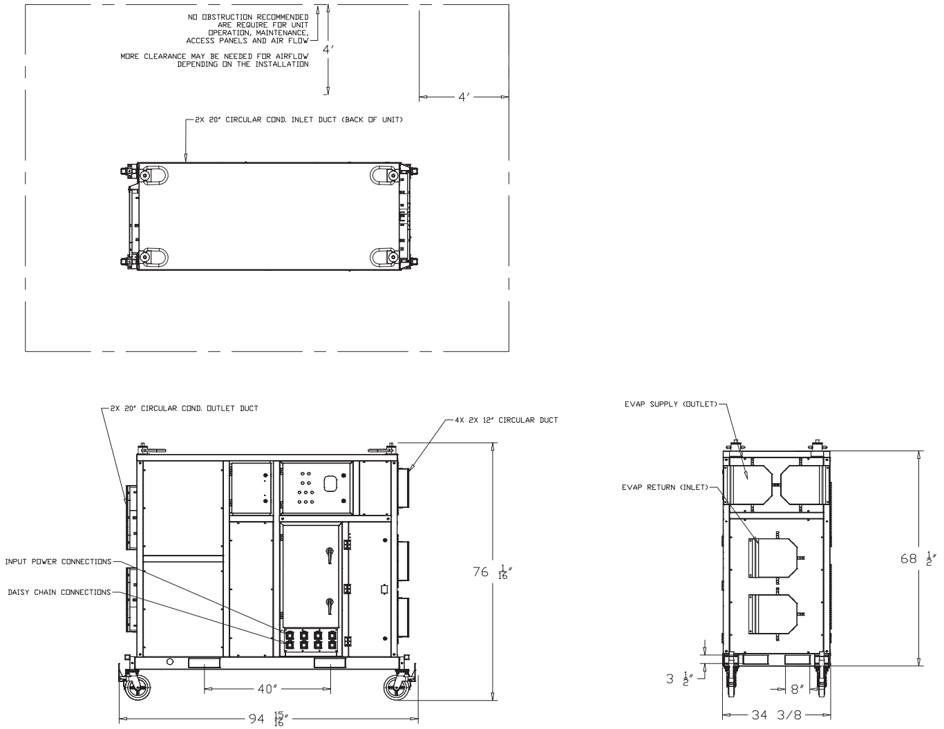
Figure 8. Unit drawing — RSDX0012F2AE-HV
