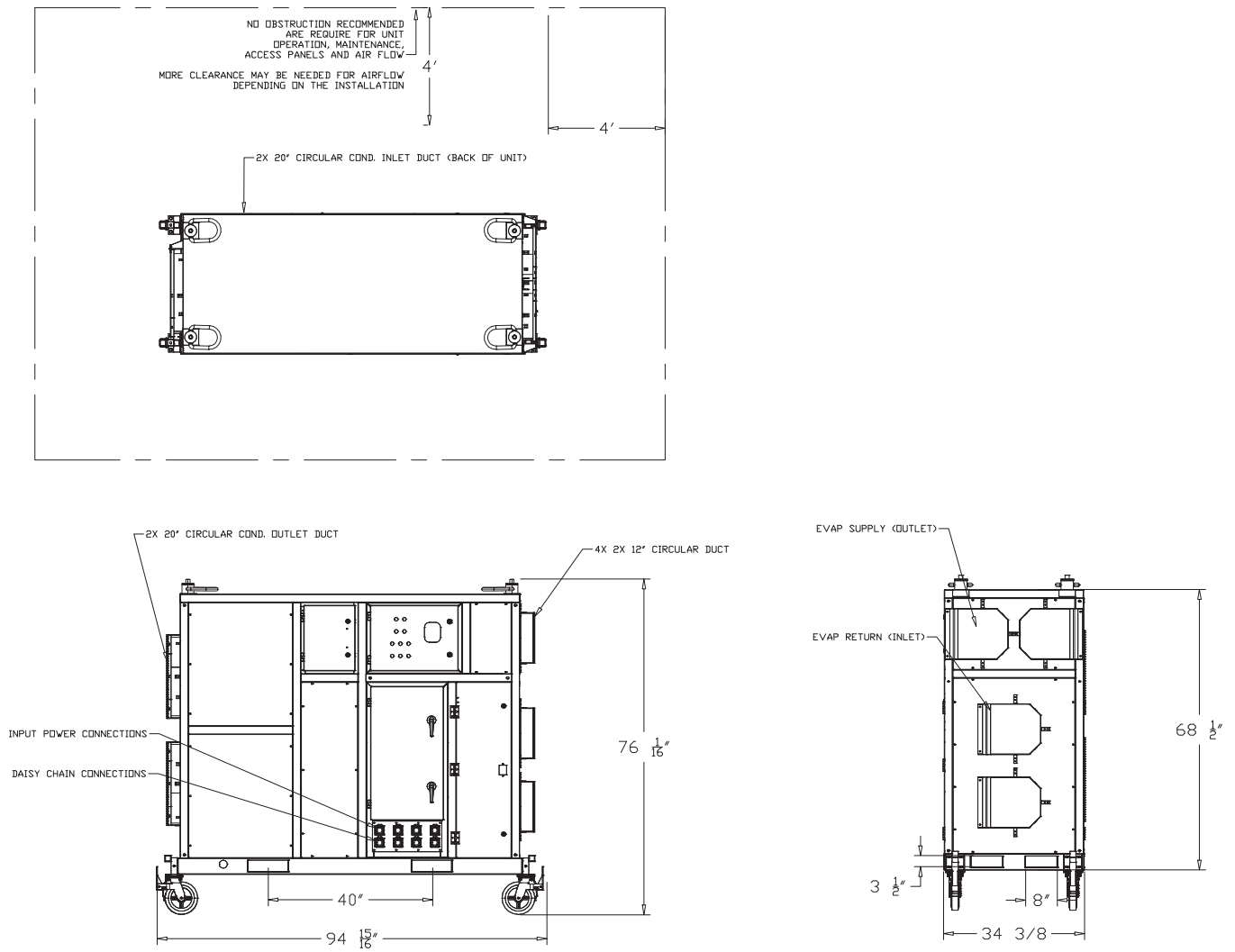
Figure 11. Unit drawing — RSDX0012D2AA-BD
