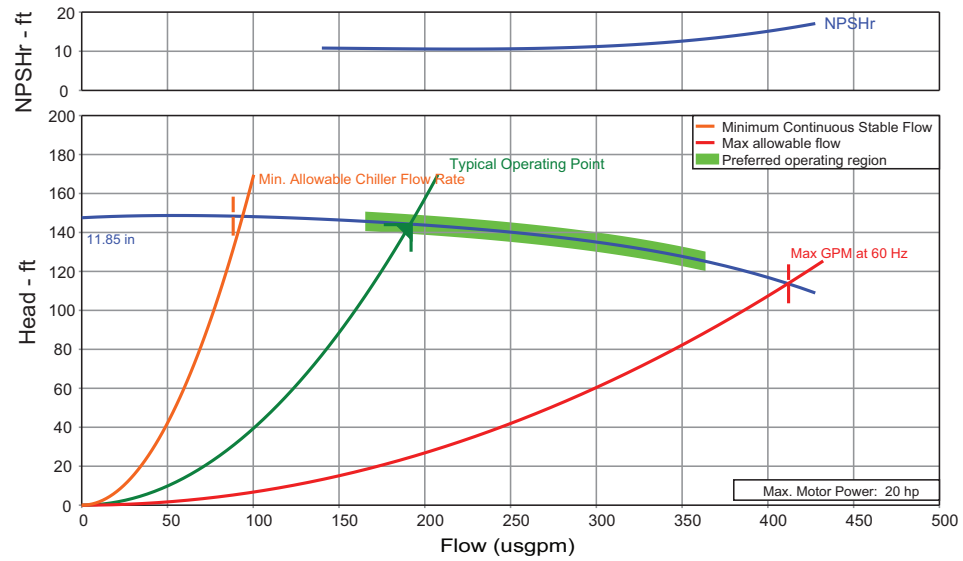
Single Speed Pump Curve
