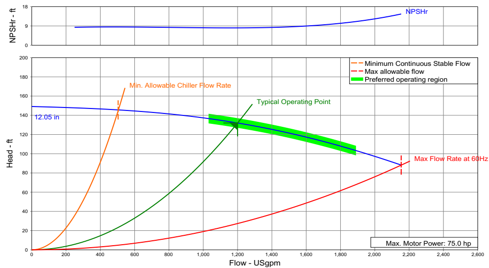
Figure 7. Multi Speed Pump Curve
