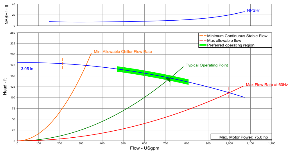
Figure 3. Multi Speed Pump Curve
