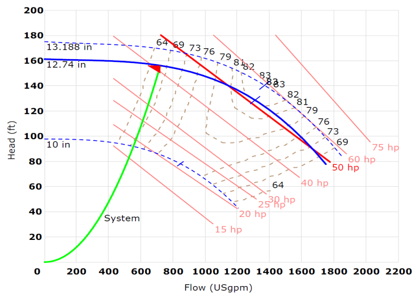
Figure 4. Single pump curve
