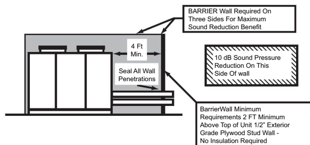
Figure 1. Minimum wall requirements
