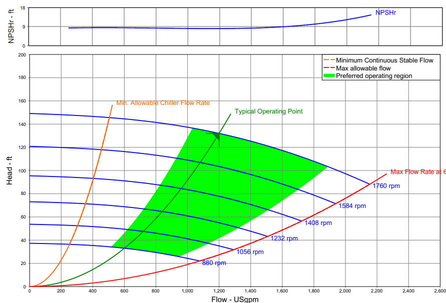
Figure 7. Multi Speed Pump Curve
