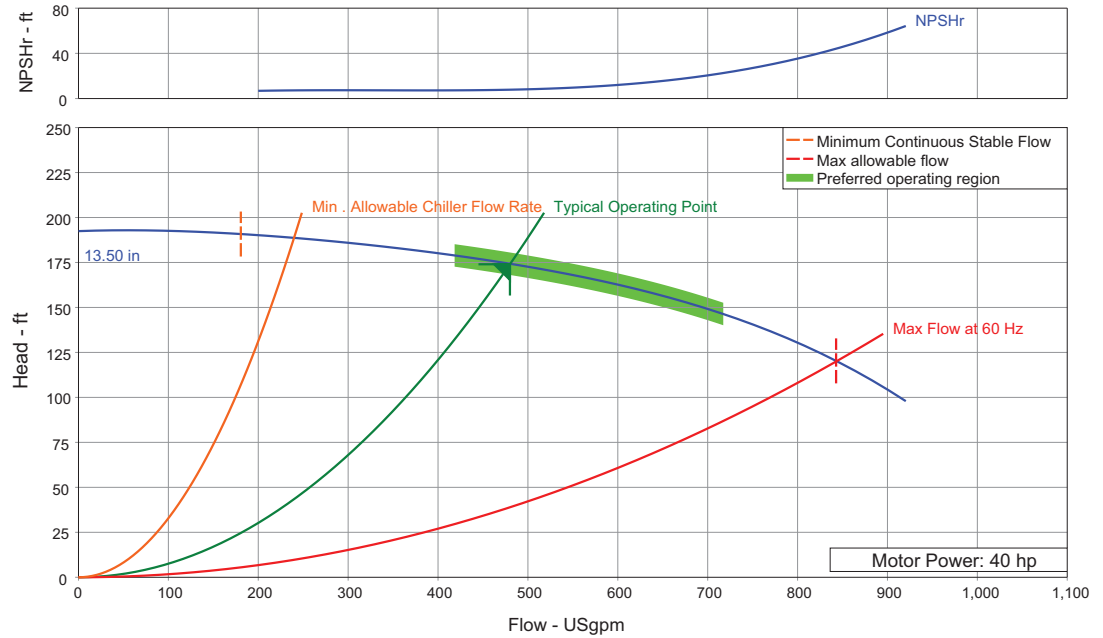
Single Speed Pump Curve
