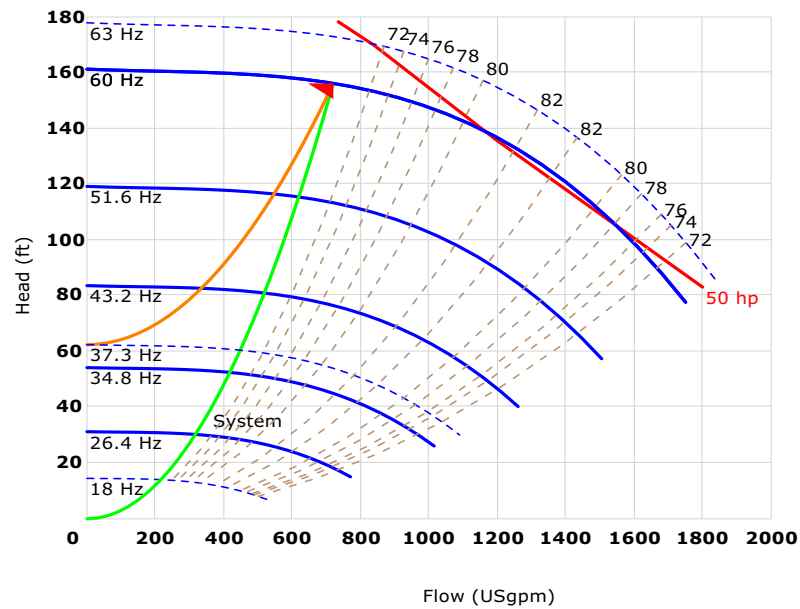
Figure 5. Multi-speed pump curve
