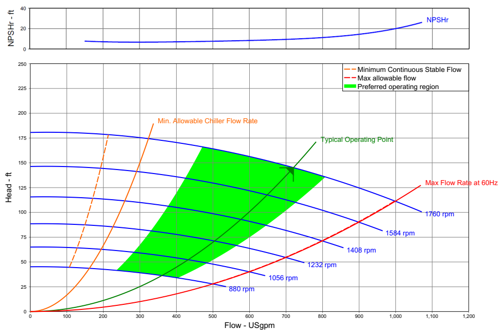
Figure 3. Multi Speed Pump Curve
