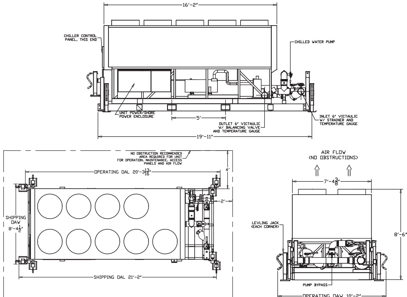
Figure 61. Unit drawings
