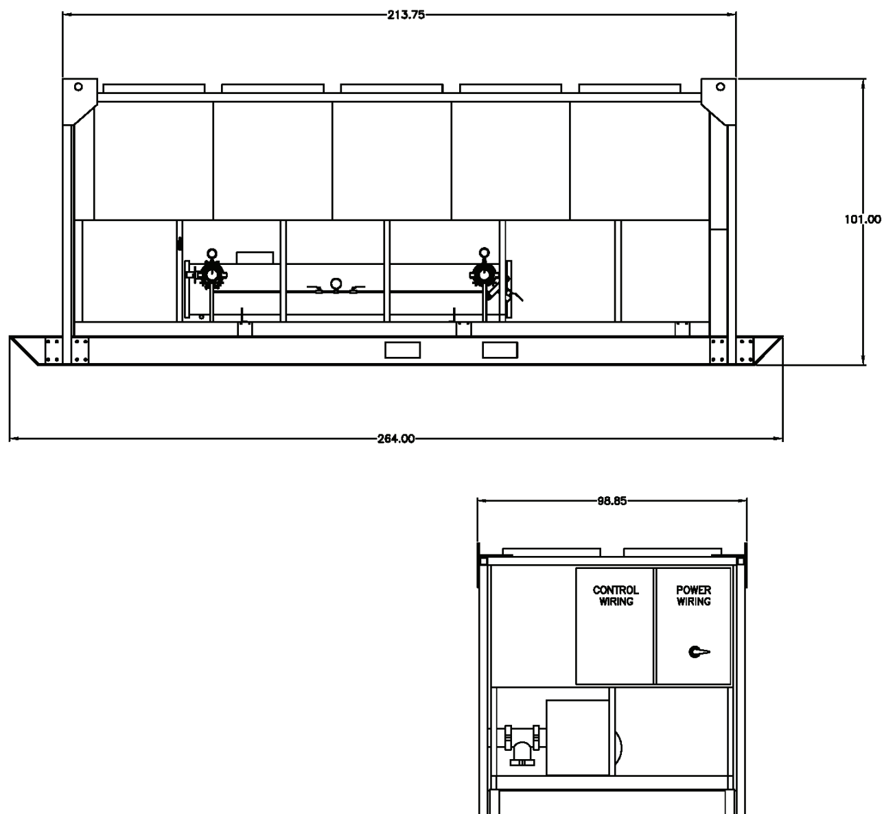
Figure 55. Unit drawings
