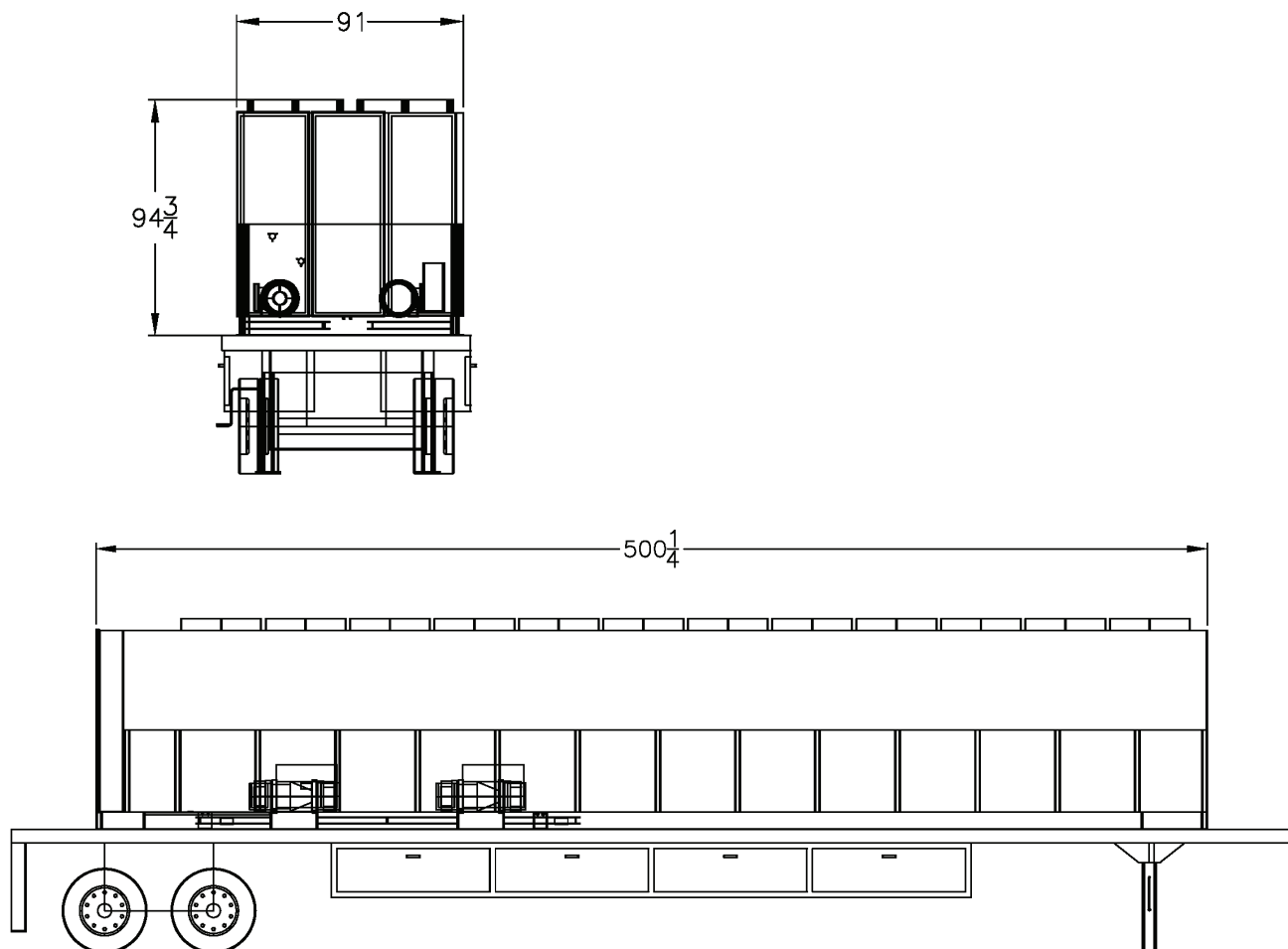
Figure 91. Unit drawings
