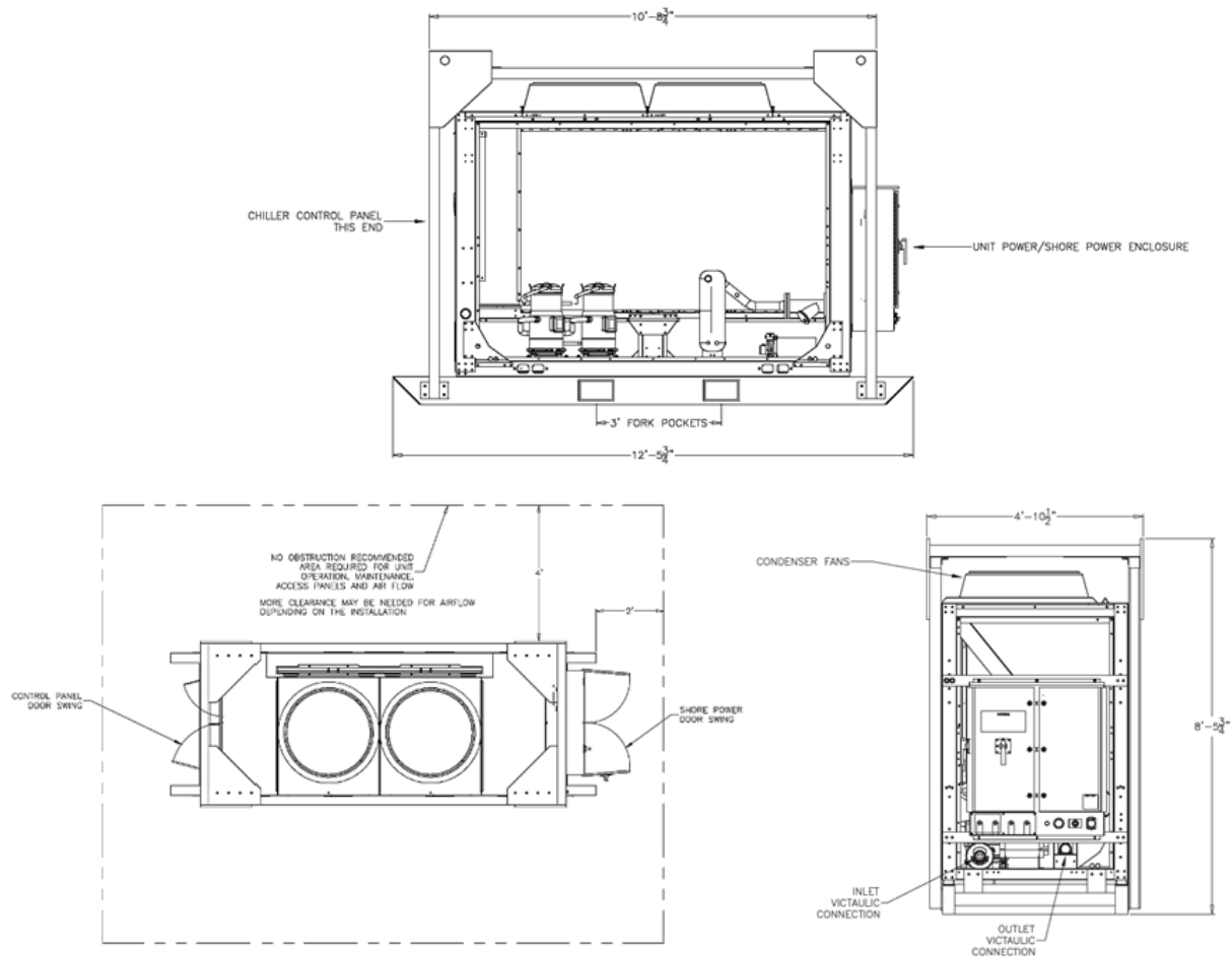
Figure 11. Unit drawings
