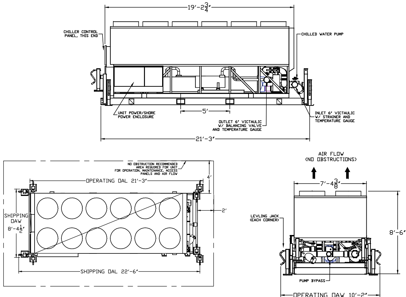
Figure 73. Unit drawings
