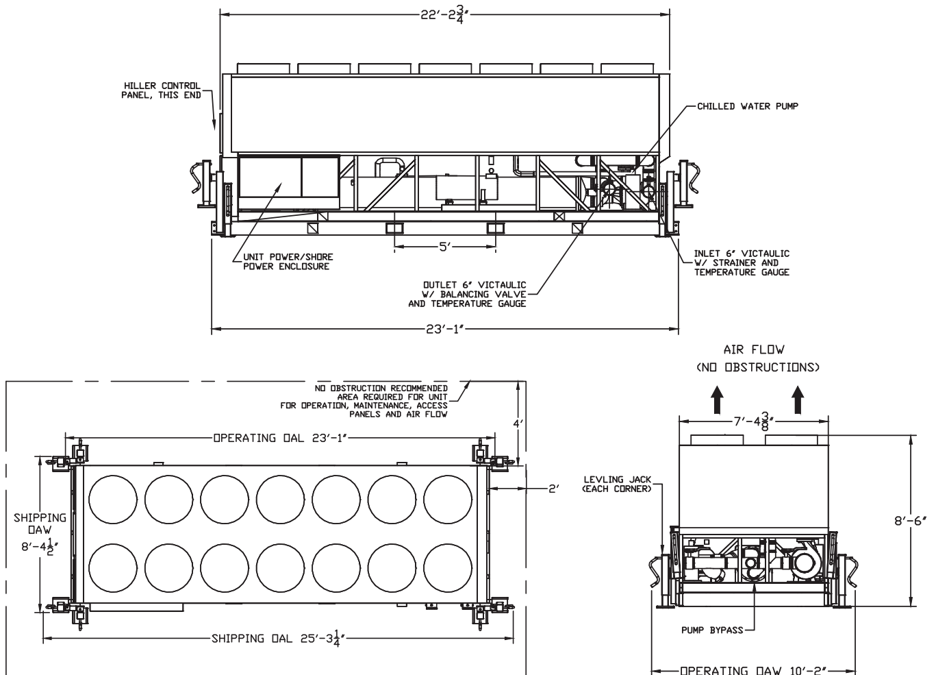
Figure 79. Unit drawings
