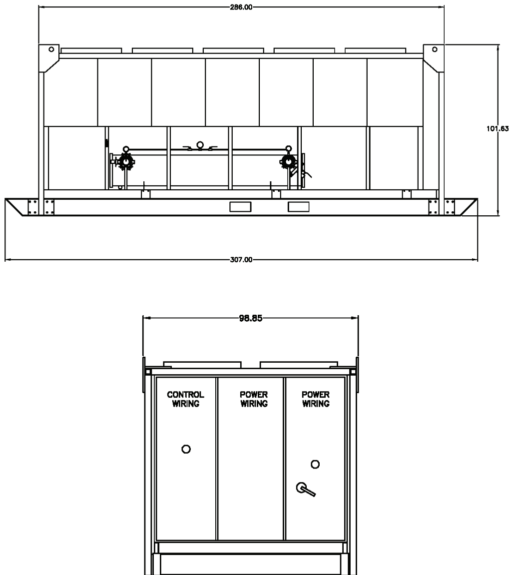
Figure 62. Unit drawings
