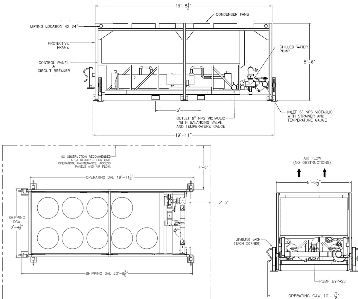
Figure 59. Unit drawings
