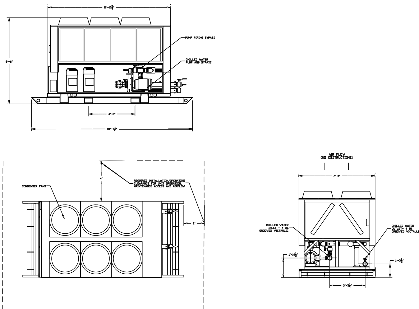
Figure 29. Unit drawings
