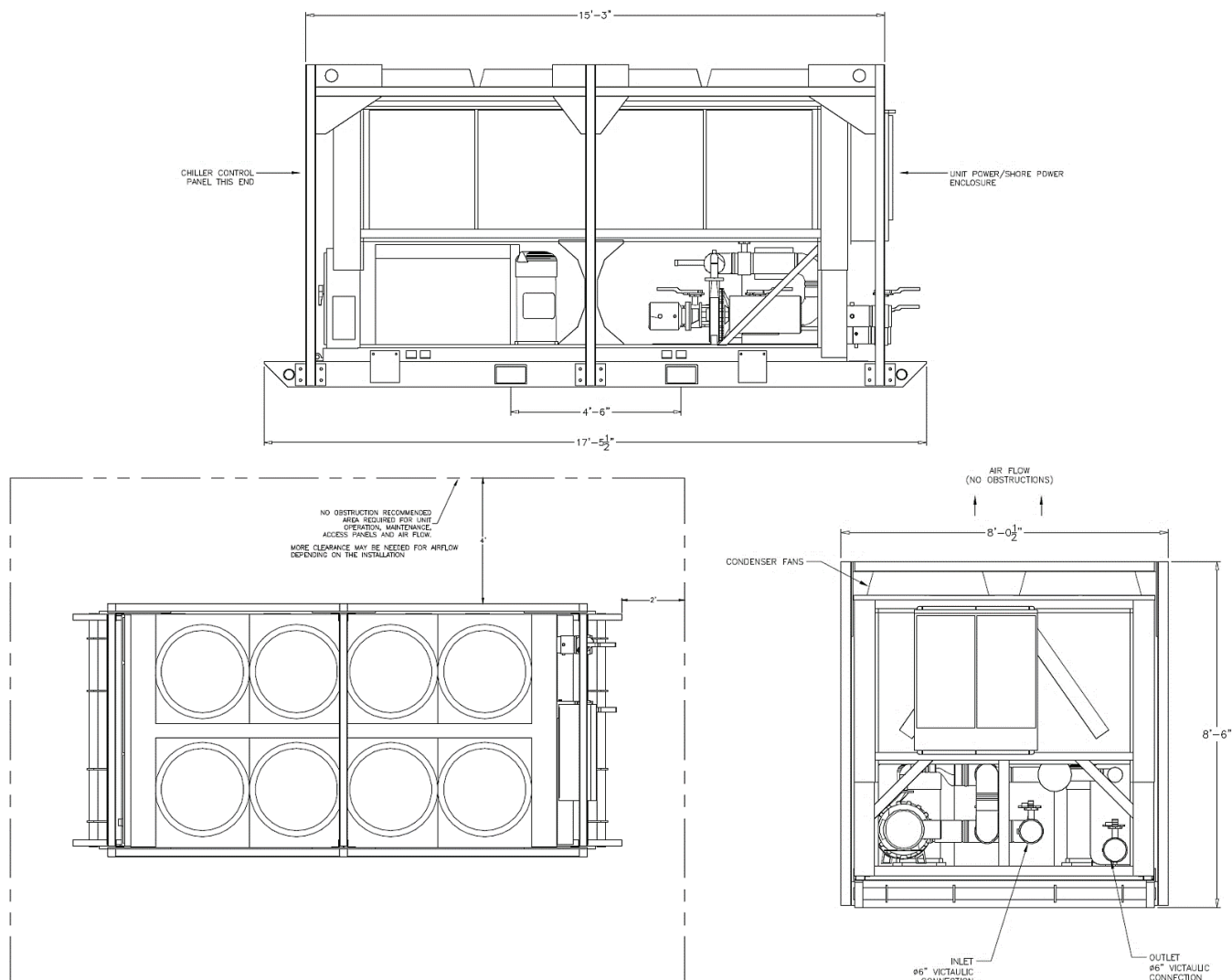
Figure 39. Unit drawings
