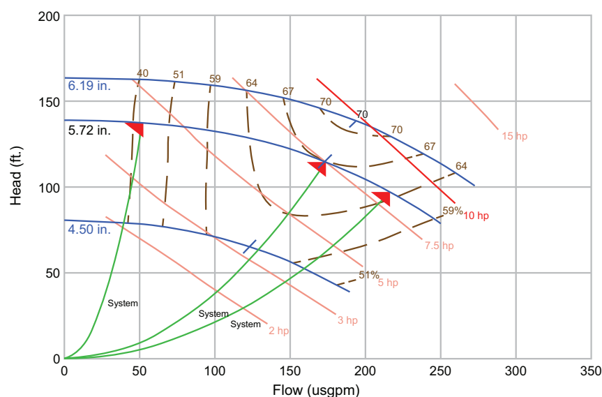
Figure 14. CSCA0040F0 pump curve
