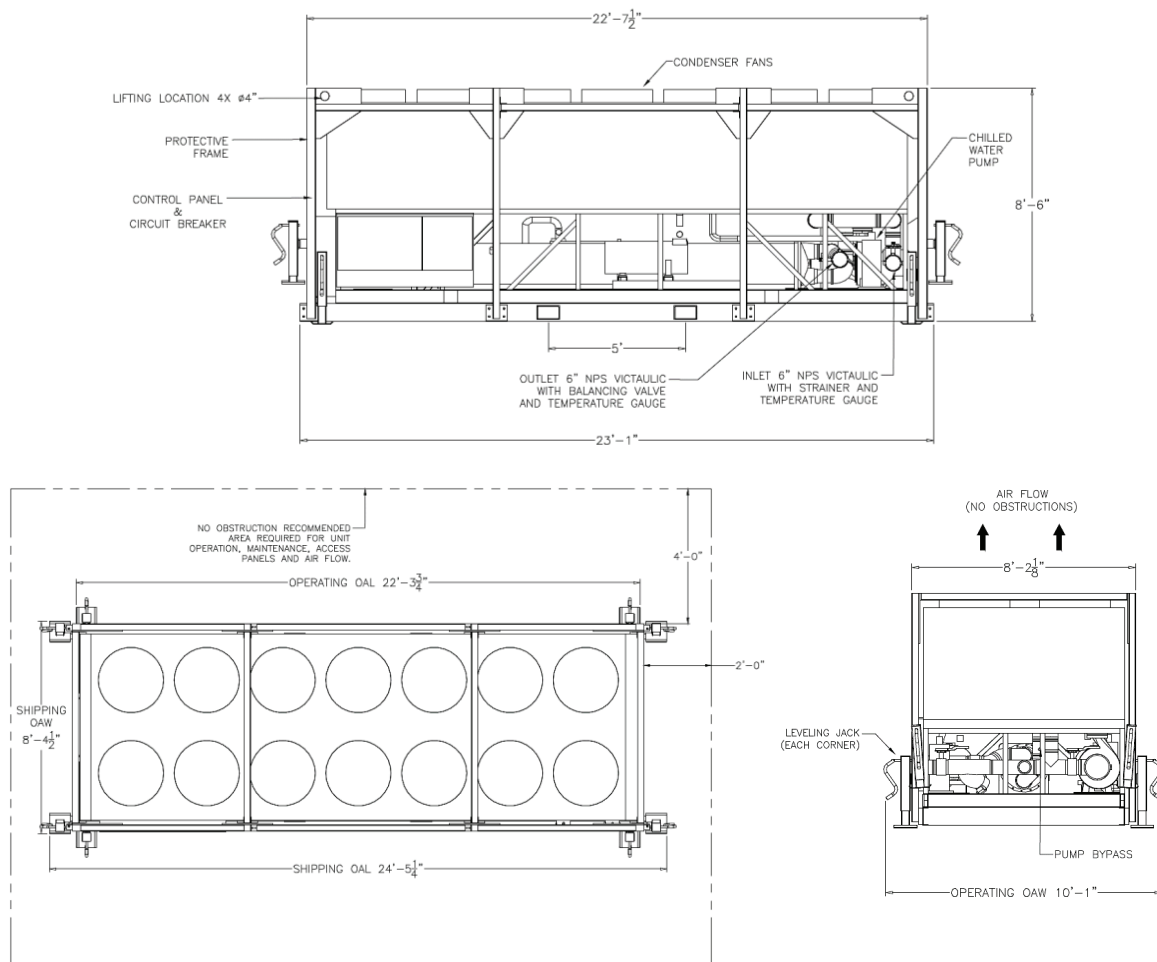
Figure 77. Unit drawings
