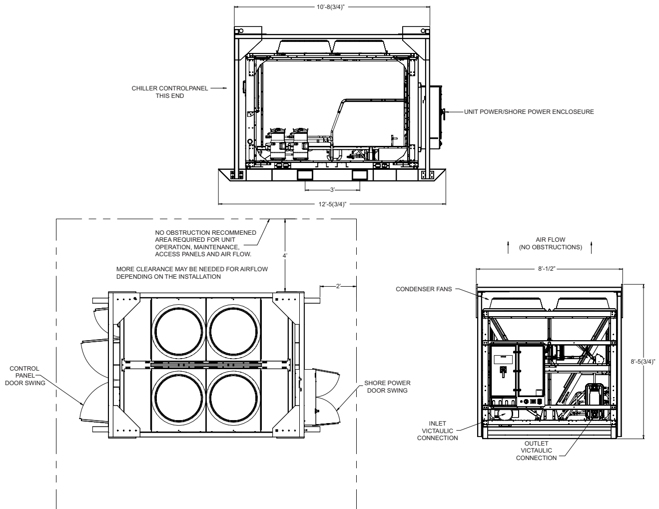
Figure 15. Unit drawings
