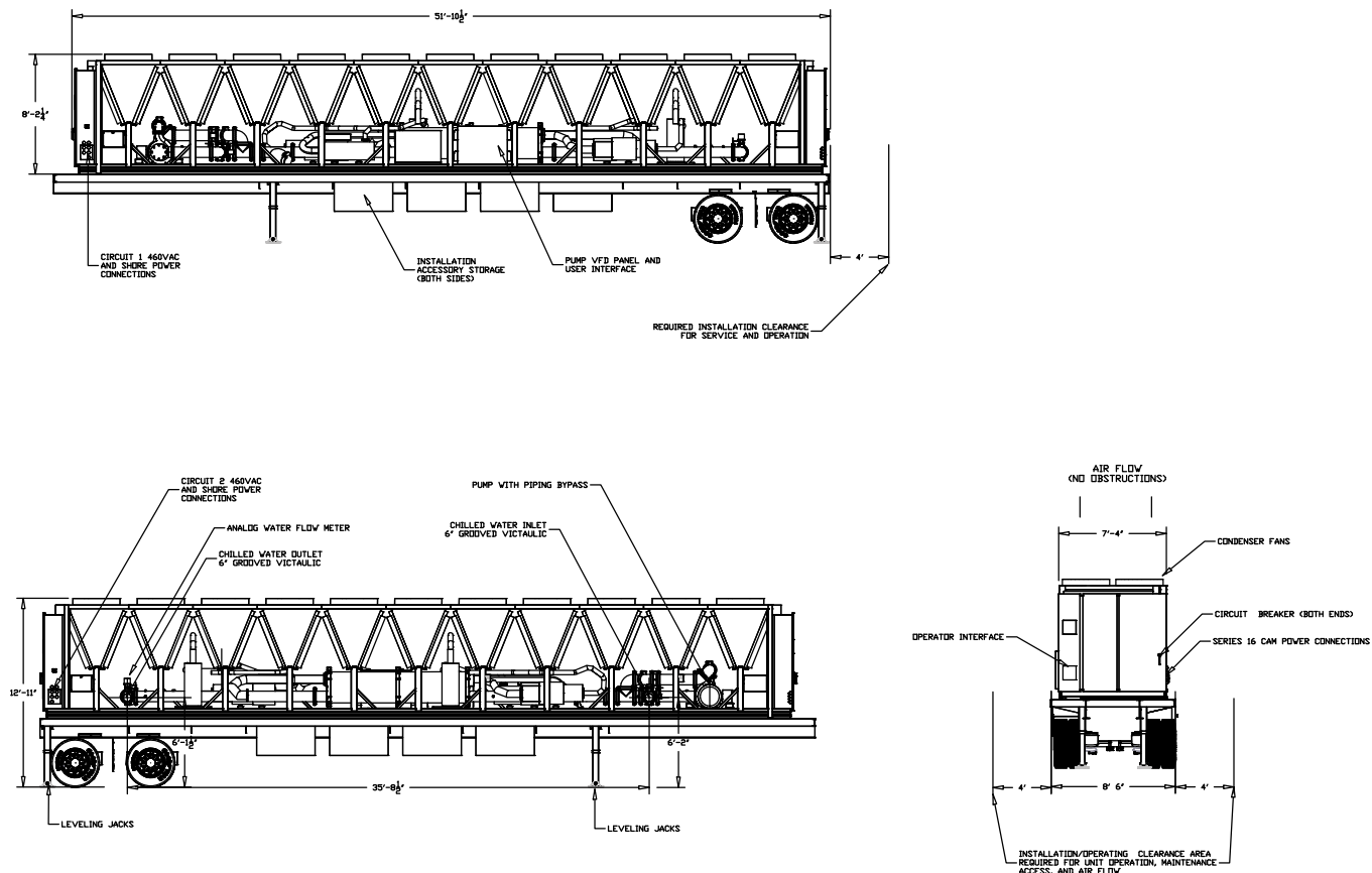
Figure 114. Unit drawings
