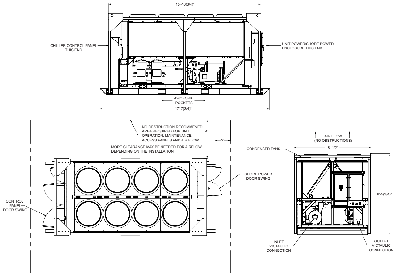
Figure 37. Unit drawings
