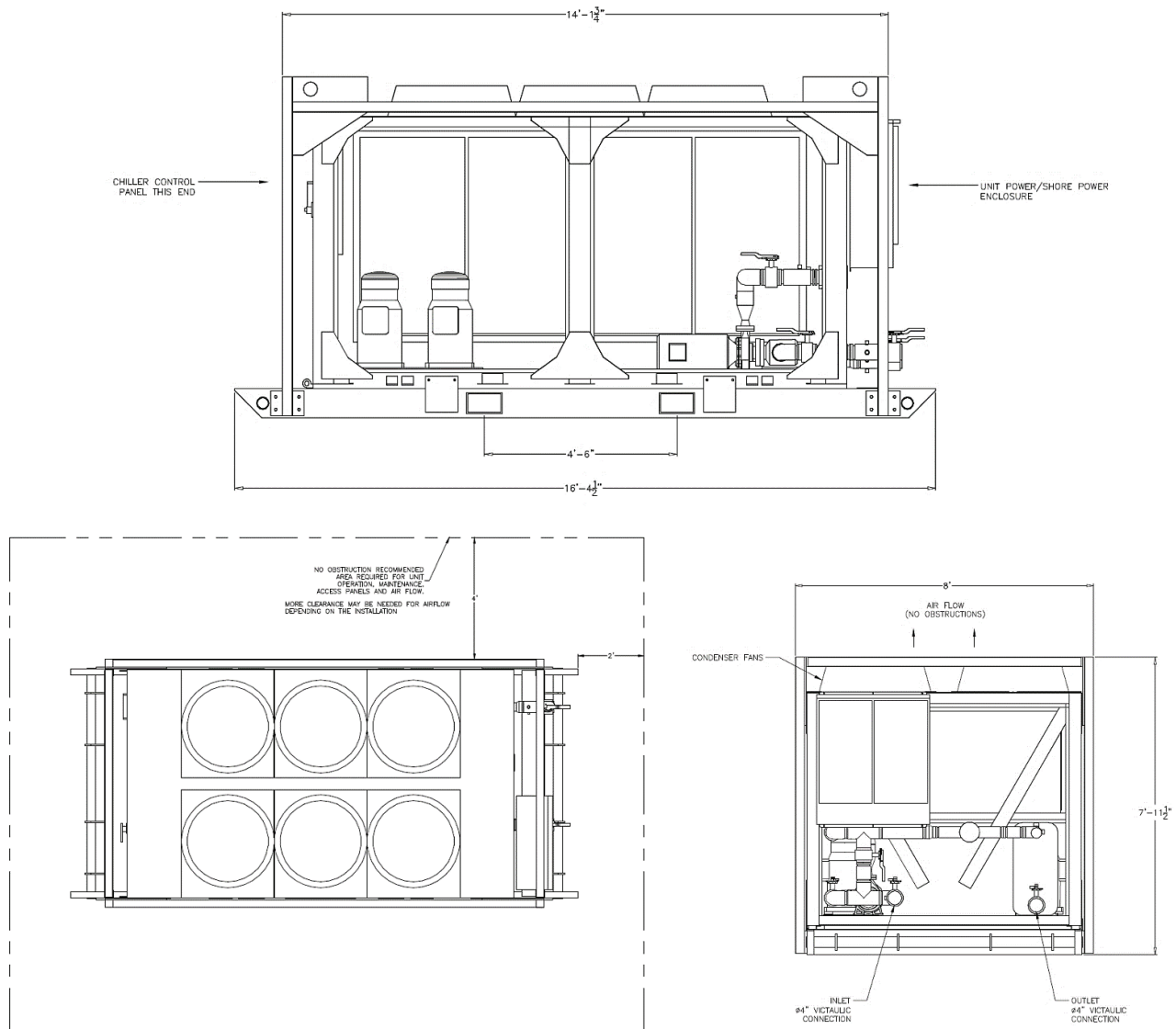
Figure 21. Unit drawings
