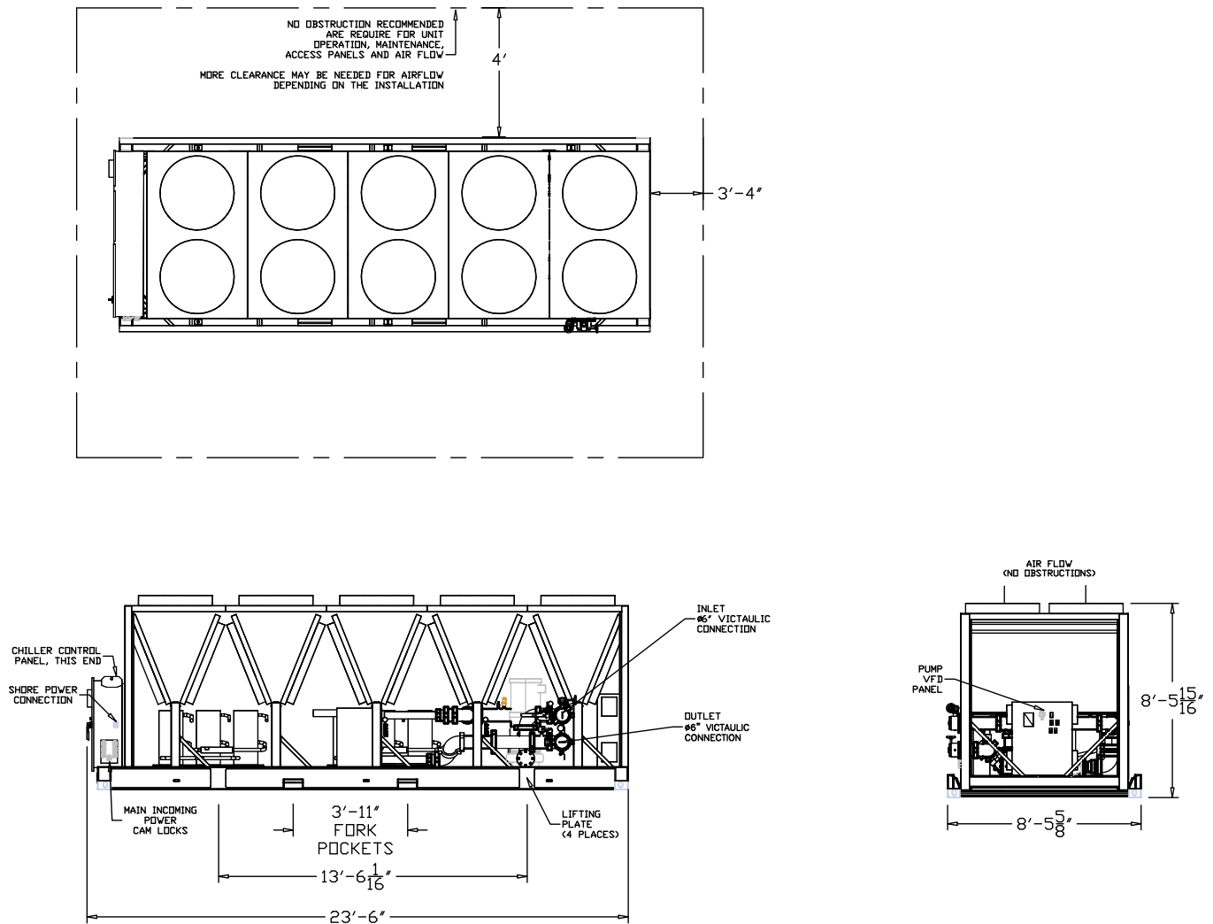
Figure 49. Unit drawings
