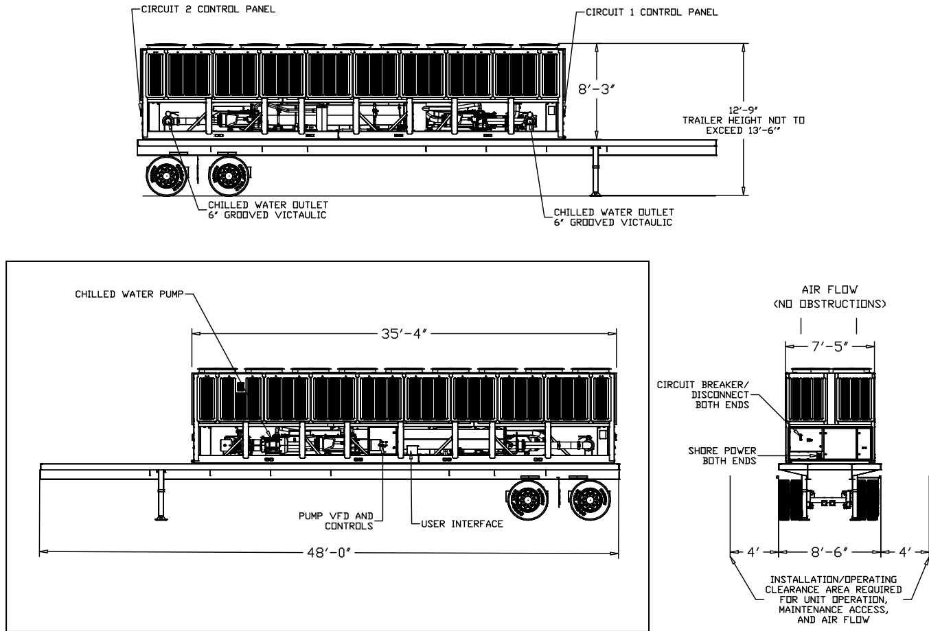
Figure 90. Unit drawings
