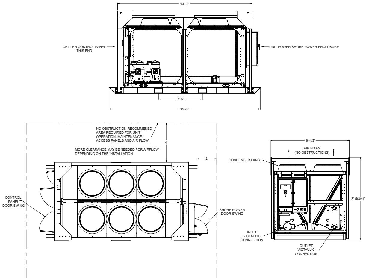
Figure 19. Unit drawings
