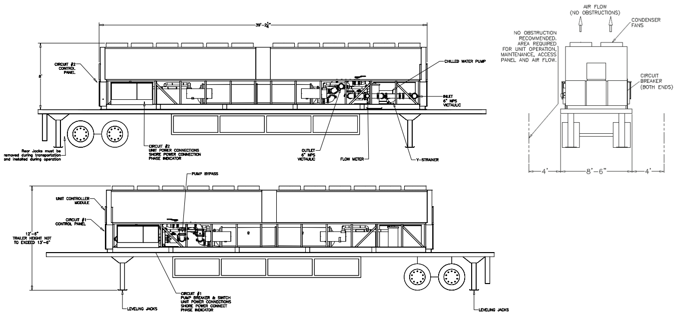
Figure 95. Unit drawings
