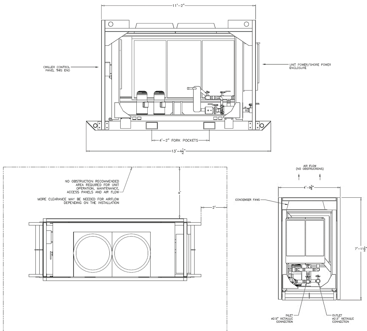
Figure 13. Unit drawings
