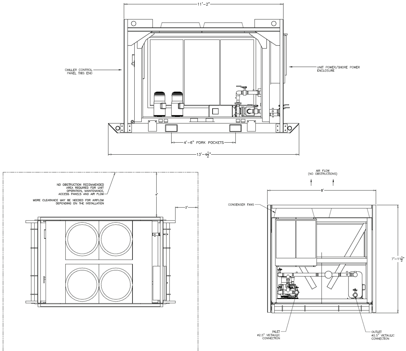
Figure 17. Unit drawings
