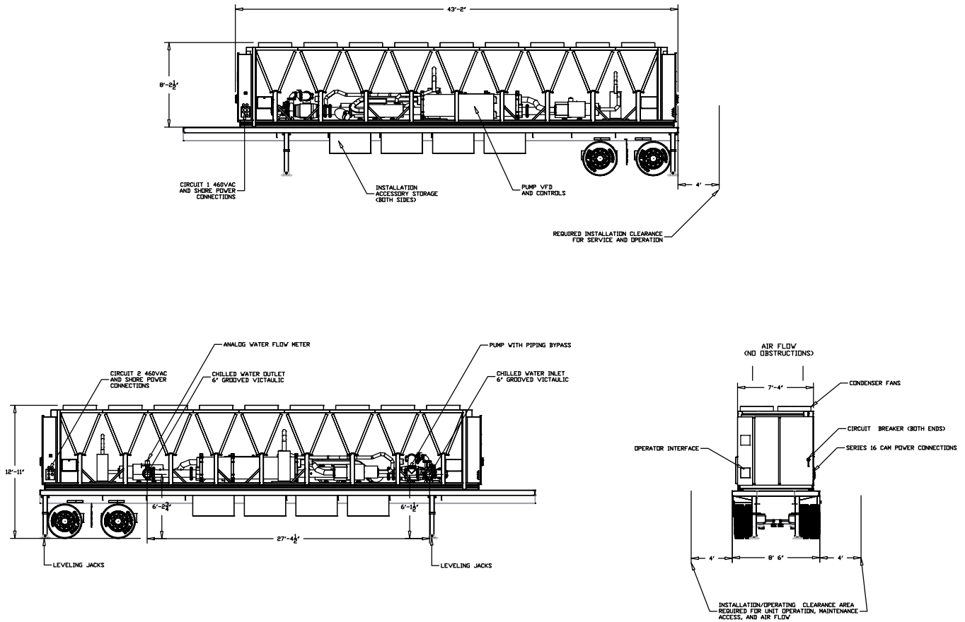
Figure 101. Unit drawings
