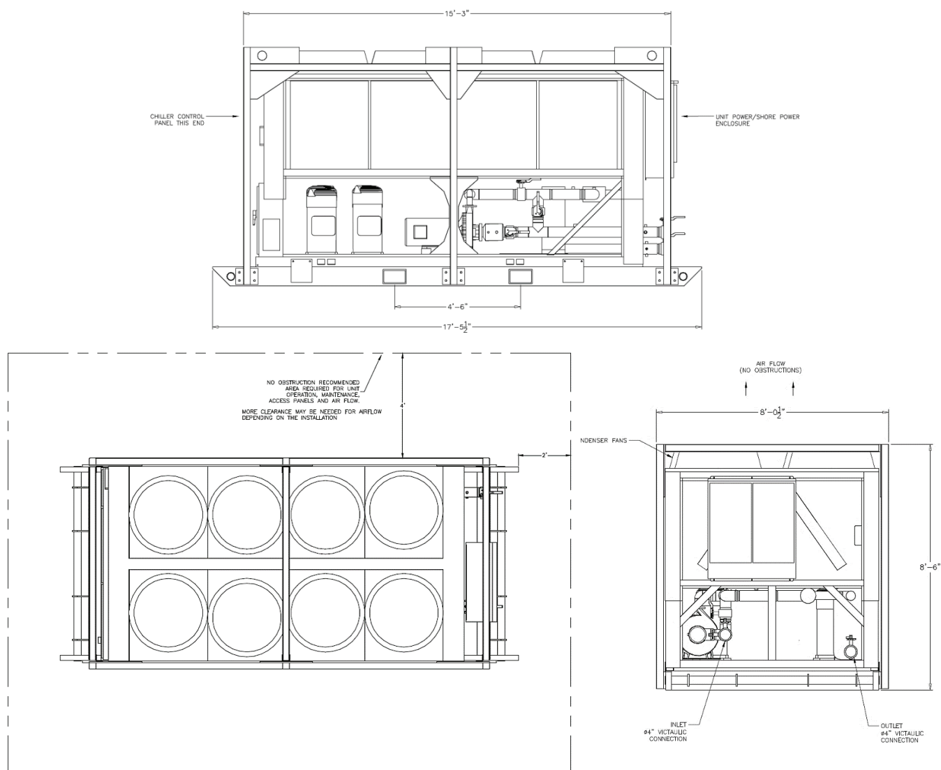
Figure 33. Unit drawings
