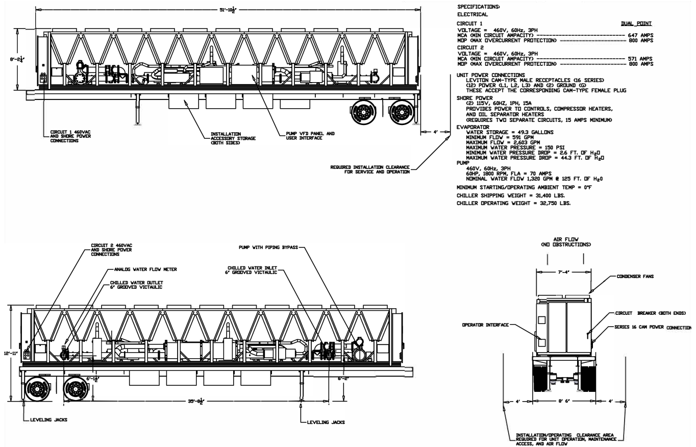
Figure 111. Unit drawings
