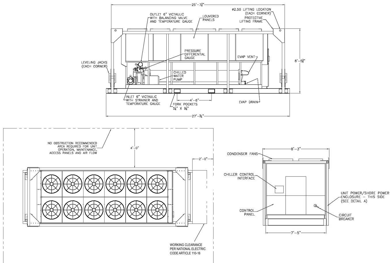
Figure 75. Unit drawings
