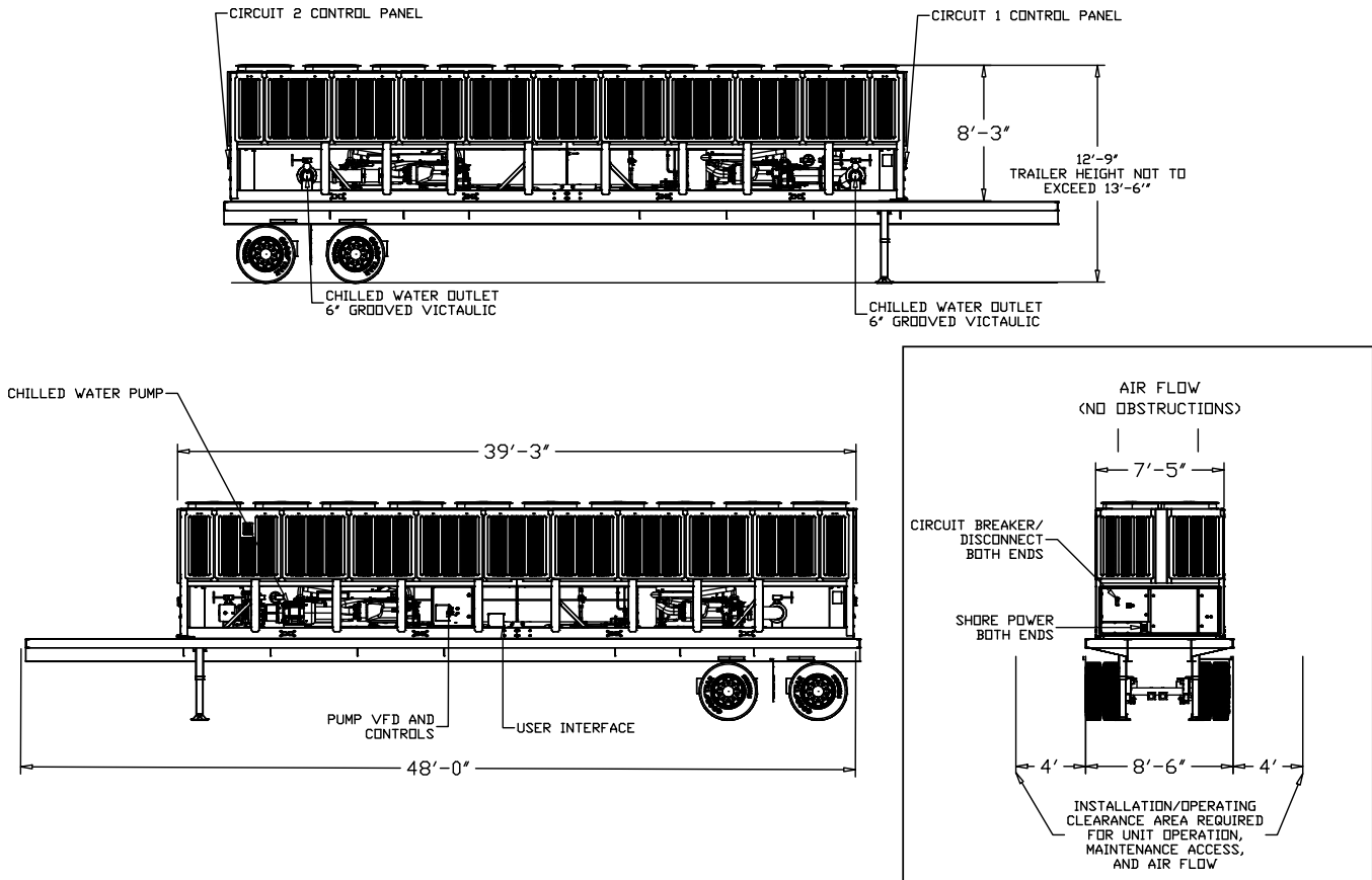
Figure 98. Unit drawings
