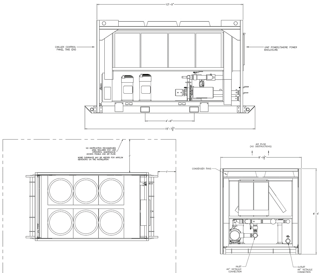
Figure 27. Unit drawings
