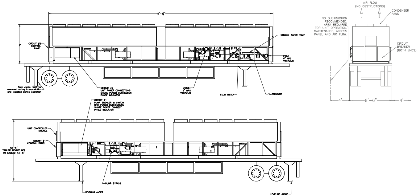
Figure 105. Unit drawings
