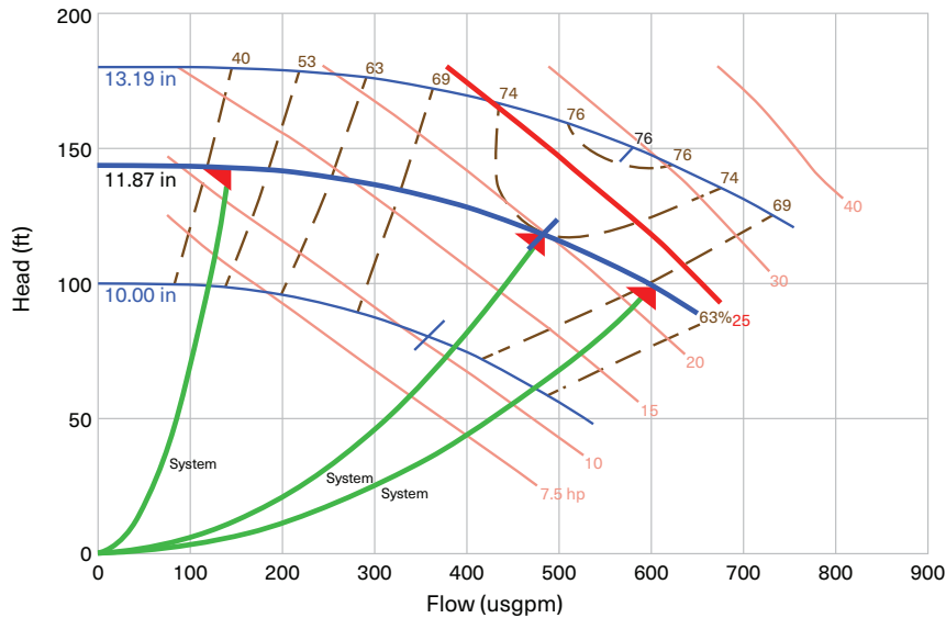
Figure 60. CSCA0155F3 pump curve
