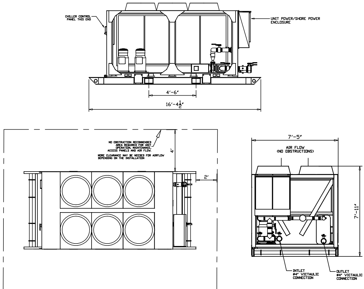
Figure 23. Unit drawings
