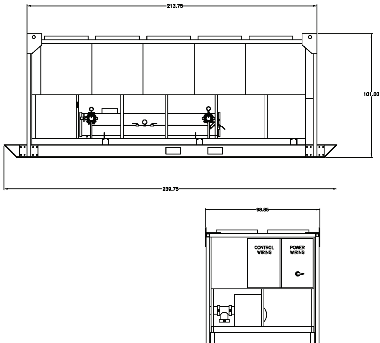
Figure 51. Unit drawings
