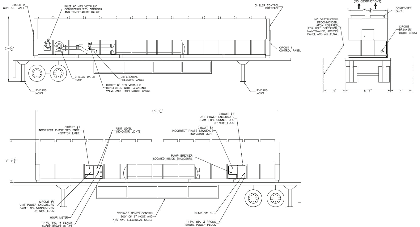
Figure 103. Unit drawings
