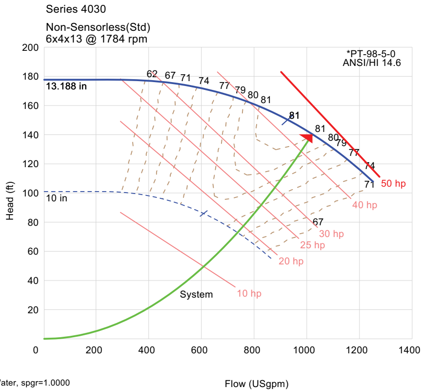
Figure 96. RSCA0440F0 - single speed pump curve
