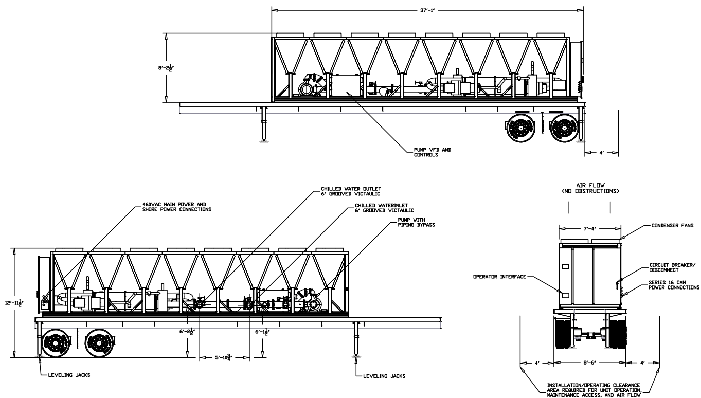
Figure 87. Unit drawings
