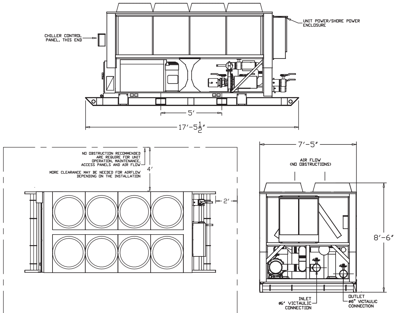
Figure 41. Unit drawings
