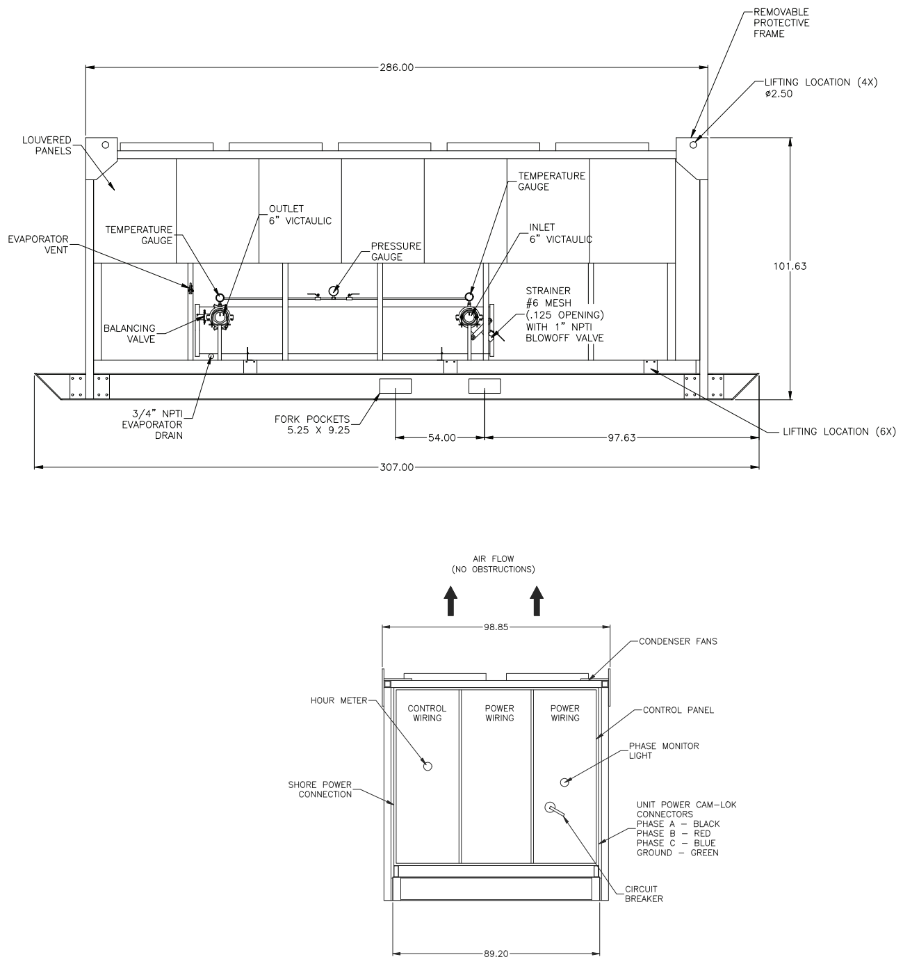
Figure 67. Unit drawings
