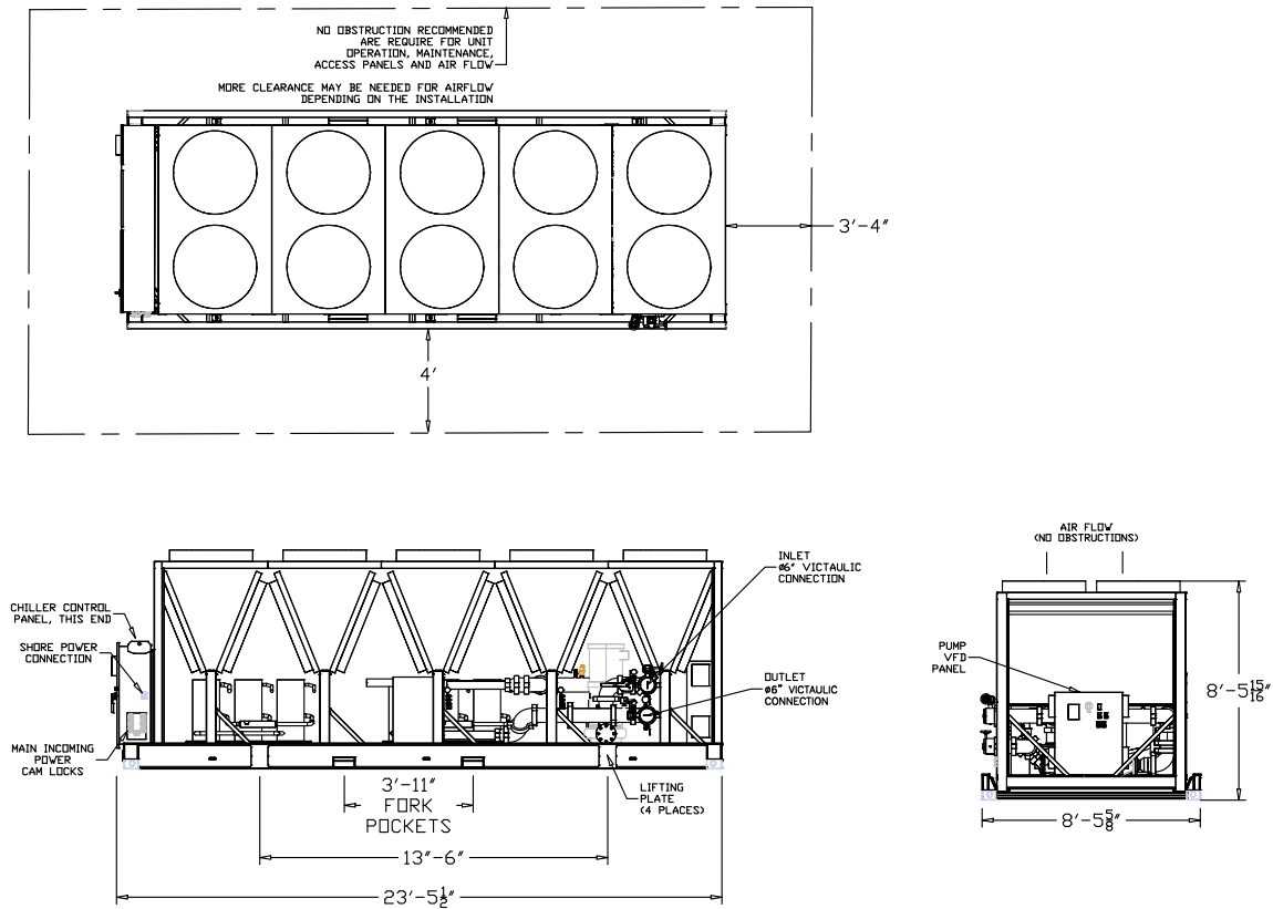
Figure 46. Unit drawings
